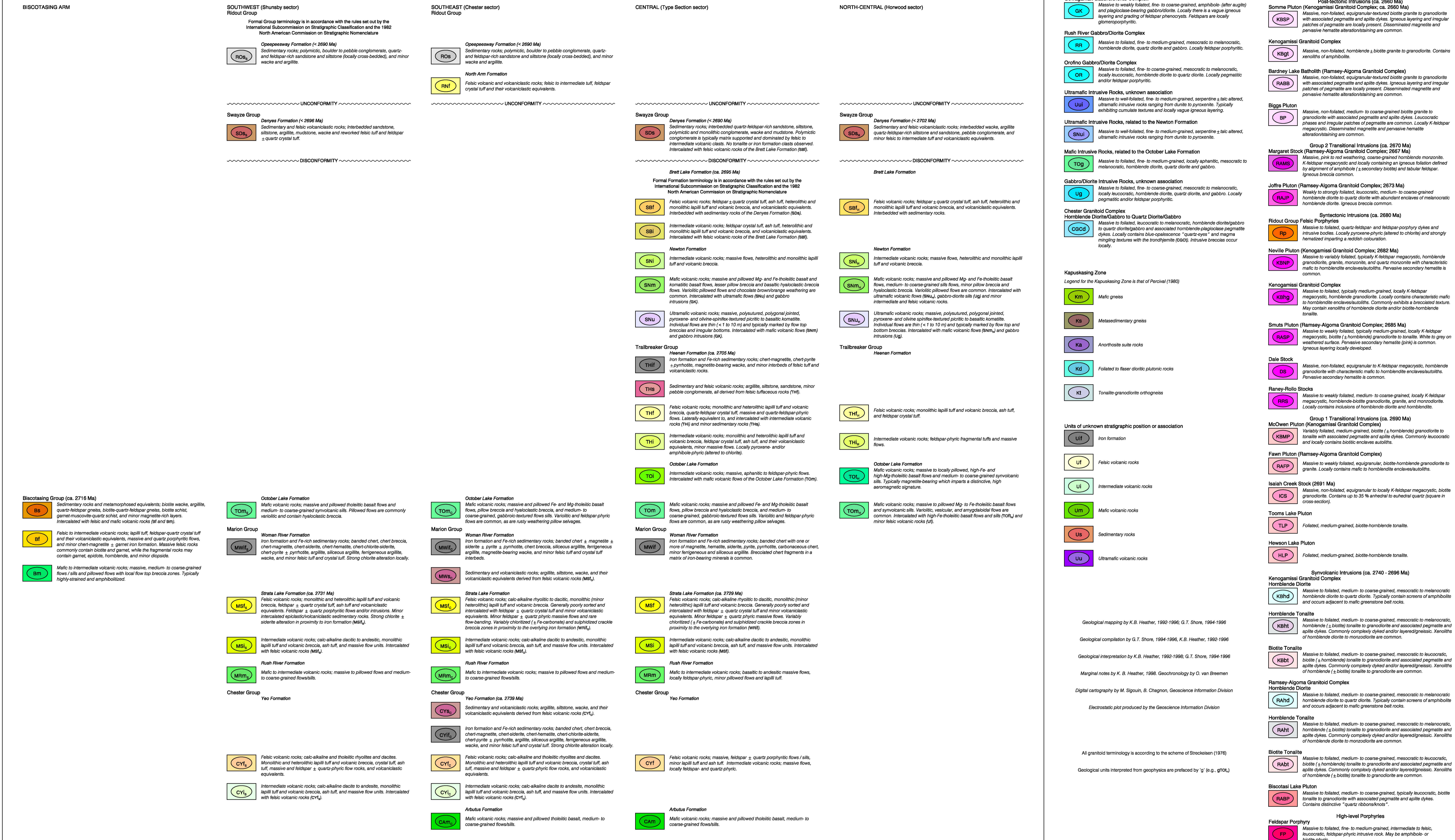
Geological mapping by K.B. Heather, 1992-1996; G.T. Shore, 1994-1996. Geological interpretation by K.B. Heather, 1992-1996; G.T. Shore, 1994-1996. Marginal notes by K.B. Heather, 1996. Geochronology by O. van Breemen. Digital cartography by M. Spagnol, B. Chagnon, Geoscience Information Division. Electrostatic plot produced by the Geoscience Information Division. All granitoid terminology is according to the scheme of Breckelien (1976). Geological units interpreted from geophysics are prefixed by 'g' (e.g., gTOL).
