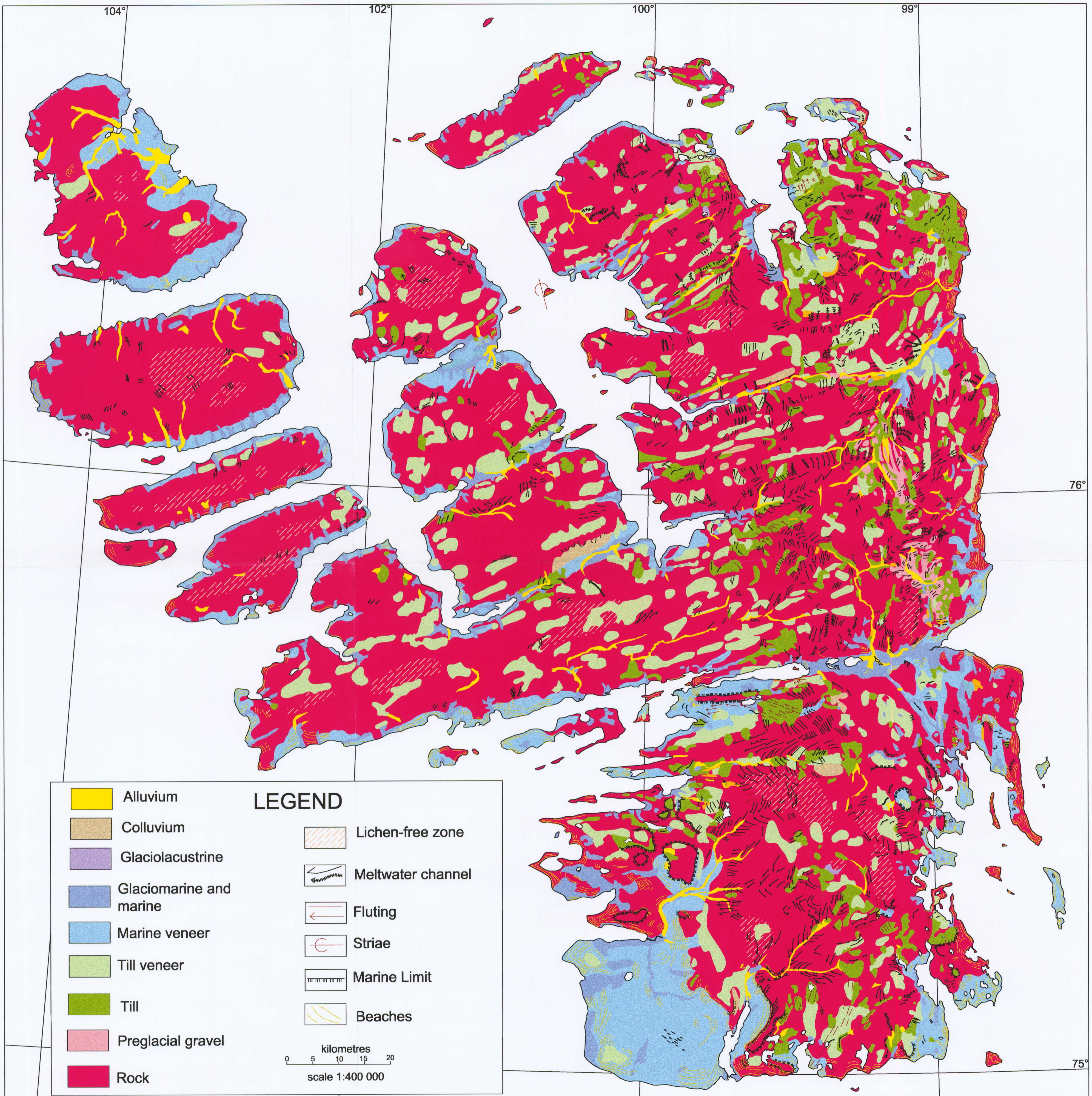
Figure 3. General Surficial Geology
