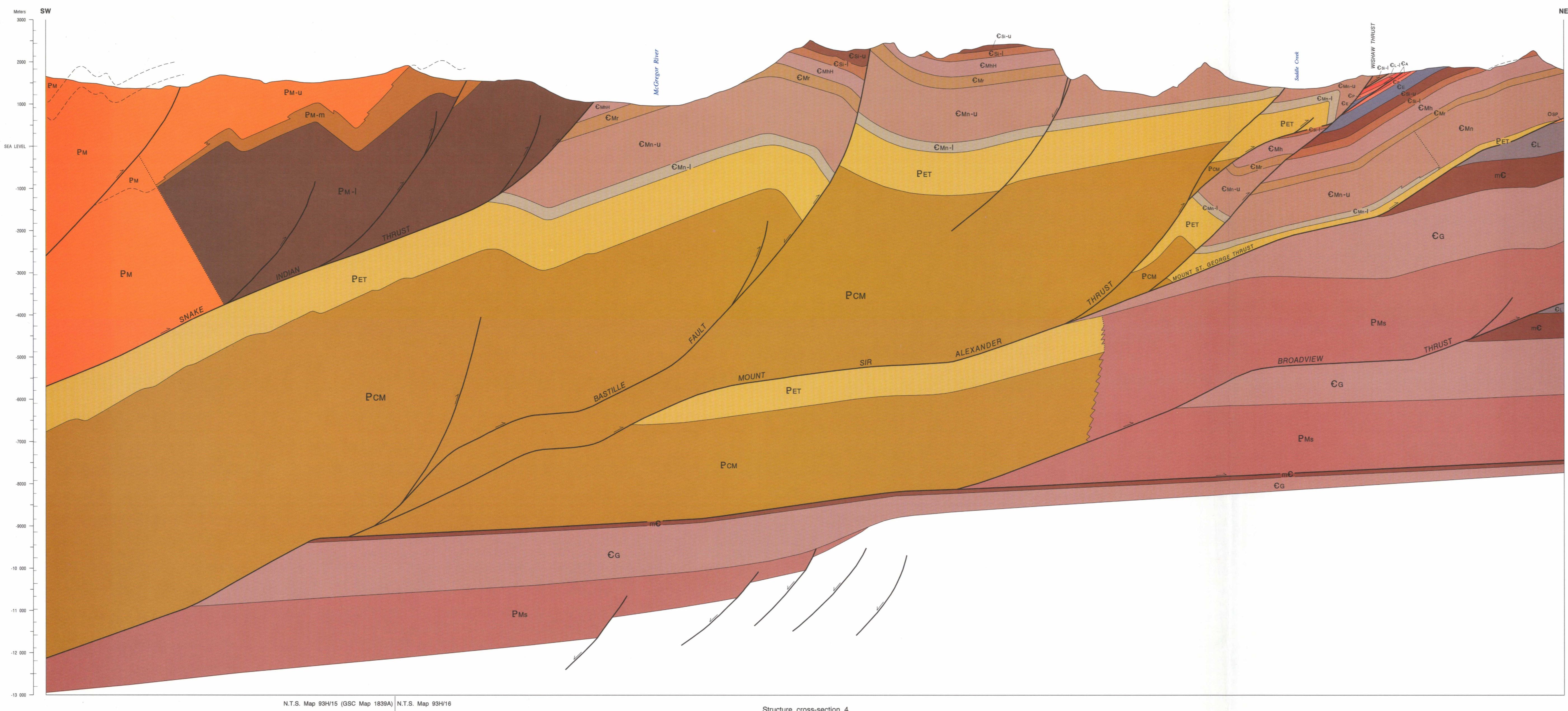
Structure cross-section 4
