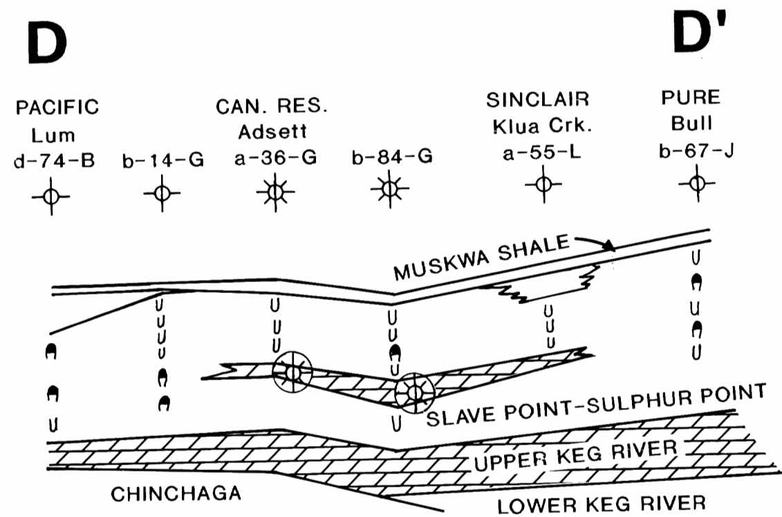
STRUCTURAL CROSS SECTION ADSETT AREA
