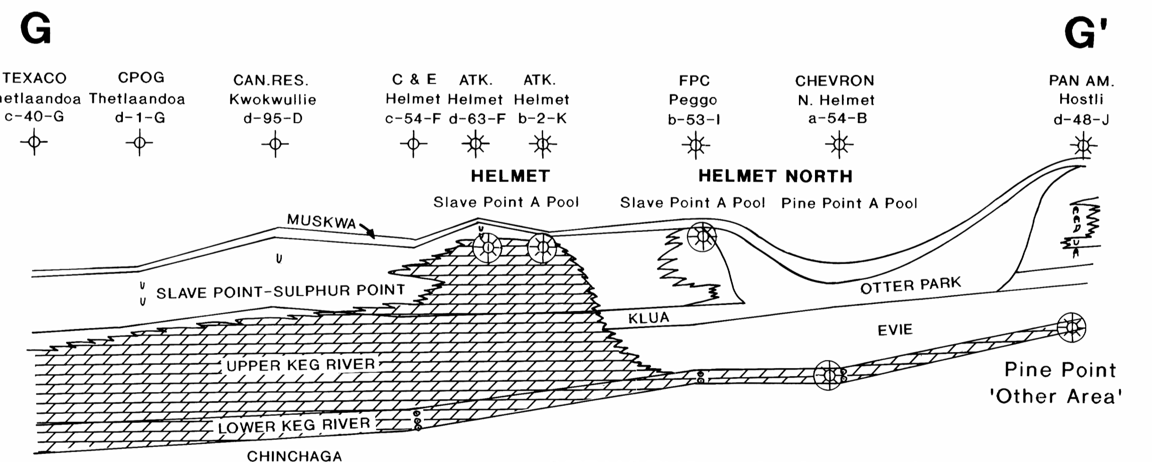
STRUCTURAL CROSS SECTION HELMET AREA
