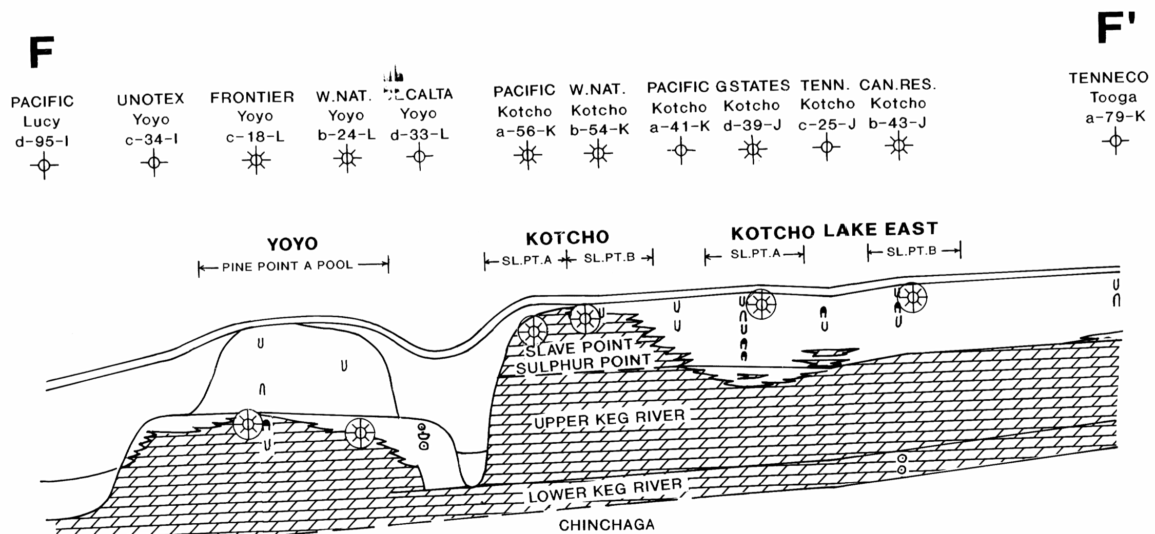
STRUCTURAL CROSS SECTION YOYO-KOTCHO AREA
