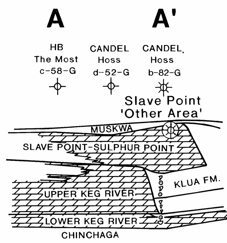
STRUCTURAL CROSS SECTION HOSS AREA
