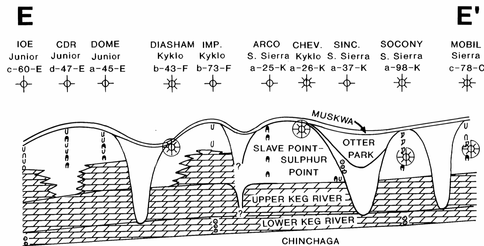
STRUCTURAL CROSS SECTION SIERRA AREA
