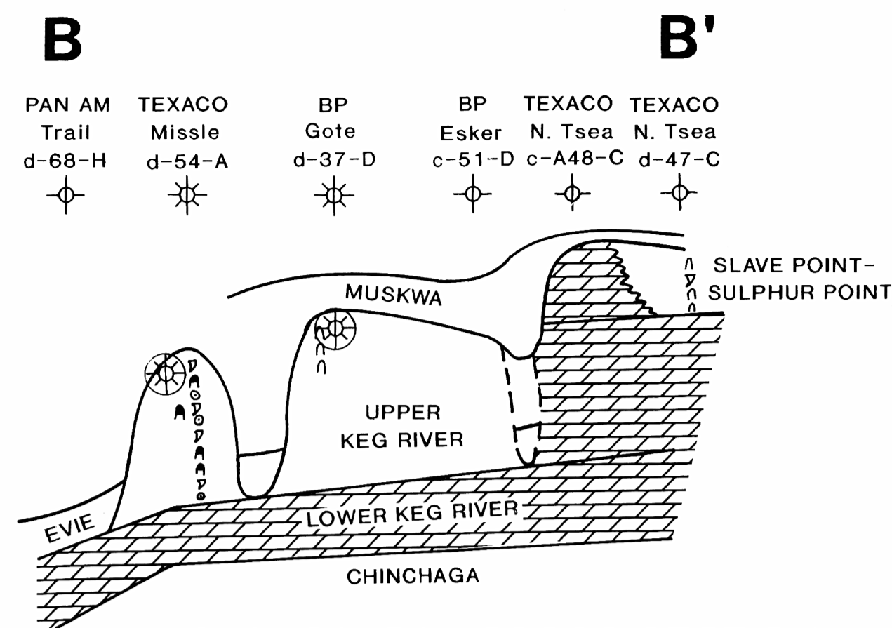
STRUCTURAL CROSS SECTION GOTE AREA
