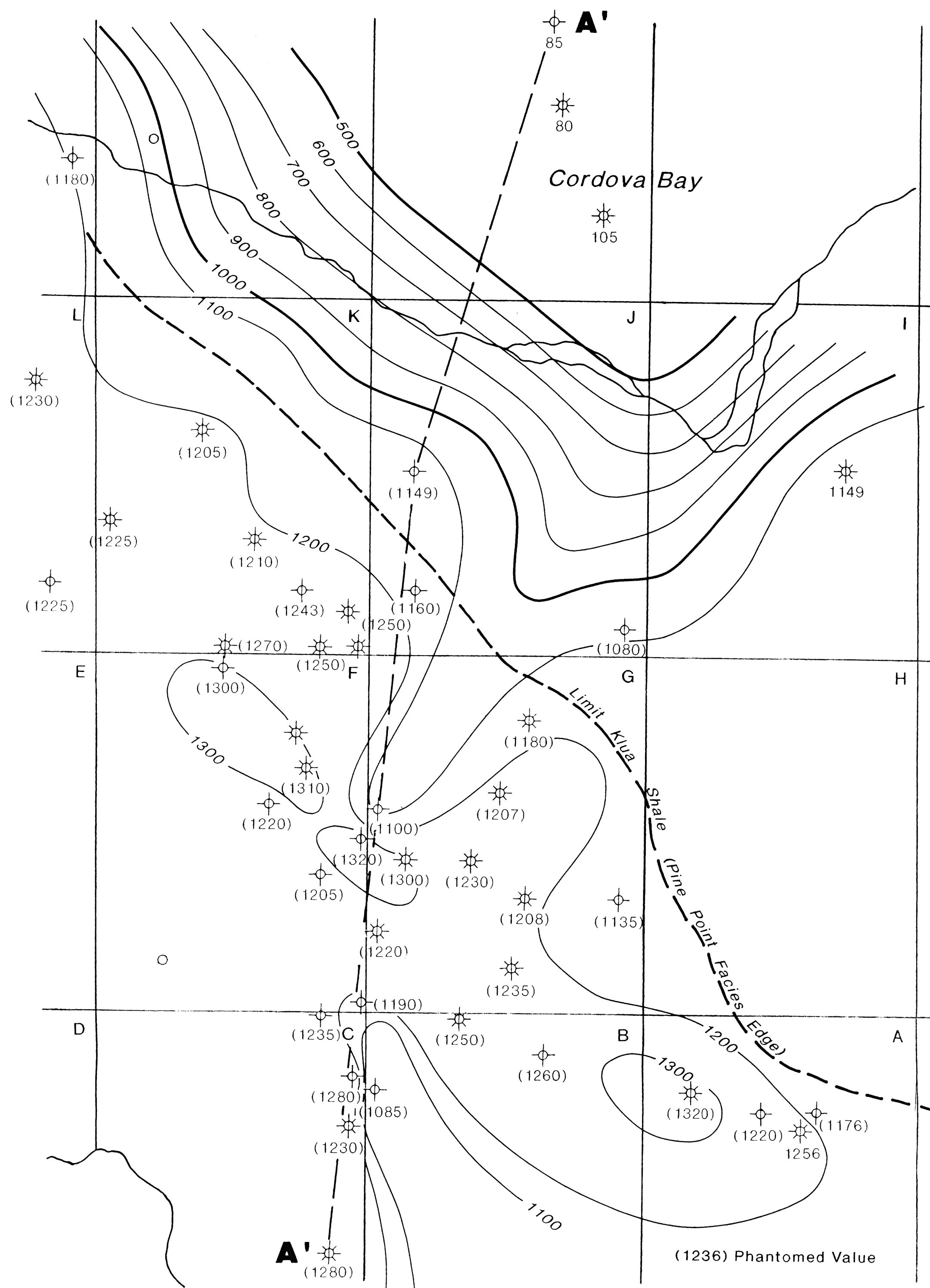
Middle Devonian Carbonate Thickness (Feet) CI - 100 Feet
