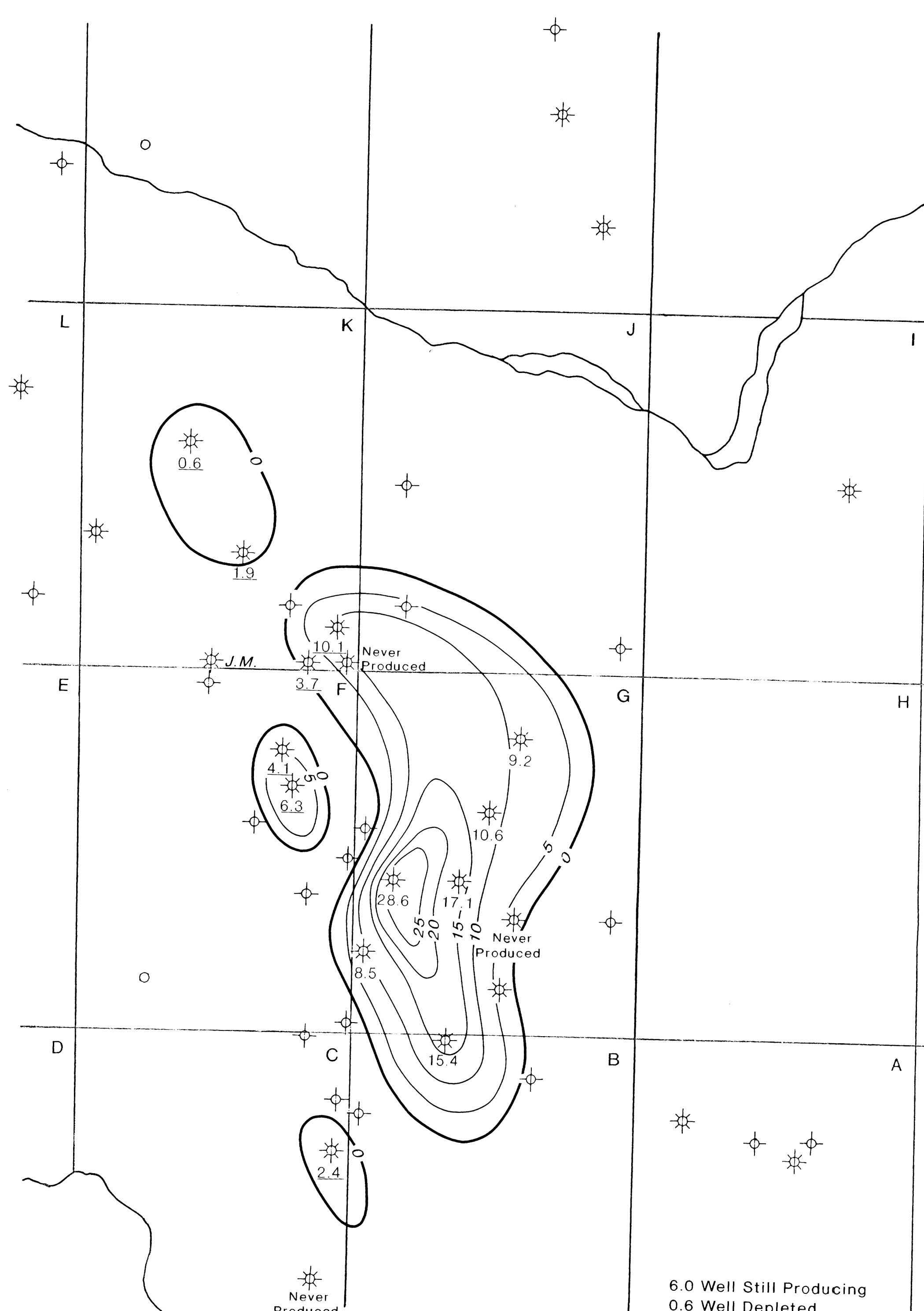
Cumulative Production Bcf CI - 5 Bcf
