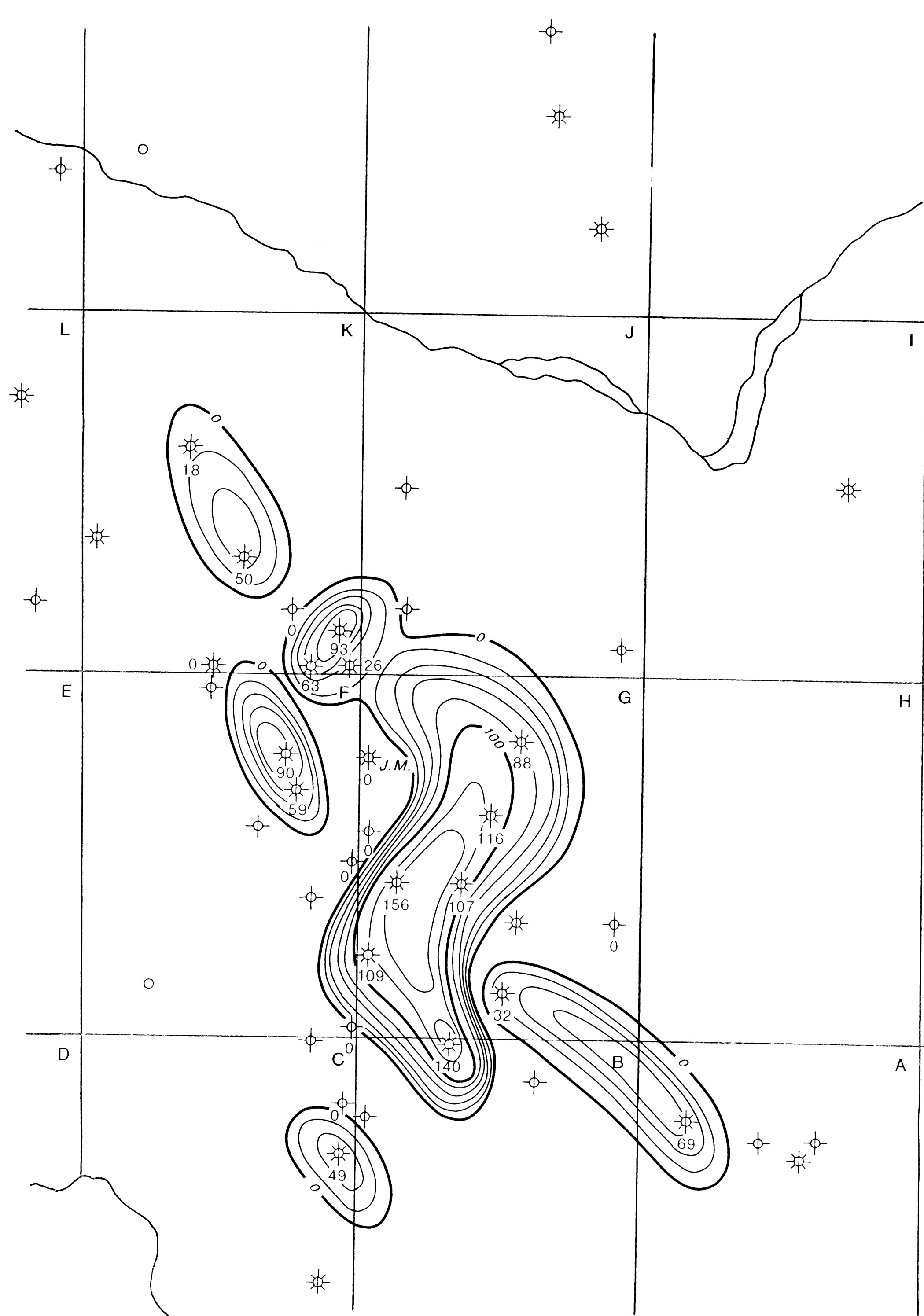
Feet Net Gas Pay CI - 20 Feet
