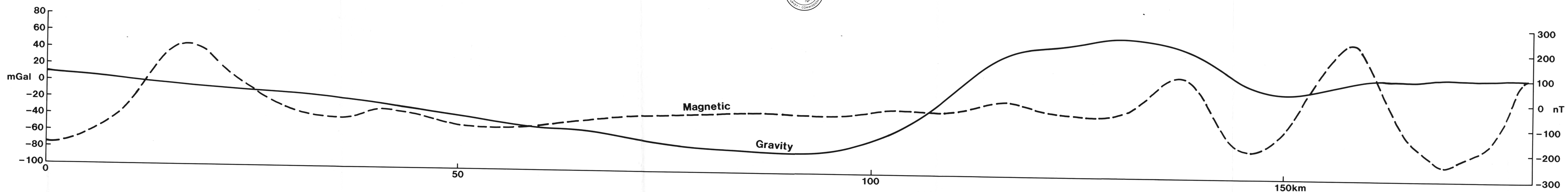
Figure 8. Multi-channel reflection line 5 and corresponding gravity (solid) and magnetic (dashed) profile data.
