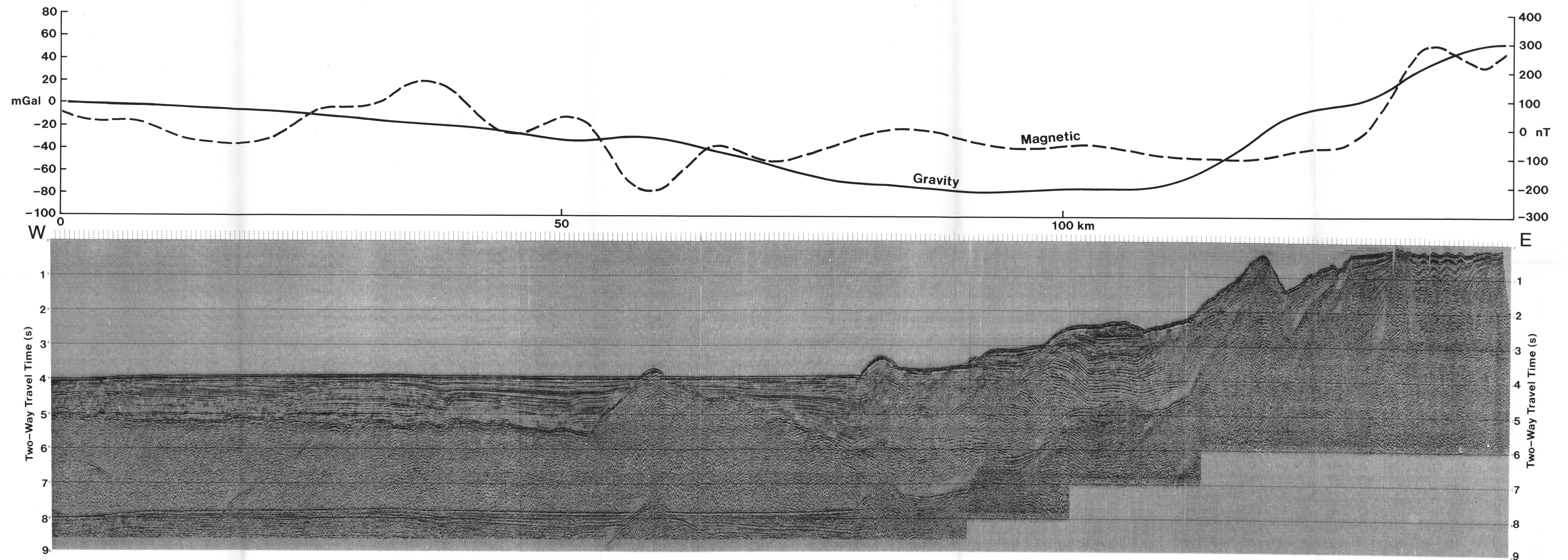
Figure 7. Multi-channel reflection line 1 and corresponding gravity (solid) and magnetic (dashed) profile data.
