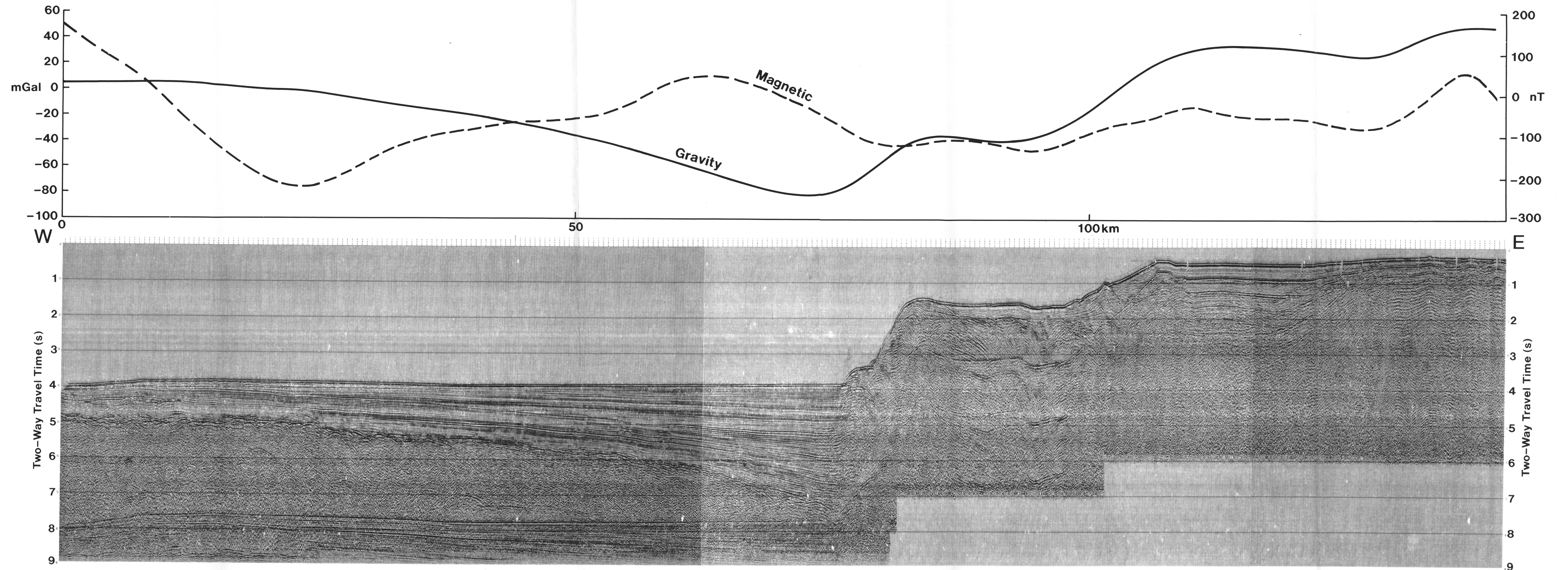
Figure 6. Multi-channel reflection line 2 and corresponding gravity (solid) and magnetic (dashed) profile data. See text for description of acquisition and processing procedures.
