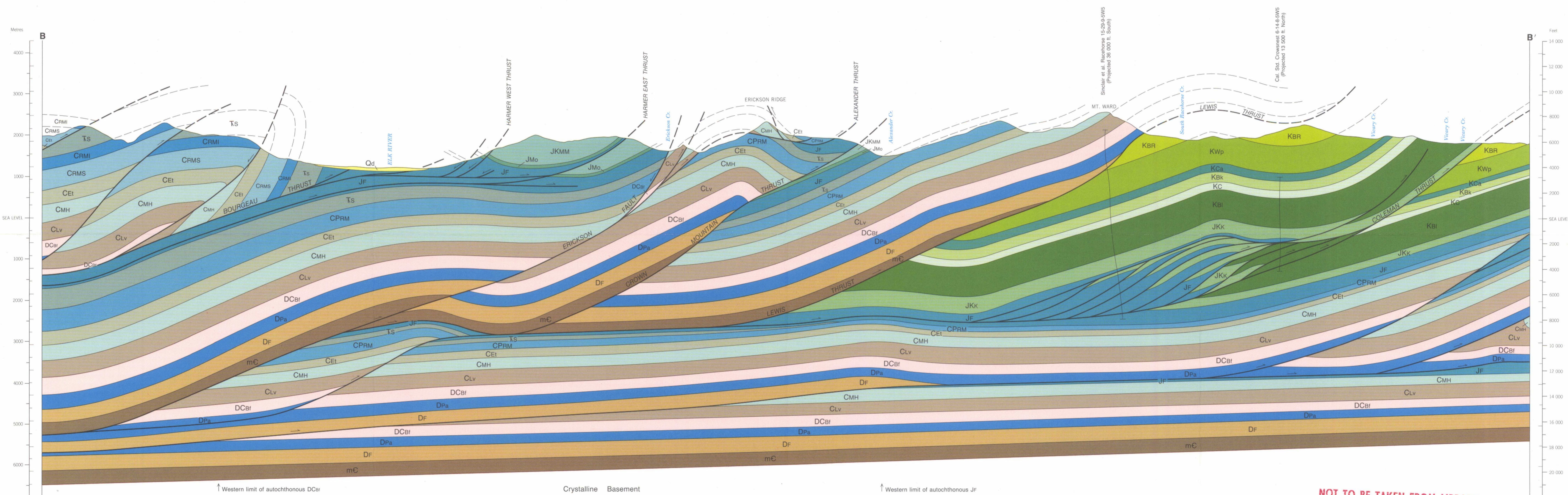
Structure cross-sections A-A' and B-B' to accompany Map 1823A, Tornado Mountain Scale 1:50 000
