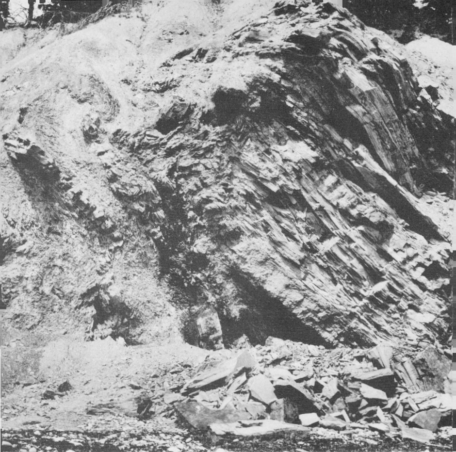
The cliffs at Broad Cove on the east side of the park consist of sandstone, siltstone and shale of Carboniferous age. These have been folded and faulted so that in many places they stand on edge. Wave-erosion undercuts the cliffs rapidly; sliding and slumping are common.
