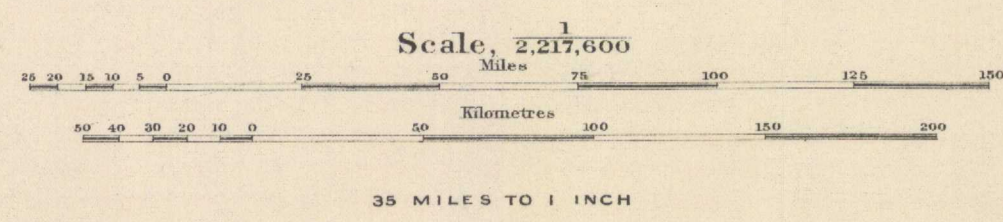
MAP 51A Geological Map of portions of ALBERTA, SASKATCHEWAN AND MANITOBA
