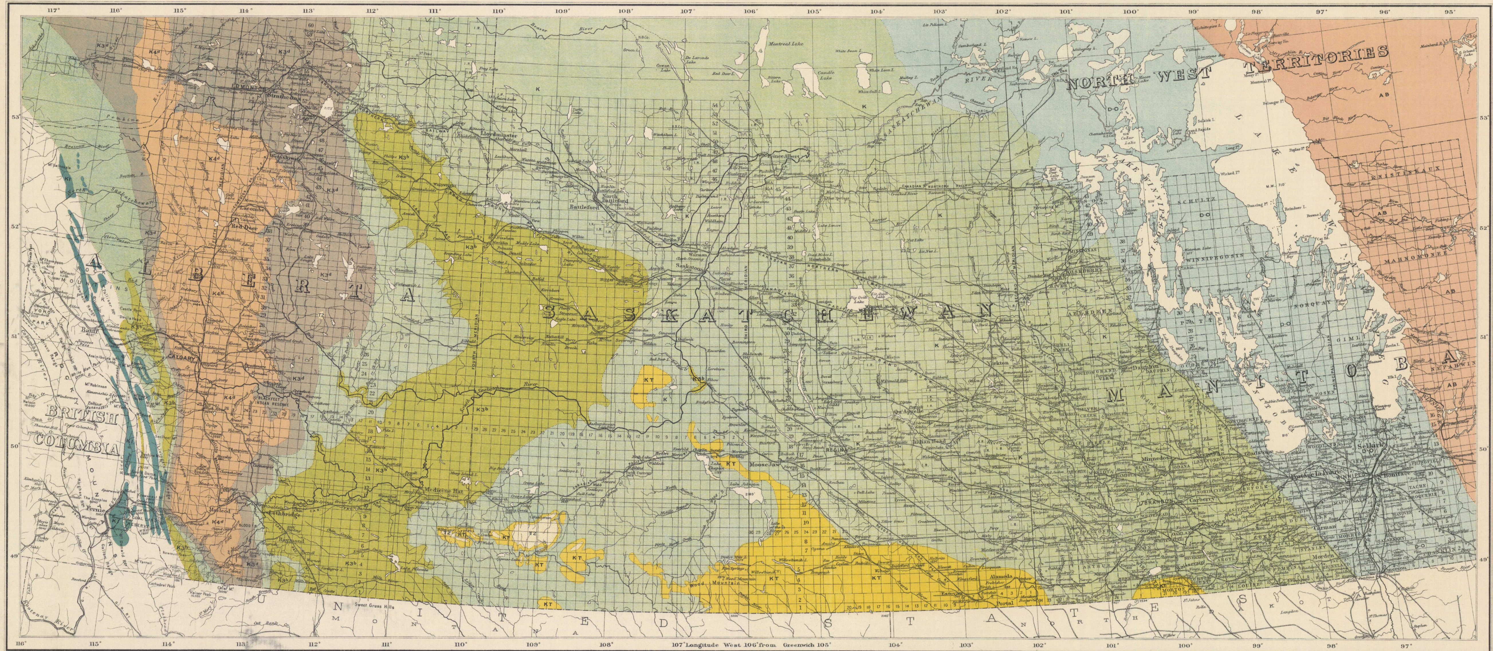
MAP 51A Geological Map of portions of ALBERTA, SASKATCHEWAN AND MANITOBA
