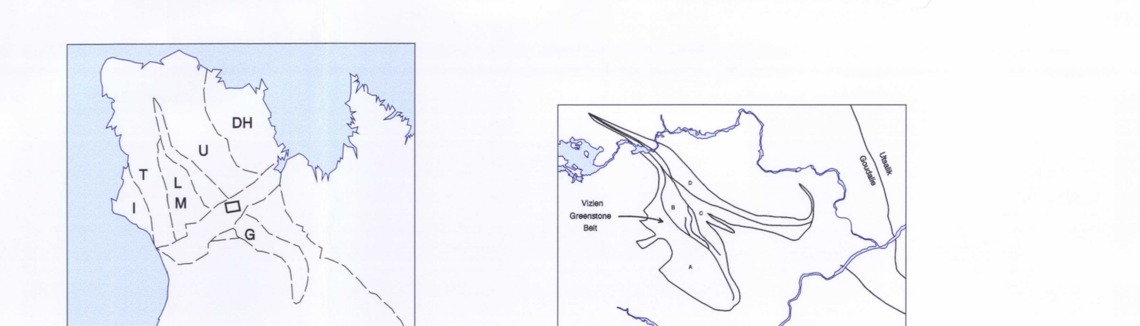
Fig. 1. Location map showing the location of the Vizion Greenstone Belt in the province of Québec. Fig. 2. Detailed map of the Vizion River area.
