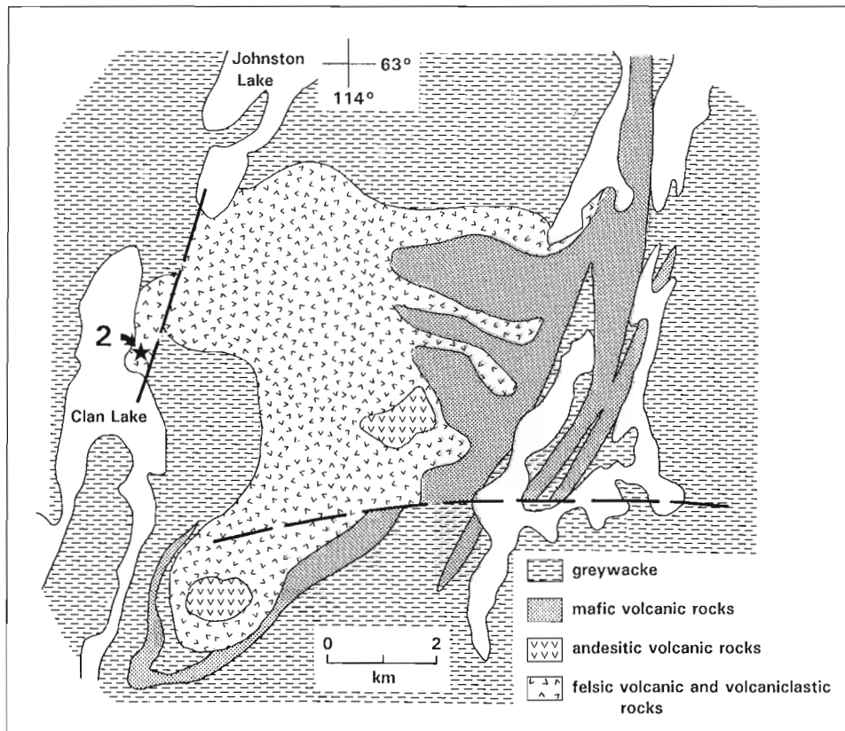
Figure 3. Simplified geological map of the Clan Lake volcanic complex (modified from Hurdle, 1984). Numbered star shows location of Sample 2.
