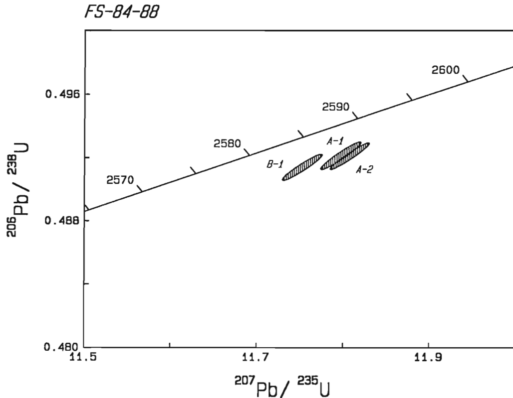
Figure 4. U-Pb concordia diagram for sample FS-84-88. Error ellipses are 2\sigma .
