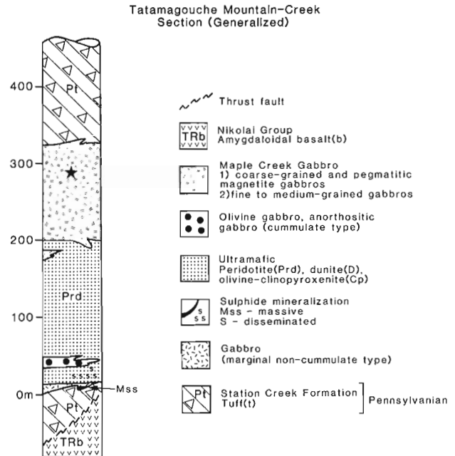
Figure 3. Schematic section through the western part of the Tatamagouche Creek intrusive complex. Star shows the relative position of the dated sample of Maple Creek gabbro.
