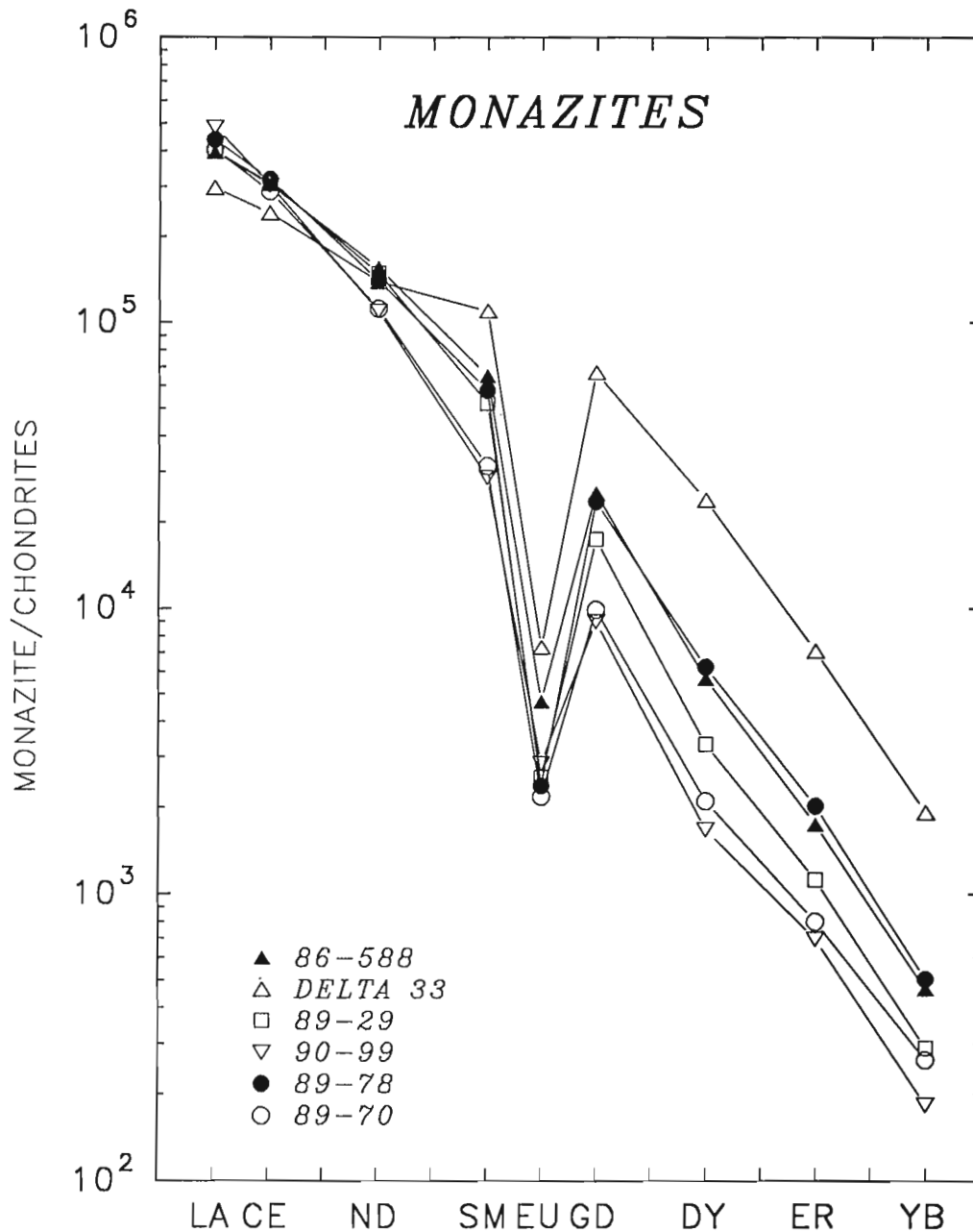
Figure 1. Chondrite-normalized rare earth element diagram of single monazite grains from granodiorite (#29, #99), charnockite (#70), and diatexite (#78) from the Minto block, tonalite from the Ashuanipi complex (#588), and leucogranite from Mount Everest (sample Delta 33).
