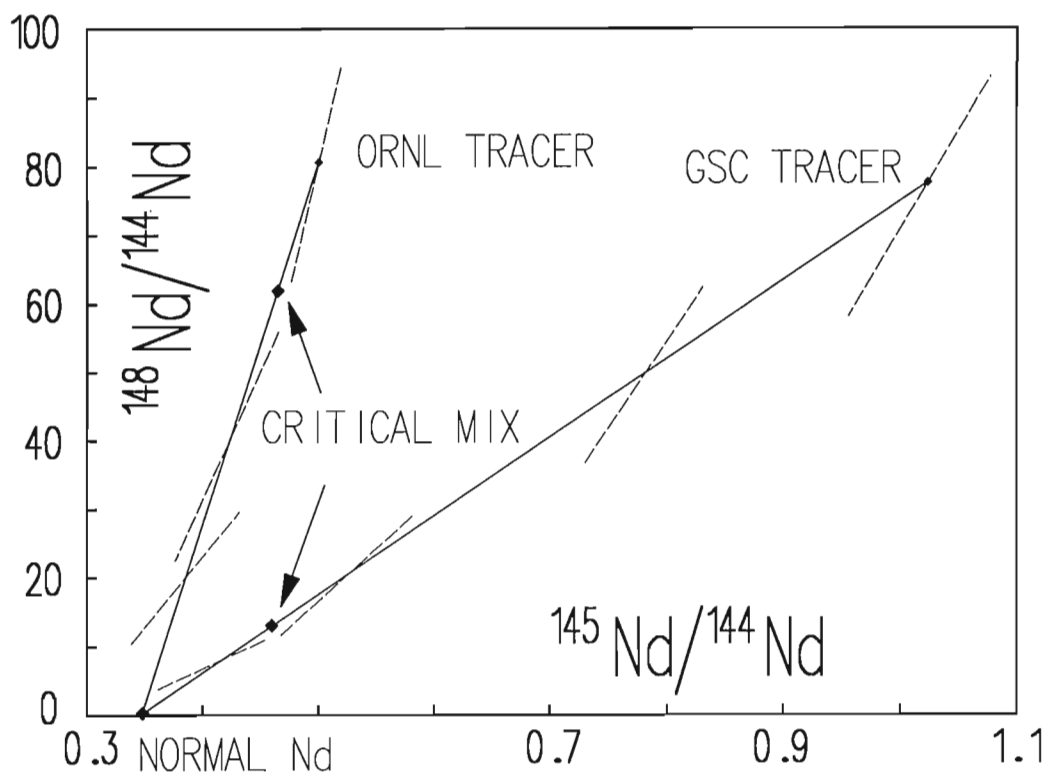
Figure 1. Mixing and isotopic mass fractionation relationships in three isotope ratio plots. Two solid lines define mixing between normal Nd and two ^{148}\text{Nd} tracers differing in ^{145}\text{Nd}/^{144}\text{Nd} . Short dashed lines are isotopic mass fractionation trends for various normal-tracer compositions. At the critical mixtures, mixing and fractionation lines coincide. Critical mixture and normal Nd define the mixing line independent of fractionation. Tracer isotopic composition is determined by intersection of the mixing line and tracer fractionation line. A larger angle of intersection for the GSC tracer permits tracer composition to be determined more accurately than for the ORNL tracer.
