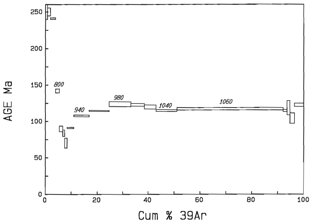
Figure 7. ^{40}\text{Ar}/^{39}\text{Ar} age spectra for hornblende from sample 5, PCA-251-85.
