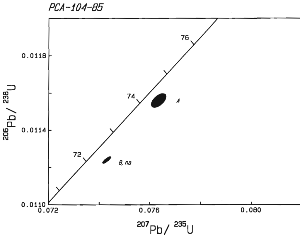
Figure 16. U-Pb concordia diagram for zircon from sample 14, PCA-104-85.
