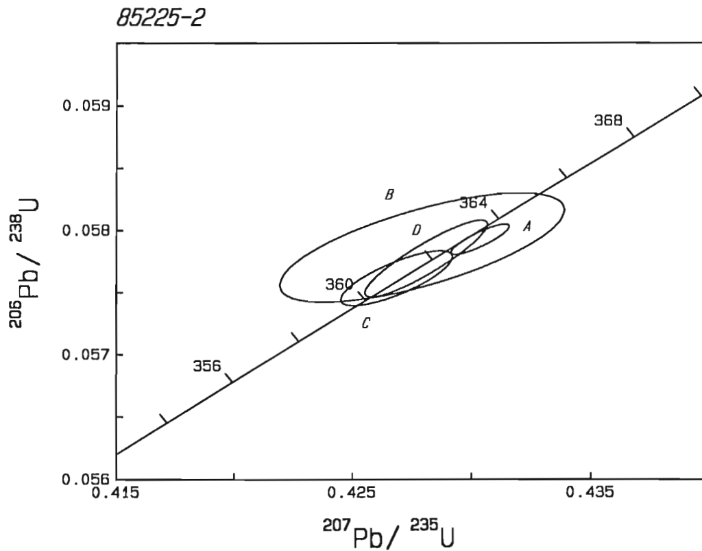
Figure 3. U-Pb concordia diagram of sample 85225-2, Saltspring Intrusion. Error ellipses reflect 2\sigma uncertainty.
