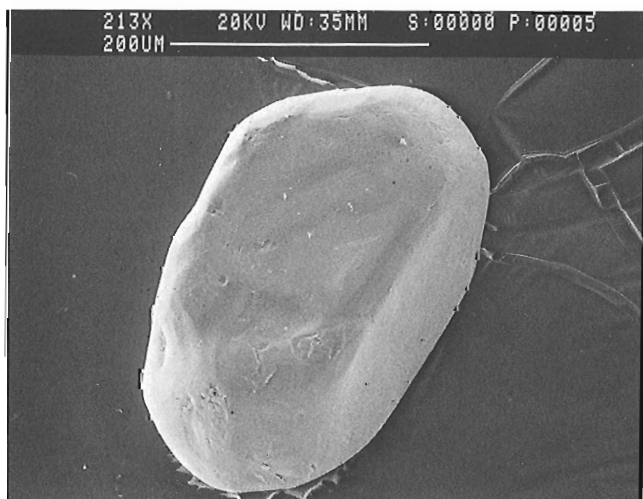
Figure 5. A scanning electron microscope (SEM) photomicrograph from a grain mount showing a typical zircon, similar to those in Figure 4. Note the equant, generally rounded morphology.
