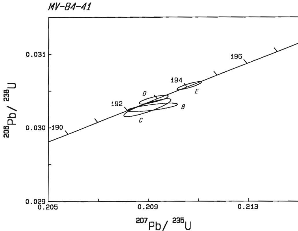
Figure 4b. U-Pb concordia plot of data points from MV-84-41 clustered near concordia. Error ellipses reflect the 2\sigma uncertainty.
