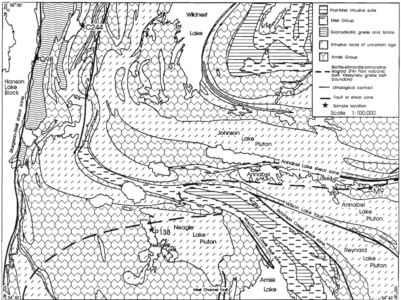
Figure 2. Simplified geological map showing the western sample locations.
