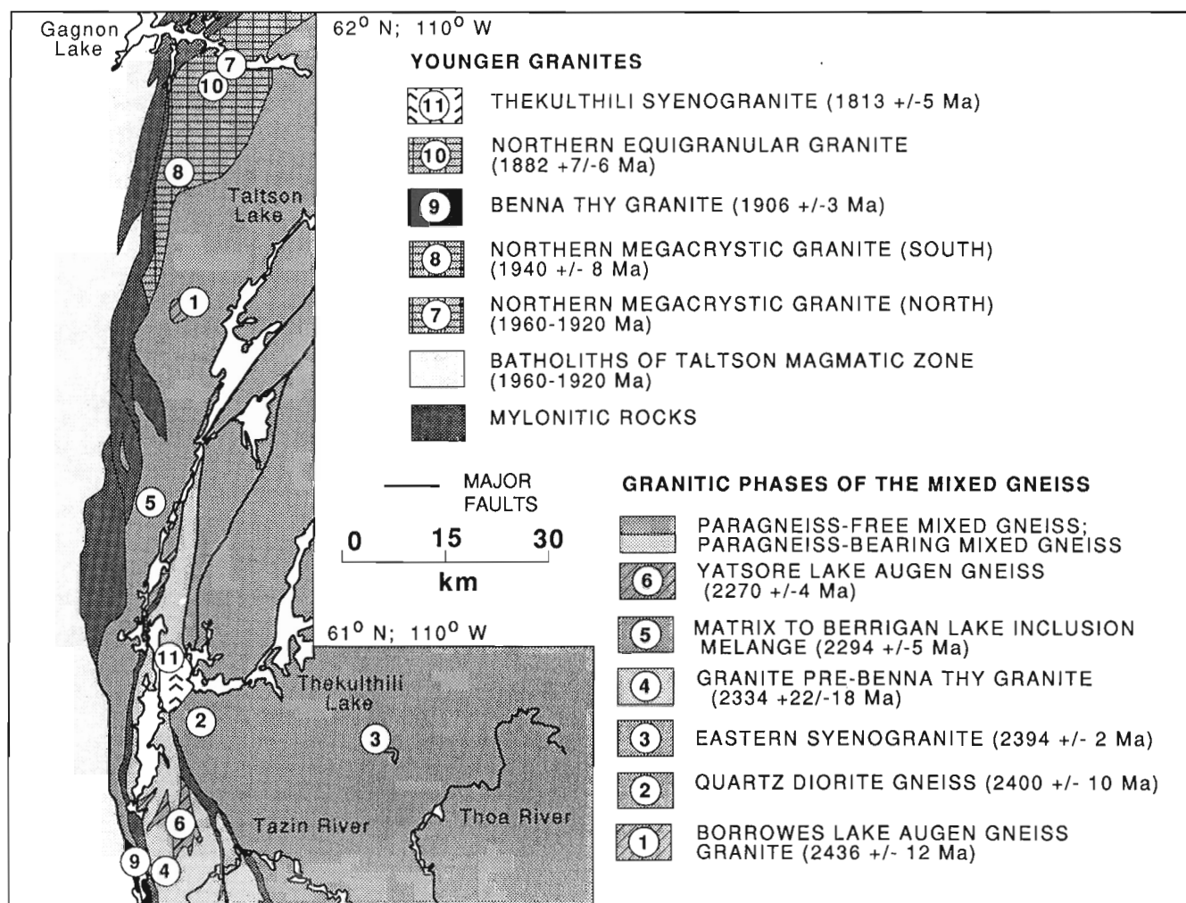
Figure 1. Plutonites of the mapping corridor along the western margin of the Rae Province. These plutonites comprise two zones of mixed granite and gneiss characterized by the presence and near absence of paragneiss. Granitic phases dated are listed in the legend in order of decreasing U-Pb zircon, monazite or sphene age. Sources: localities 2,3,7,8 and 10 (this study); localities 1,4 and 9 (Bostock and Loveridge, 1988); localities 5 and 6 (Bostock et al., 1991). Supracrustal rocks (eg. Nonacho Group) are not shown.
