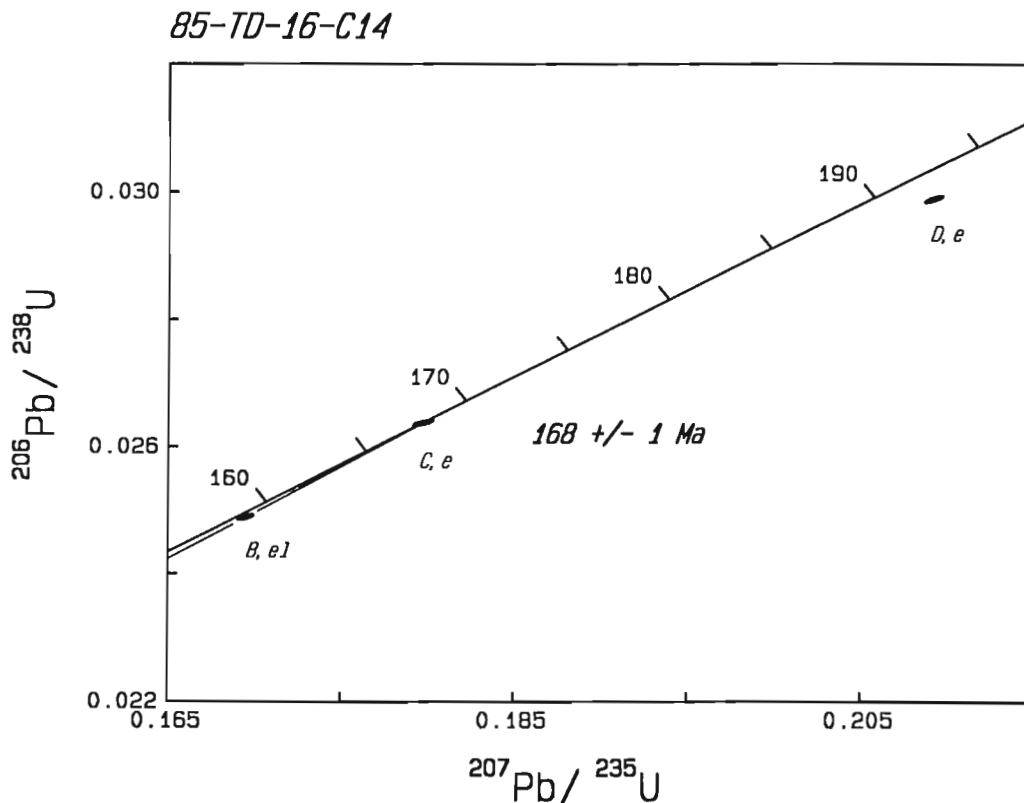
Figure 2. U-Pb concordia diagram for sample 85-TD-16-C14, a syenite boulder from the Uslika conglomerate. Error ellipses reflect 2σ uncertainty.
