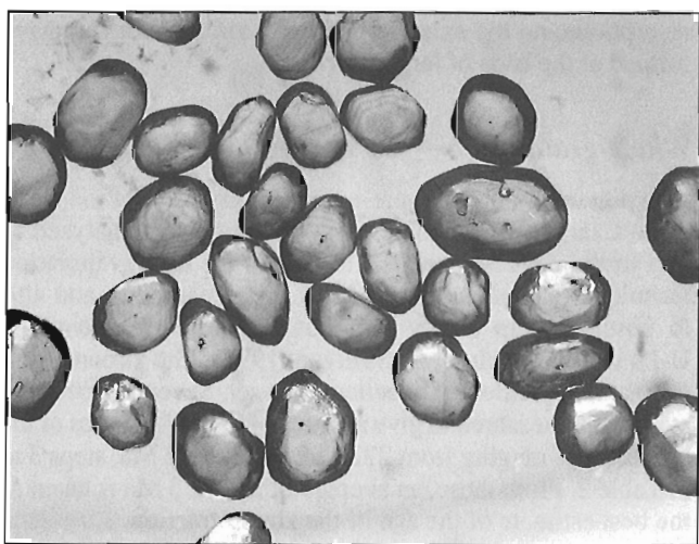
Figure 4. A photomicrograph of a picked aliquot of the large equant zircons that are typical of the bulk of the zircon from the sample. These belong to the ca. 2725 Ma age group.
