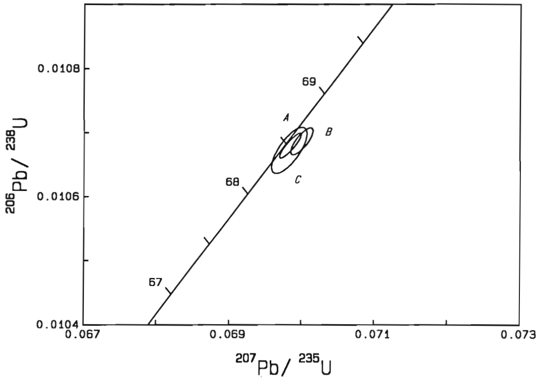
Figure 17. U-Pb concordia plot for MC-88-119, foliated hornblende-biotite granite. Error ellipses reflect the 2\sigma uncertainty.
