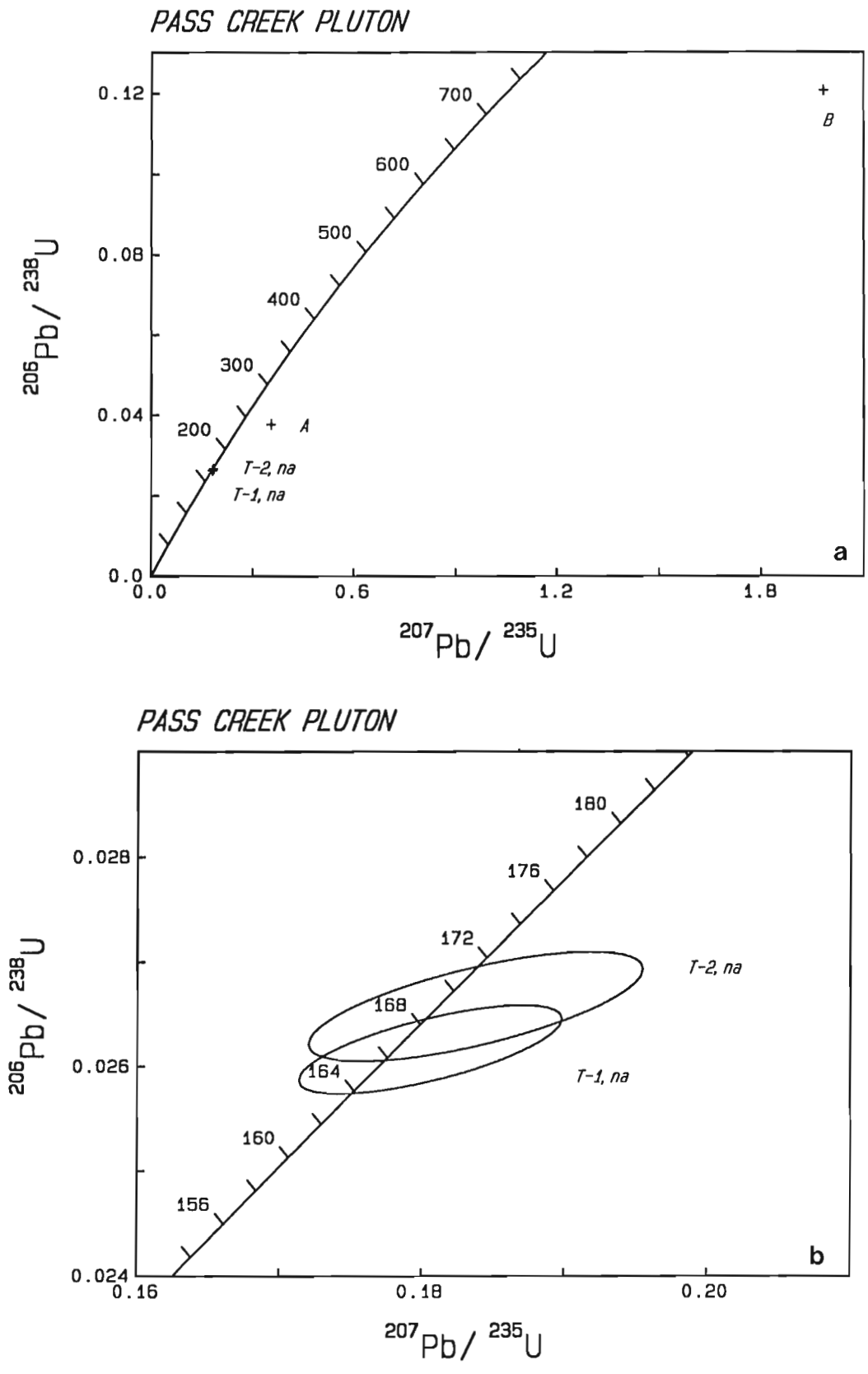
Figure 4. U-Pb concordia diagram of zircon and titanite data from the Pass Creek Pluton. Error ellipses are 2\sigma .
