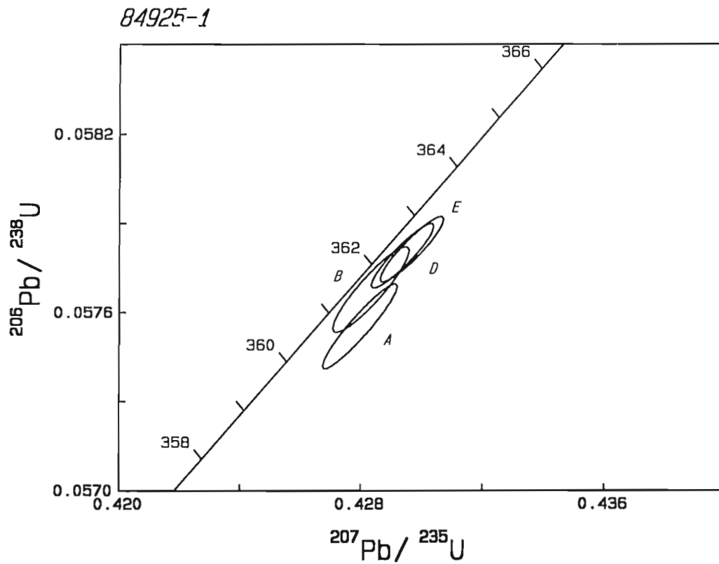
Figure 2. U-Pb concordia diagram of Sample 84925-1, Saltspring Intrusion. Error ellipses reflect 2\sigma uncertainty.
