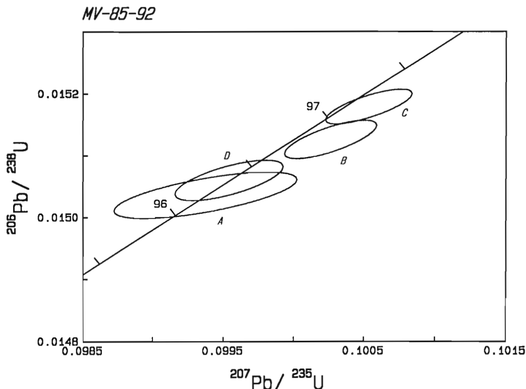
Figure 9. U-Pb concordia plot of MVH-85-92, gneissic quartz diorite. Error ellipses reflect the 2\sigma uncertainty.
