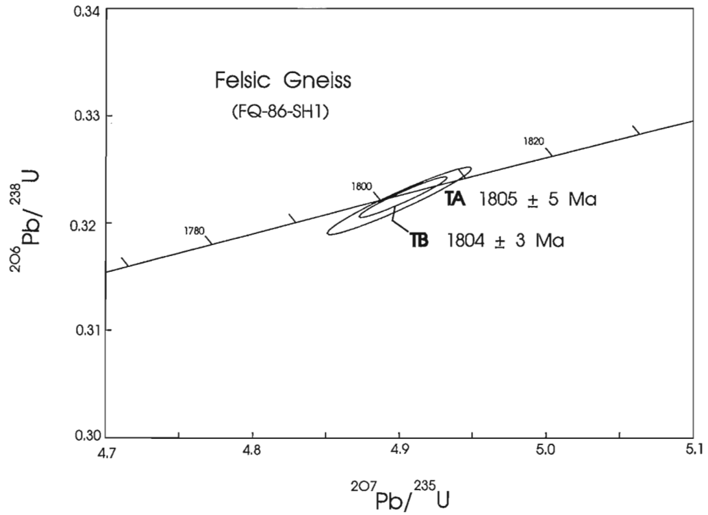
Figure 7. Concordia diagram showing results of titanite analyses from felsic gneiss FQ-86-SH1, Sherridon, Manitoba.
