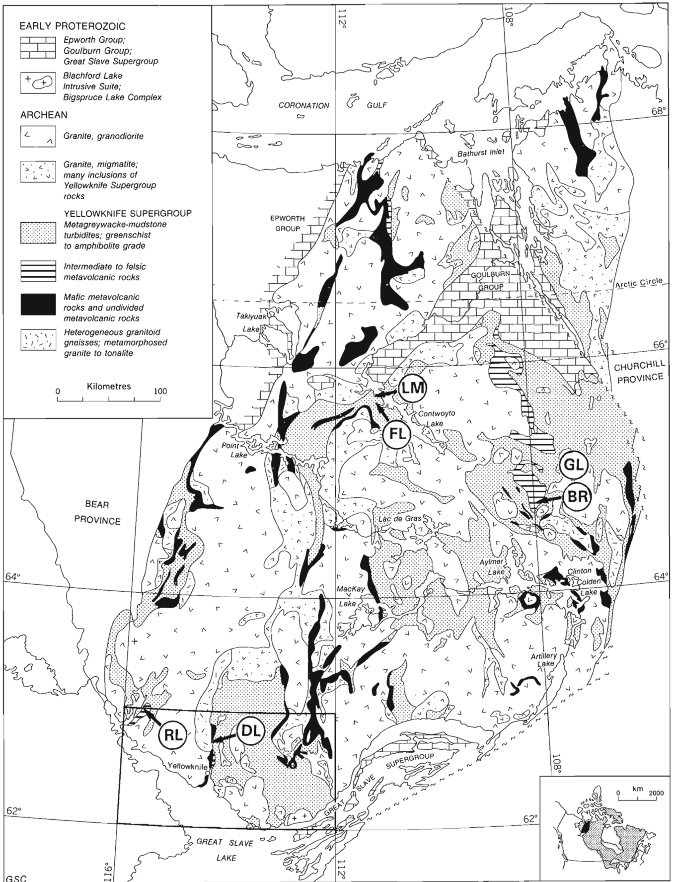
Figure 1. Locations of dated iron-formations in the Slave Province (modified from Henderson, 1985). FL = Fingers Lake; LM = Lupin gold mine; GL = George Lake; BR = Back River; DL = Dwyer Lake; RL = Russell Lake.
