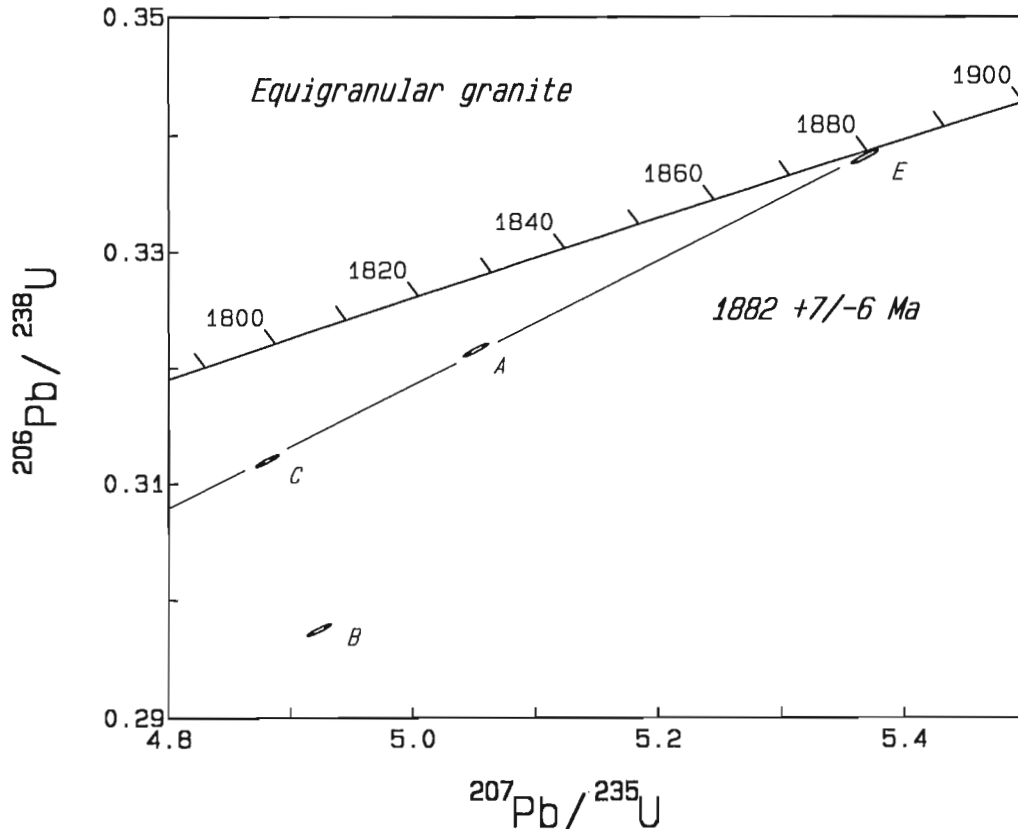
Figure 5. U/Pb isotope ratio plot showing zircon data points with error envelopes for equigranular northern granite (89BK-12X). Letters with data points correspond to those of Table 1.
