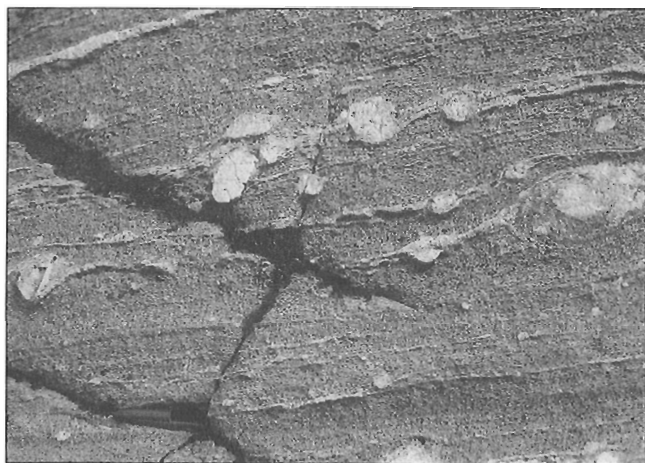
Figure 9. Rotated winged feldspars and granitoid segregations indicating a dextral component of shear in the Sturgeon-weir Shear Zone.
