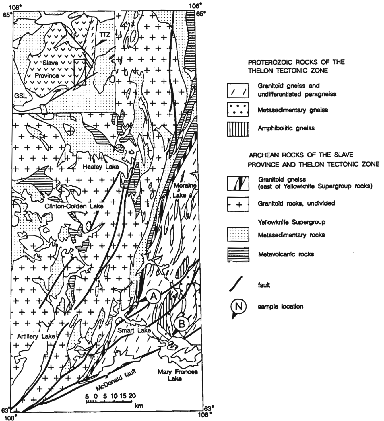
Figure 1. Geology of the Healey Lake - Artillery Lake area at the boundary between the Slave Province and the Thelon Tectonic Zone (inset). Location of the two samples analyzed are indicated. Sample A - granitoid gneiss east of last Archean Yellowknife Supergroup supracrustal rocks at Smart Lake; Sample B - Mary Frances metasedimentary gneiss north of Mary Frances Lake. TTZ - Thelon Tectonic Zone; GSL - Great Slave Lake.
