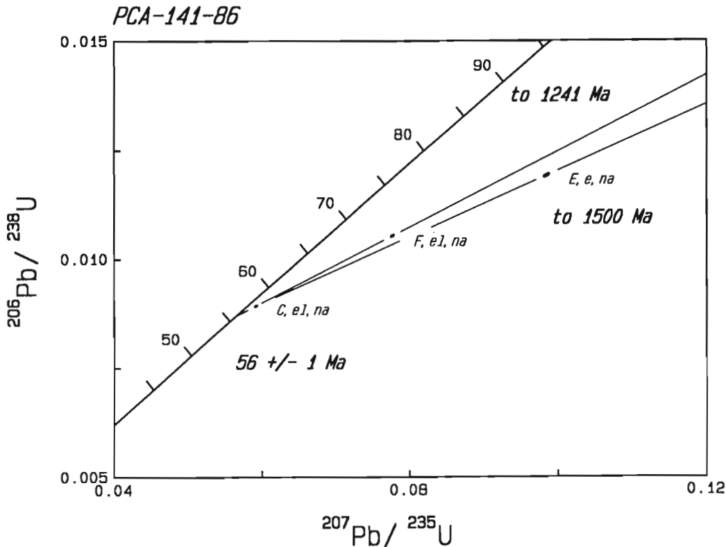
Figure 2. Concordia diagram for U-Pb data from sample PCA-141-86. Error ellipses reflect 2\sigma uncertainty.
