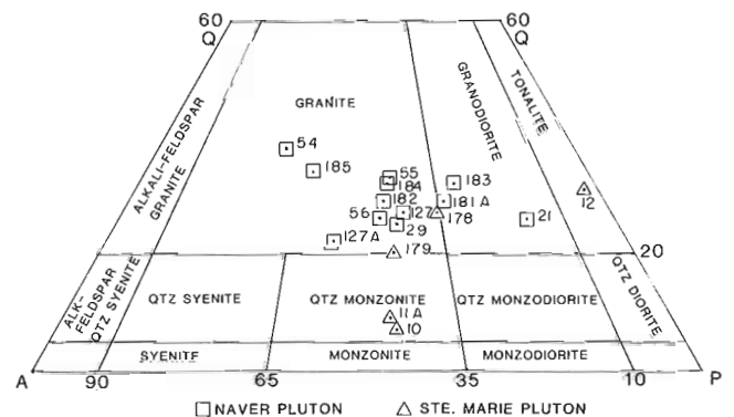
Figure 2. Classification of the point counted specimens from the Naver and Ste Marie plutons, where A = Alkali Feldspar, Q = Quartz, and P = Plagioclase. Table 1 has the percentage relative concentrations of the macroscopic rock forming minerals.
