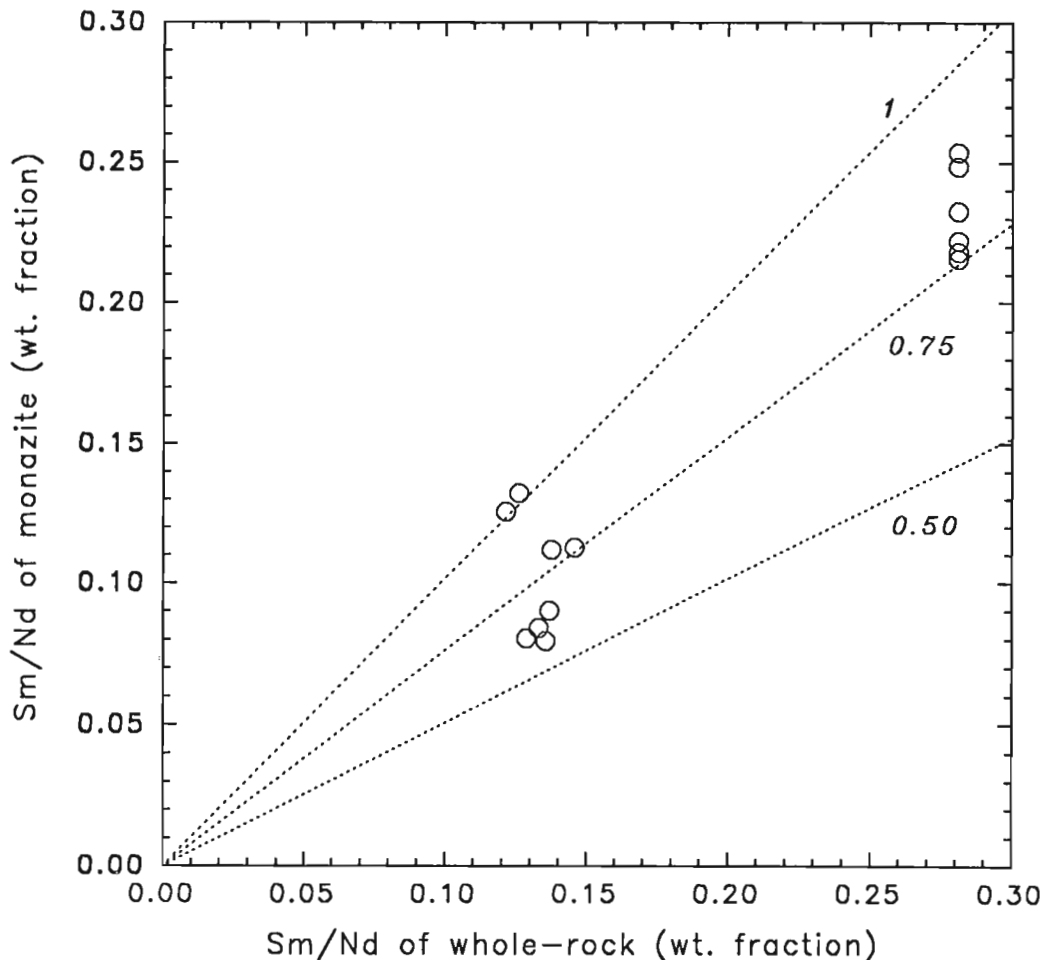
Figure 2. Sm/Nd ratios in monazites vs. the Sm/Nd ratios of whole-rock samples of the host granitoids.
