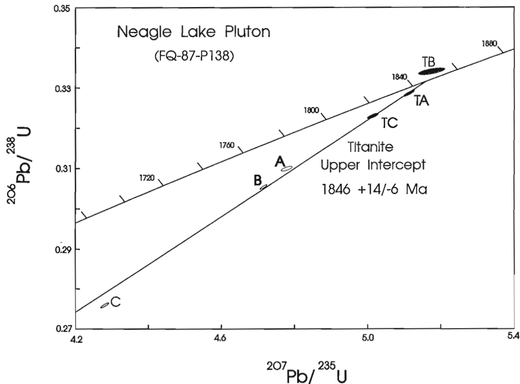
Figure 3. Concordia diagram showing U-Pb results from the Neagle Lake Pluton (FQ-87-P138).
