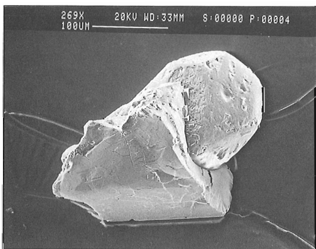
Figure 8. A photomicrograph of a dark brown zircon with a thick, obvious overgrowth. Fraction X represents one of these zircons which are rare (high uranium), and very different from the other zircons in the sample. Energy dispersive x-ray (EDX) analyses confirmed both phases were zircon.
