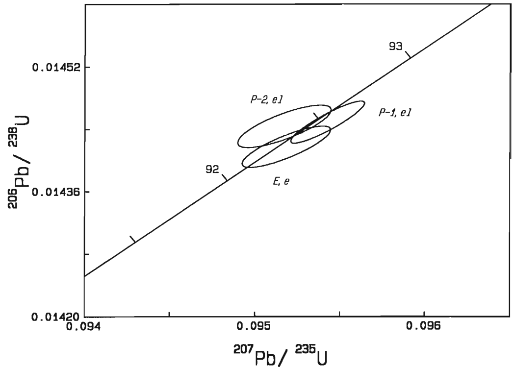
Figure 4. Concordia plot for zircons from sample 86-WV-2. Error ellipses reflect 2\sigma uncertainty.
