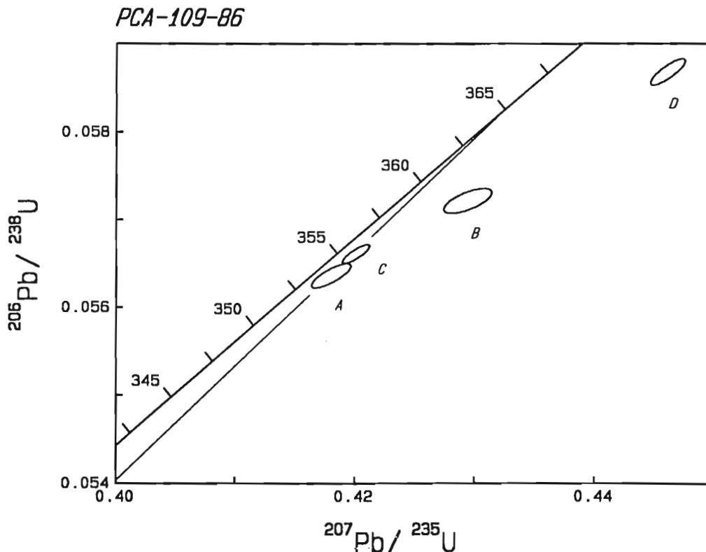
Figure 5. Concordia diagram for U-Pb data from sample PCA-109-86. Error ellipses reflect 2\sigma uncertainty.
