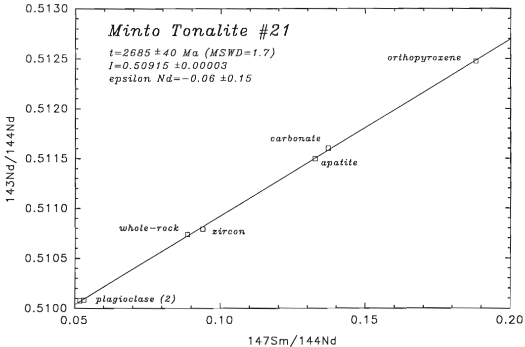
Figure 6. Mineral isochron for tonalite sample #21 from the Minto block.
