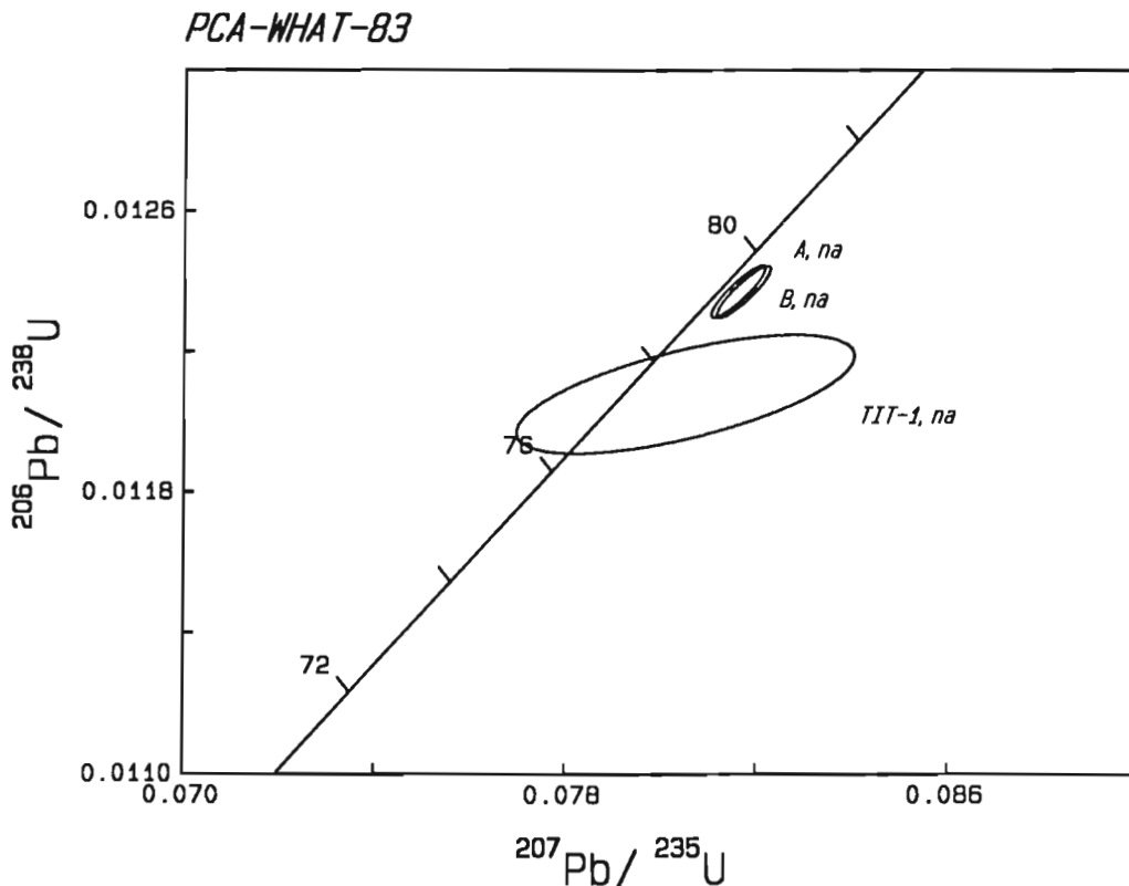
Figure 13. U-Pb concordia diagram for zircon and allanite from sample 12, PCA-WHAT-83.
