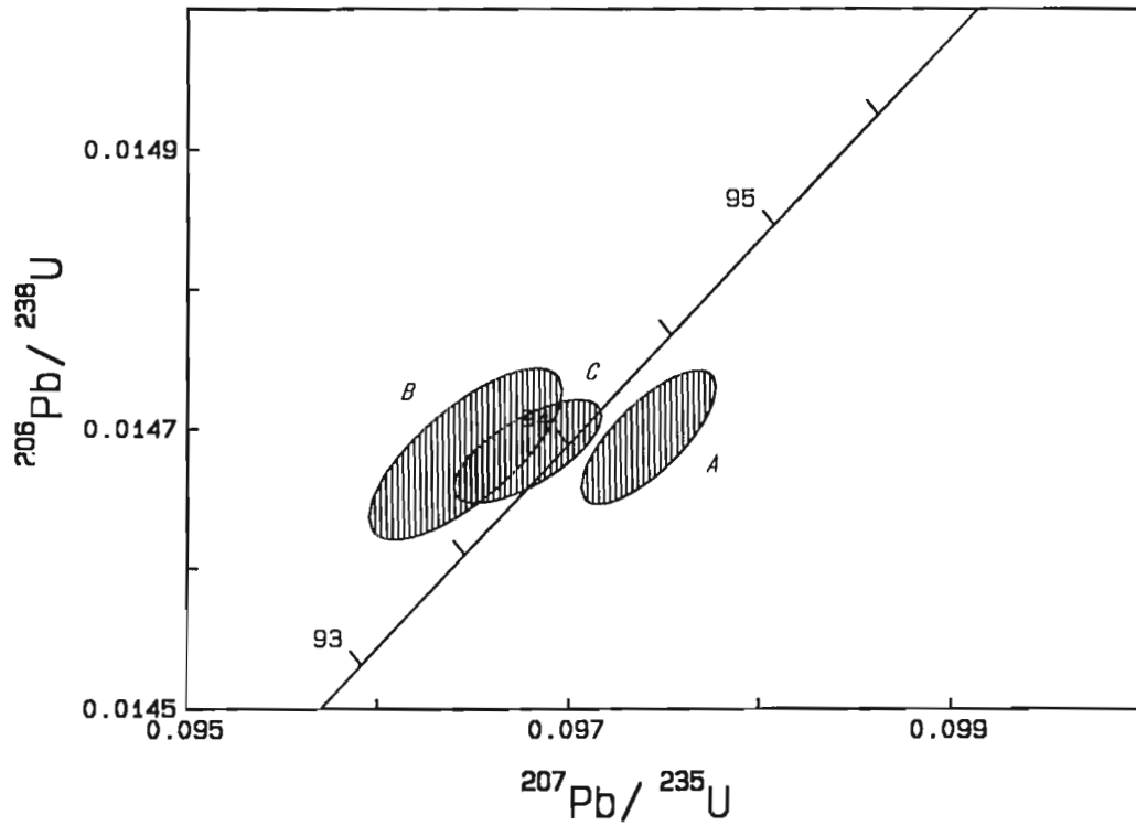
Figure 11. U-Pb concordia plot of MVD-89-375, the Snowcap Lake Pluton. Error ellipses reflect the 2\sigma uncertainty.
