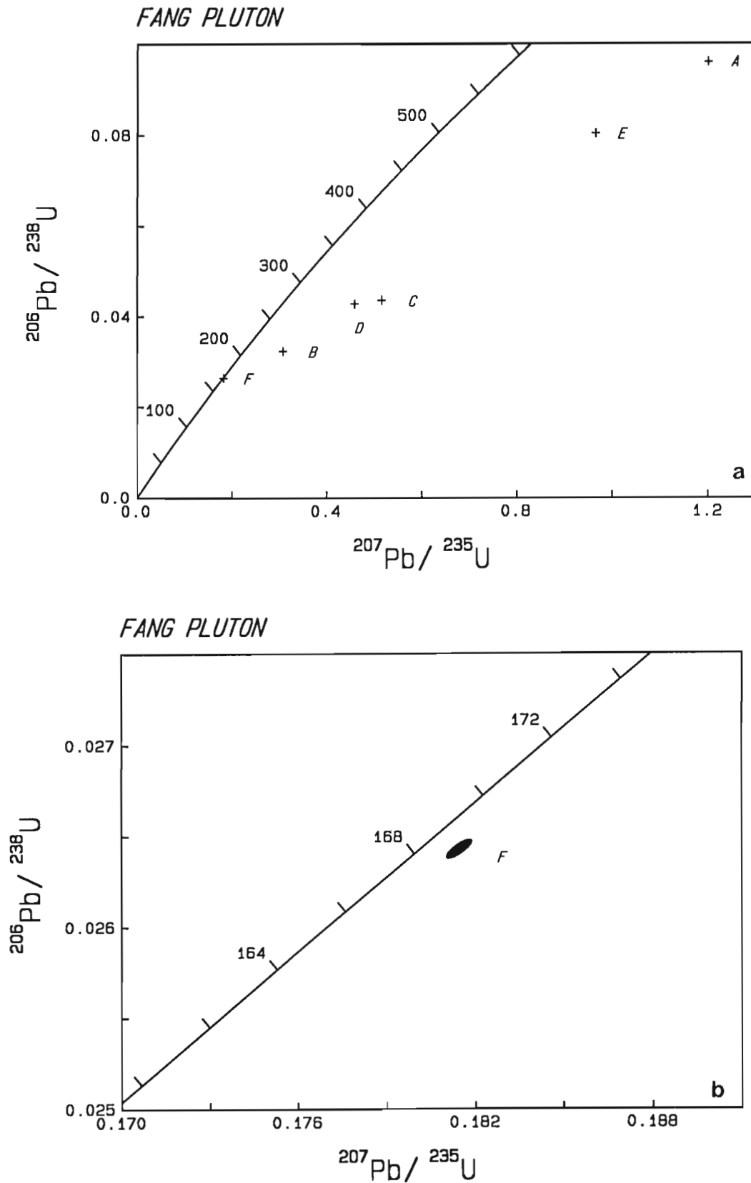
Figure 3. U-Pb concordia diagram of zircon data from the Fang Pluton. Error ellipses are 2\sigma .
