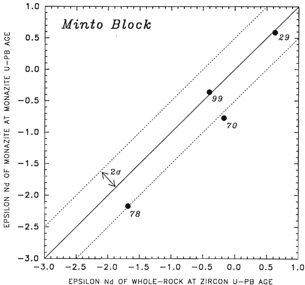
Figure 3. Comparison of epsilon Nd values of monazites and whole-rocks from the Archean Minto block.
