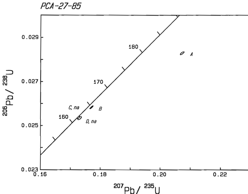
Figure 9. U-Pb concordia diagram for zircon from sample 8, PCA-27-85.
