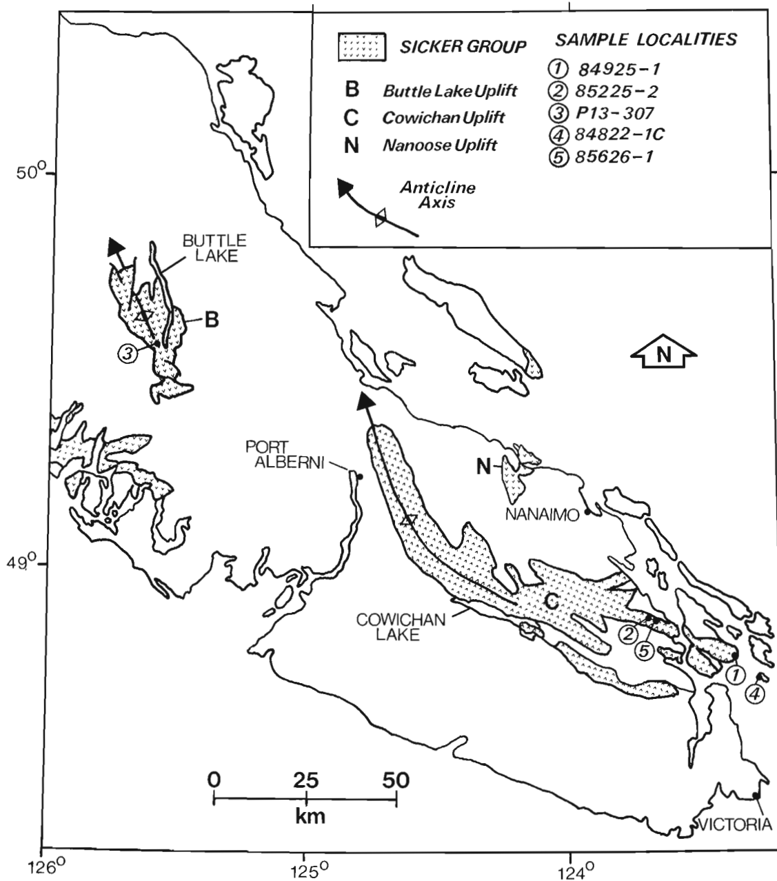
Figure 1. Map of southern Vancouver Island area with the three major anticlinal uplifts cored by Sicker Group rocks outlined (after Brandon et al., 1986; their fig. 1). Sample localities for U-Pb dating are plotted.
