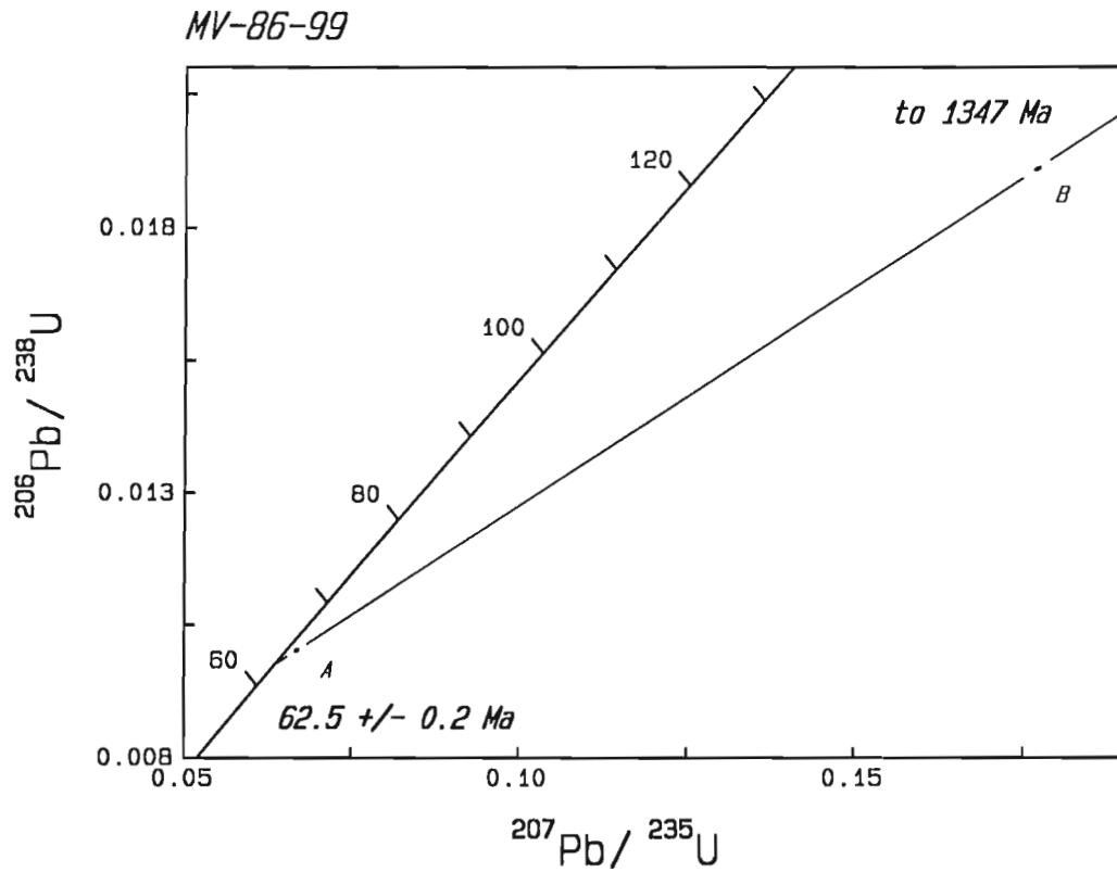
Figure 13. U-Pb concordia plot of MV-86-99, quartz-felspar porphyry. Error ellipses reflect the 2\sigma uncertainty.
