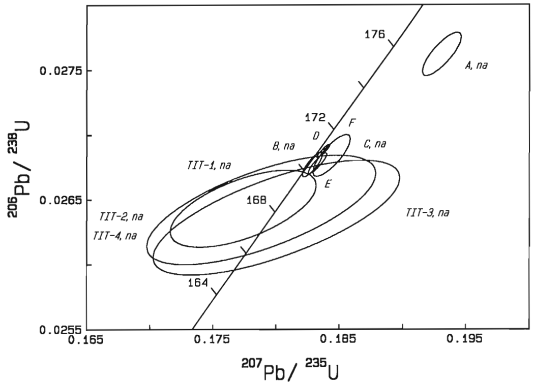
Figure 3. U-Pb concordia diagram for zircon and titanite from sample 2, PCA-452-83-SY; na, not abraded.
