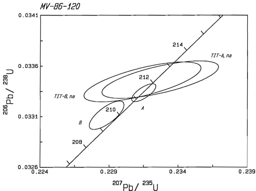
Figure 2. U-Pb concordia plot of MV-86-120, massive granodiorite of the Mount Lytton Complex. Error ellipses reflect the 2\sigma uncertainty.
