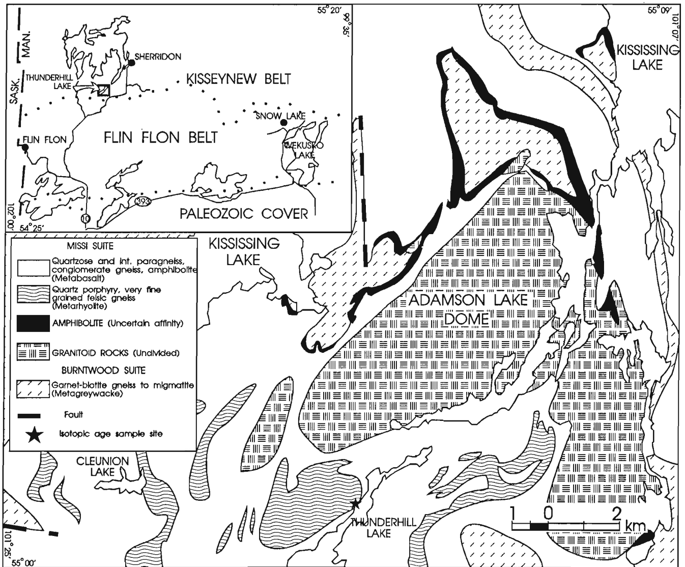
Figure 1. U-Pb zircon sample location and simplified geology of the Thunderhill Lake area, Manitoba.
