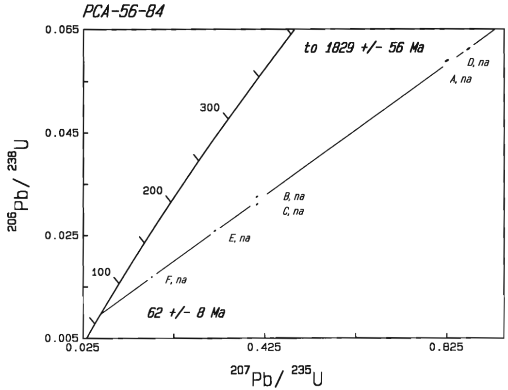
Figure 15. U-Pb concordia diagram for zircon from sample 13, PCA-56-84.
