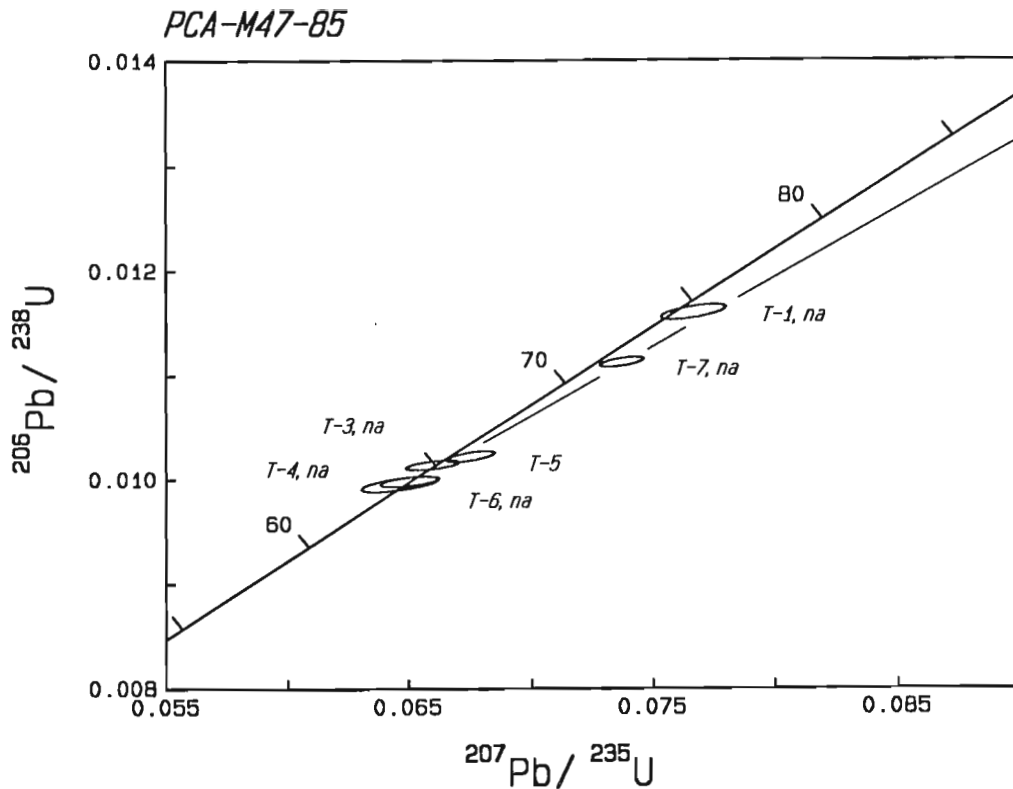
Figure 8. Concordia diagram for titanite U-Pb data from sample PCA-M47-85. A reference line from 63 to 359 Ma is included. Error ellipses reflect 2\sigma uncertainty.
