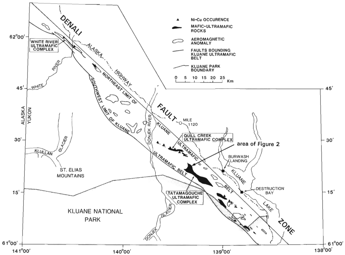
Figure 1. Map showing the regional setting and distribution of mafic and ultramafic intrusive bodies of the Kluane ultramafic belt in southwestern Yukon.
