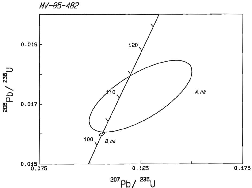
Figure 8b. U-Pb concordia plot of data points from MV-85-482 plotting on concordia. Error ellipses reflect the 2\sigma uncertainty.
