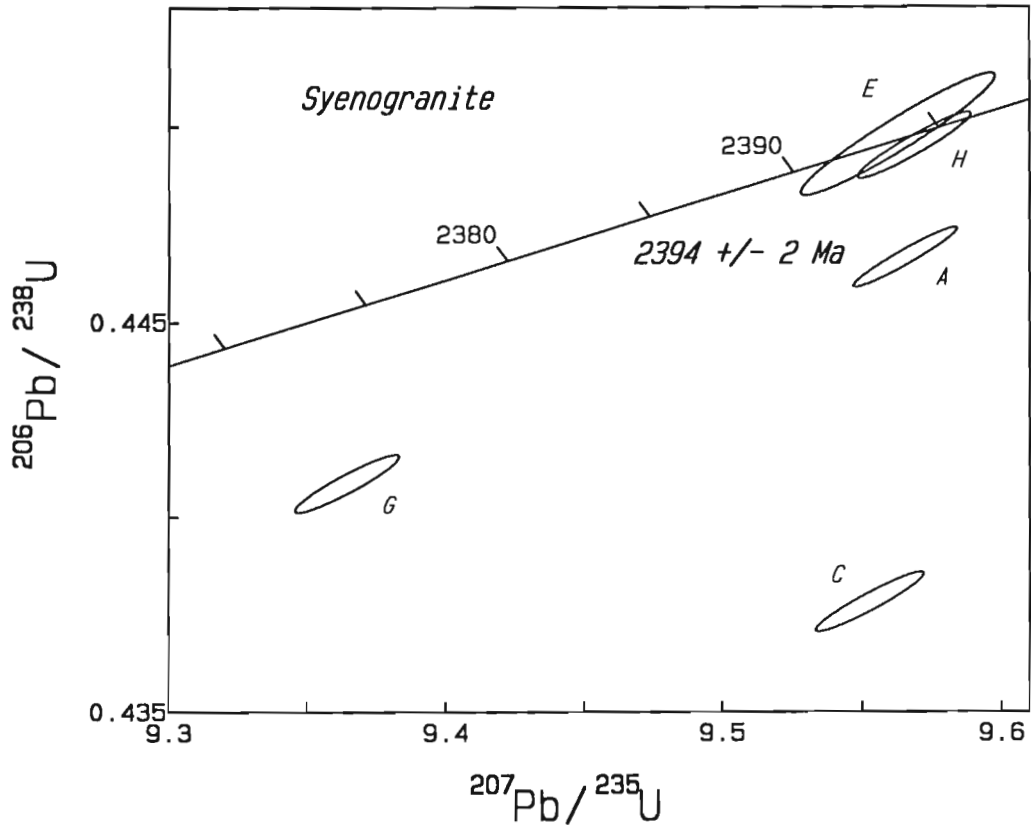
Figure 3. U/Pb isotope ratio plot showing zircon data points with error envelopes for Syenogranite (88BK-172X). Letters with data points correspond to those of Table 1.
