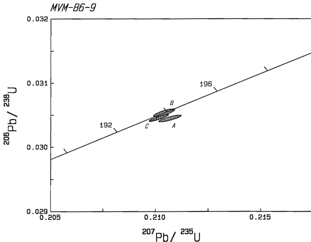
Figure 5. U-Pb concordia plot of MVM-86-9, granodiorite of the Pennask Batholith. Error ellipses reflect the 2\sigma uncertainty.
