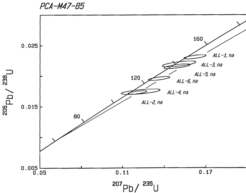
Figure 7. Concordia diagram for allanite U-Pb data from sample PCA-M47-85. A reference line from 63 to 359 Ma is included. Error ellipses reflect 2\sigma uncertainty.
