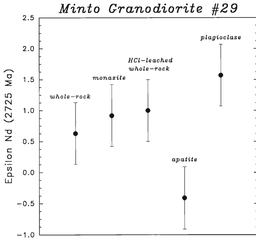
Figure 5. Comparison of epsilon Nd values of minerals from granodiorite sample #29 at the zircon crystallization age of 2725 Ma.
