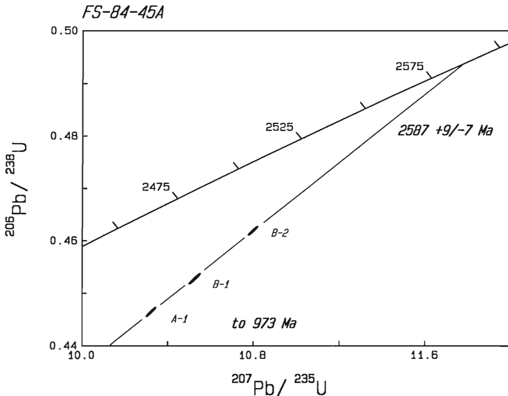
Figure 3. U-Pb concordia diagram for sample FS-84-45A. Error ellipses are 2σ.
