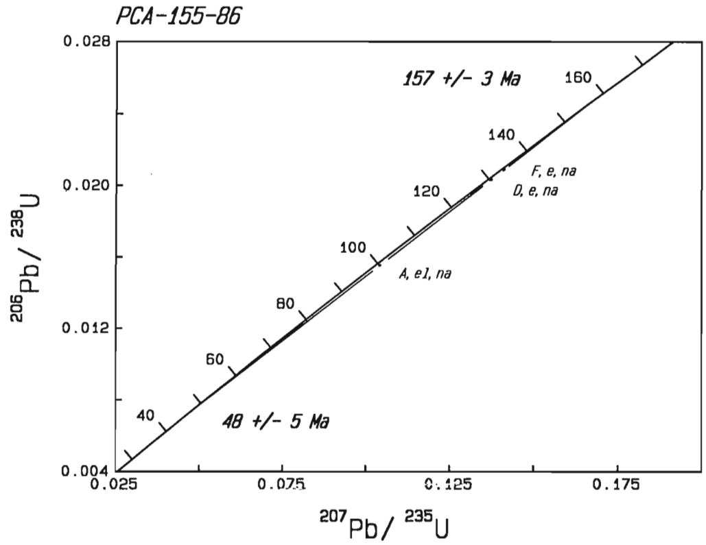
Figure 3. Concordia diagram for U-Pb data from sample PCA-155-86. Error ellipses reflect 2\sigma uncertainty.
