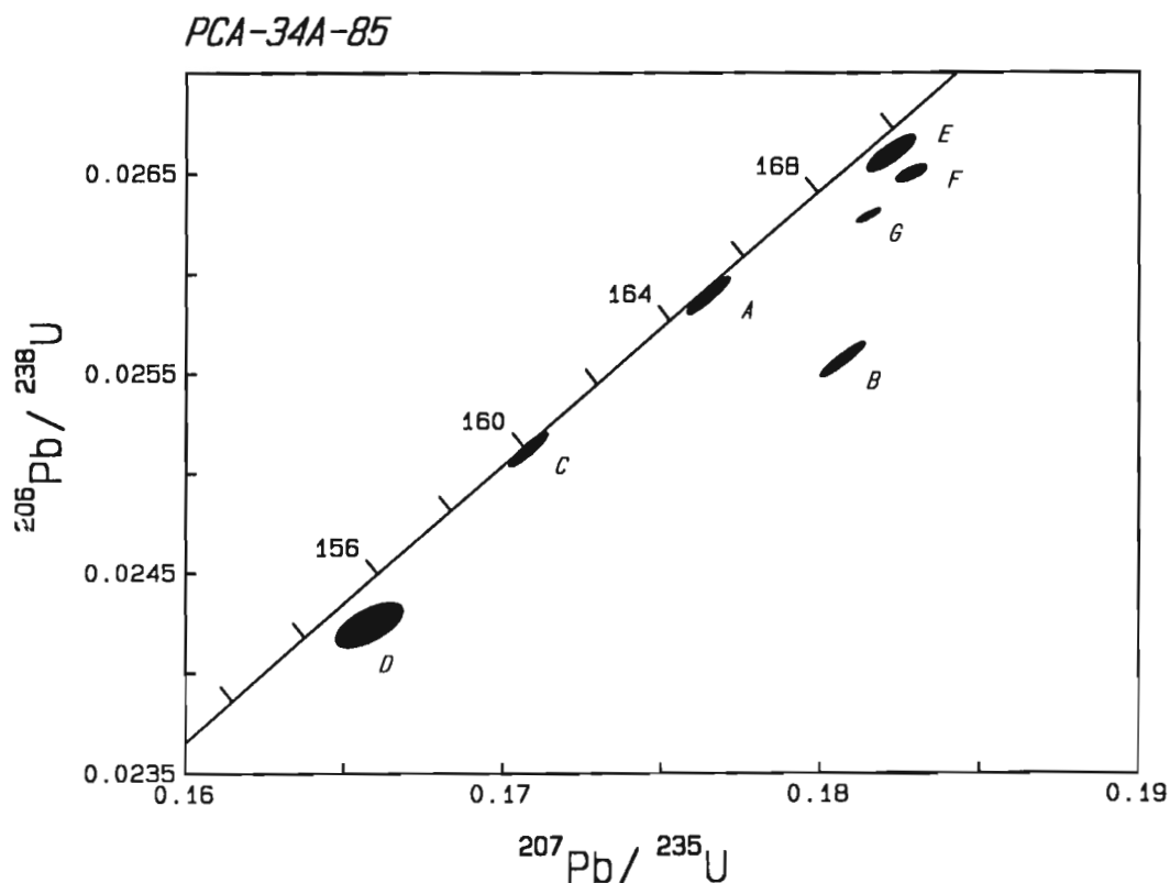
Figure 4. U-Pb concordia diagram for zircon from sample 3, PCA-34A-85.
