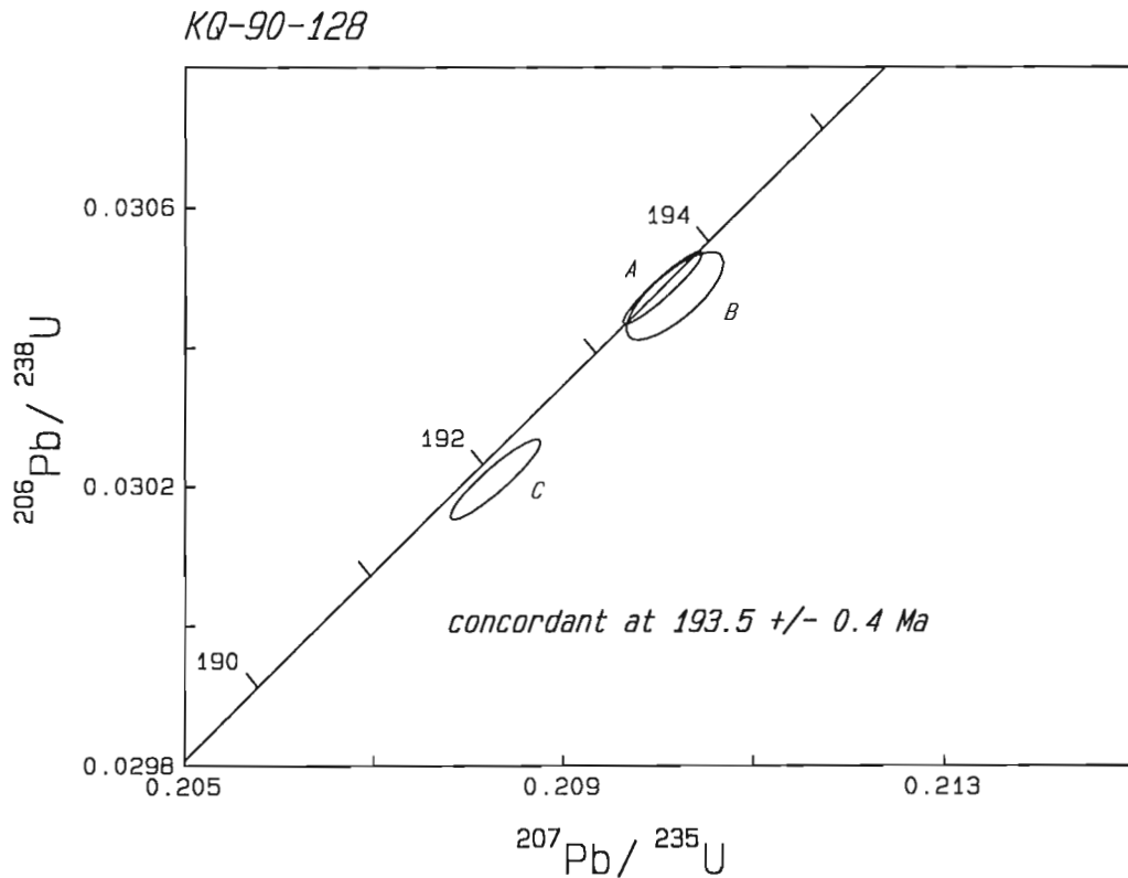
Figure 3. U-Pb concordia plot for sample KQ-90-128.
