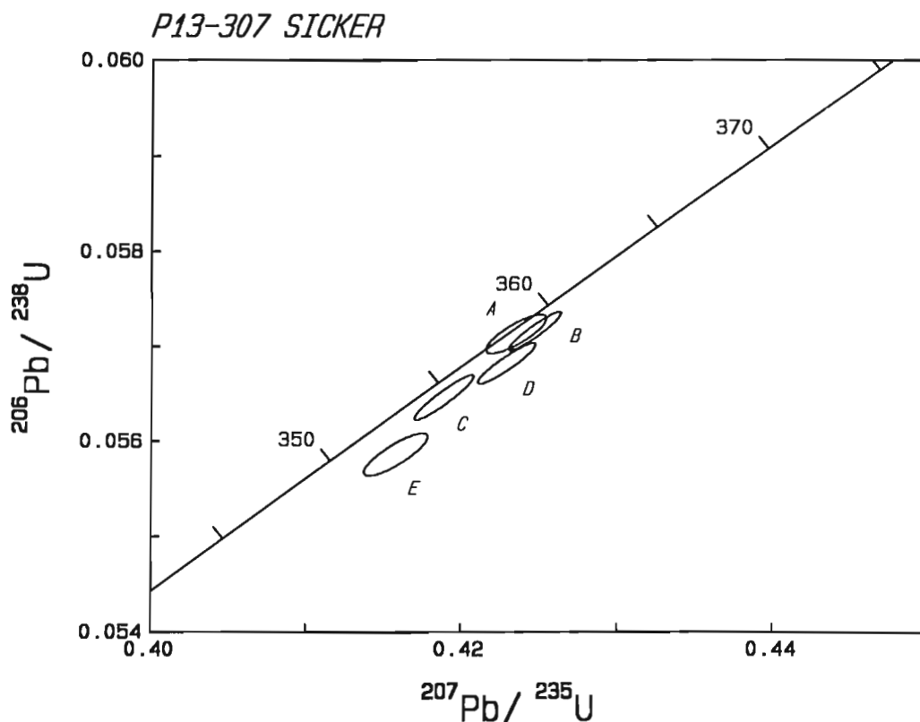
Figure 4. U-Pb concordia diagram of sample P13-307, Sicker rhyolite. Error ellipses reflect 2\sigma uncertainty.
