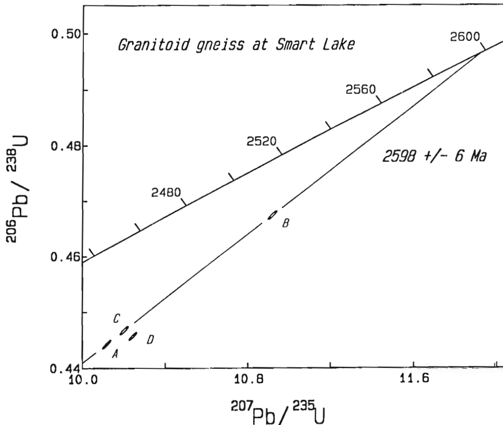
Figure 2. Concordia diagram for the granitoid gneiss at Smart Lake. Although the data are moderately discordant, the protolith of the deformed granitoid is Archean in age. Fraction D was excluded from the regression. Error ellipses are 2\sigma .
