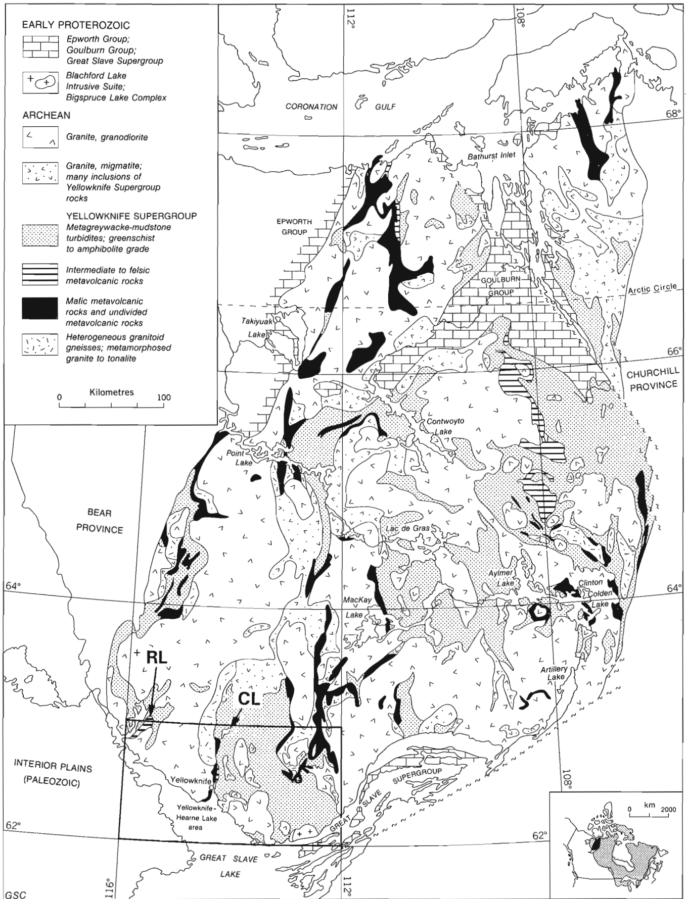
Figure 1. Simplified geological map of the Slave Province (modified from Henderson, 1985). RL = Russell Lake; CL = Clan Lake.
