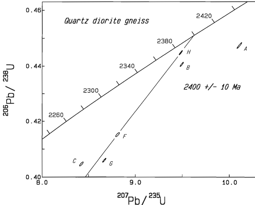
Figure 2. U/Pb isotope ratio plot showing zircon data points with error envelopes for Quartz diorite gneiss (87BK-366X). Letters with data points correspond to those of Table 1.
