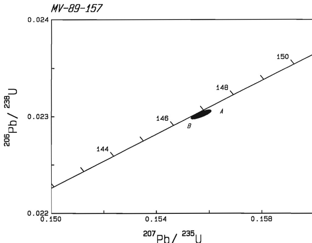
Figure 7. U-Pb concordia plot of MV-89-157, the Cloudburst quartz diorite. Error ellipses reflect the 2\sigma uncertainty. The data are not corrected for deficit of ^{206}\text{Pb} (see text).
