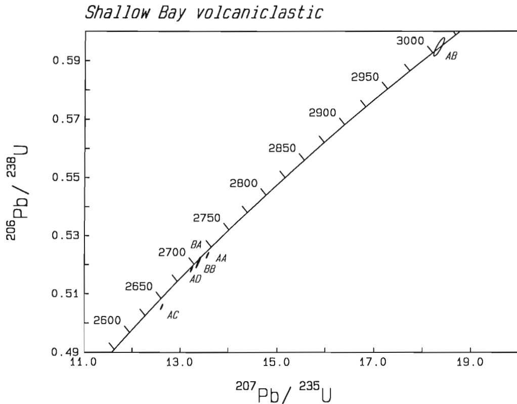
Figure 3. U-Pb concordia plot for single zircons from the Shallow Bay volcanics.
