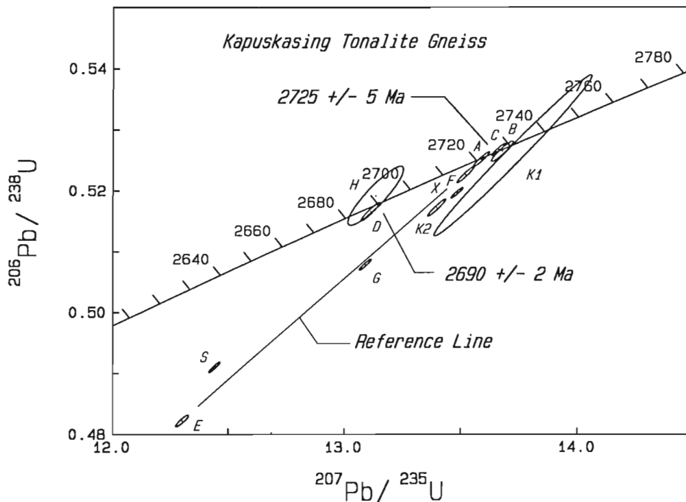
Figure 3. U-Pb concordia diagram for zircons from the Kapuskasing tonalite gneiss. There are zircons from two distinct age groups. The ca. 2725 Ma zircons have recorded a multi-event history for the tonalite (see text). The 2690 Ma zircons originated from tiny veinlets resulting from in situ melt. The reference line is drawn between fractions E and F which are a non abraded, abraded pair and is used to illustrate the two zircon populations. A regression line for fractions E, F and A yielded a 628 Ma lower intercept age.
