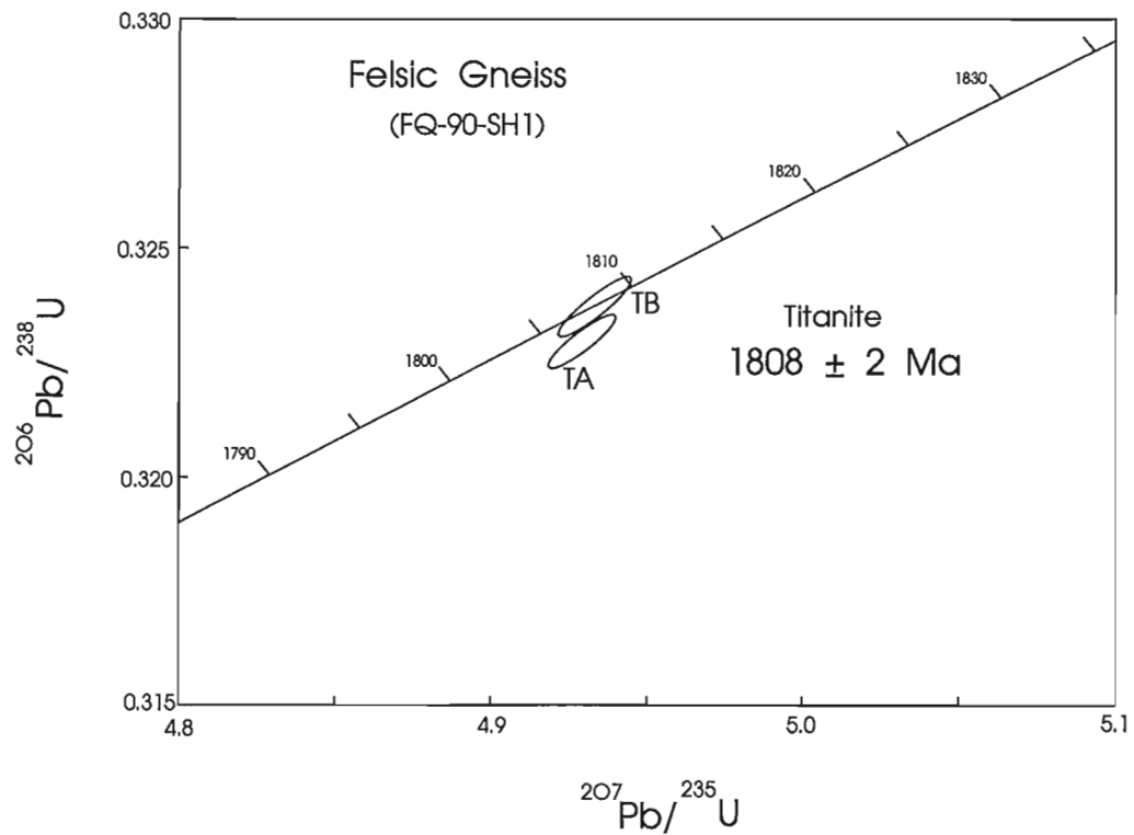
Figure 8. Concordia diagram showing results of titanite analyses from felsic gneiss FQ-90-SH1, Sherridon, Manitoba.
