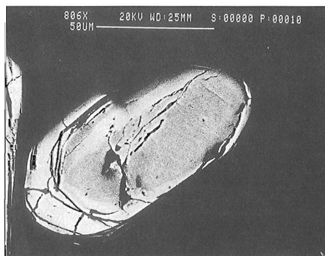
Figure 9. A SEM photomicrograph of zircon from a polished grain mount showing a core-overgrowth relationship. U-Pb analyses indicate the "core" is probably ca. 2728 Ma old, while the "overgrowth" is probably ca. 2722 Ma. The embayment is interpreted an evidence for resorption.
