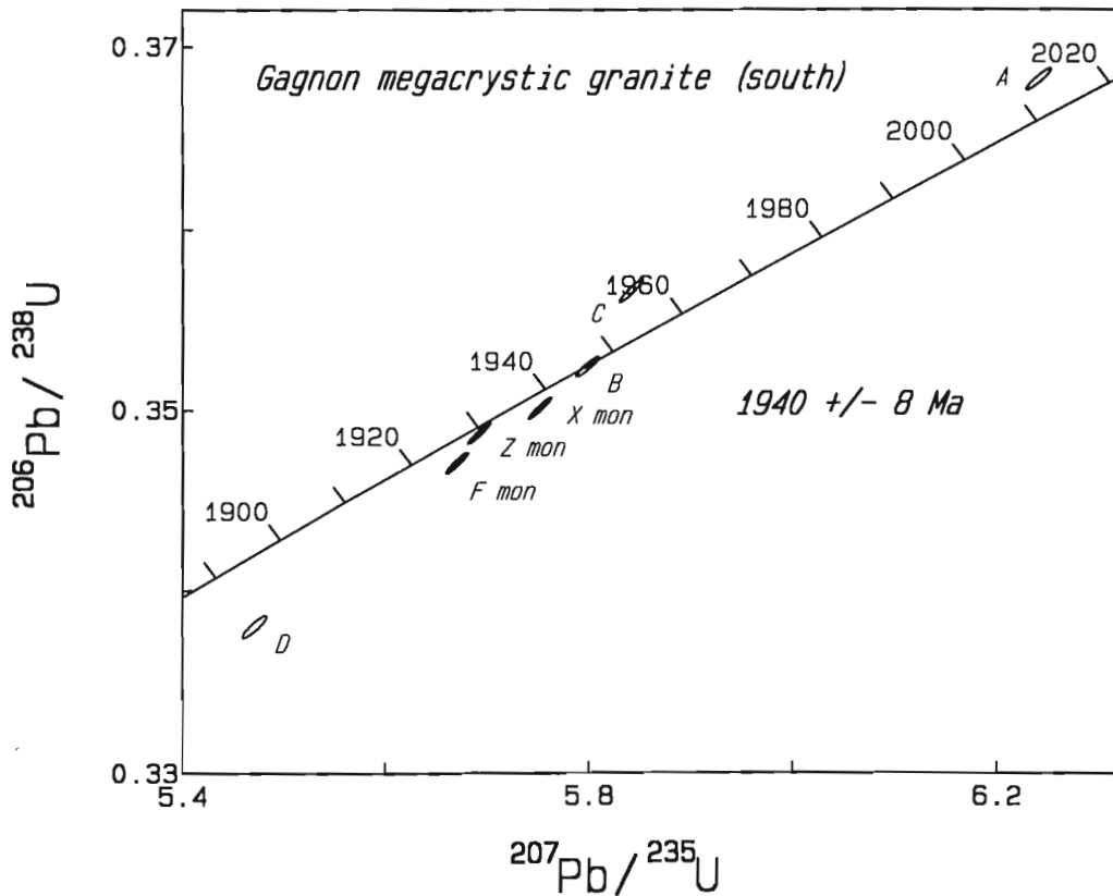
Figure 4. U/Pb isotope ratio plot showing zircon and monazite (Mon) data points with error envelopes for megacrystic northern granite (south, 89BK-10X). Letters with data points correspond to those of Table 1.
