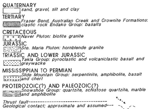
Figure 1. Regional geology around the Naver and Ste Marie plutons in central British Columbia. Sample sites for point counted specimens (triangles) and isotopically dated specimens (hexagons) are labelled to correspond with Table 1.
