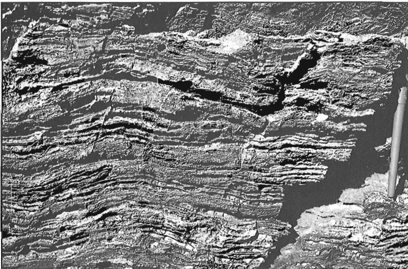
Figure 2. Typical well-bedded celestite (barite) from the Main showing, Kit property. Photograph is about 25 cm high (GSC 1991-390A).
