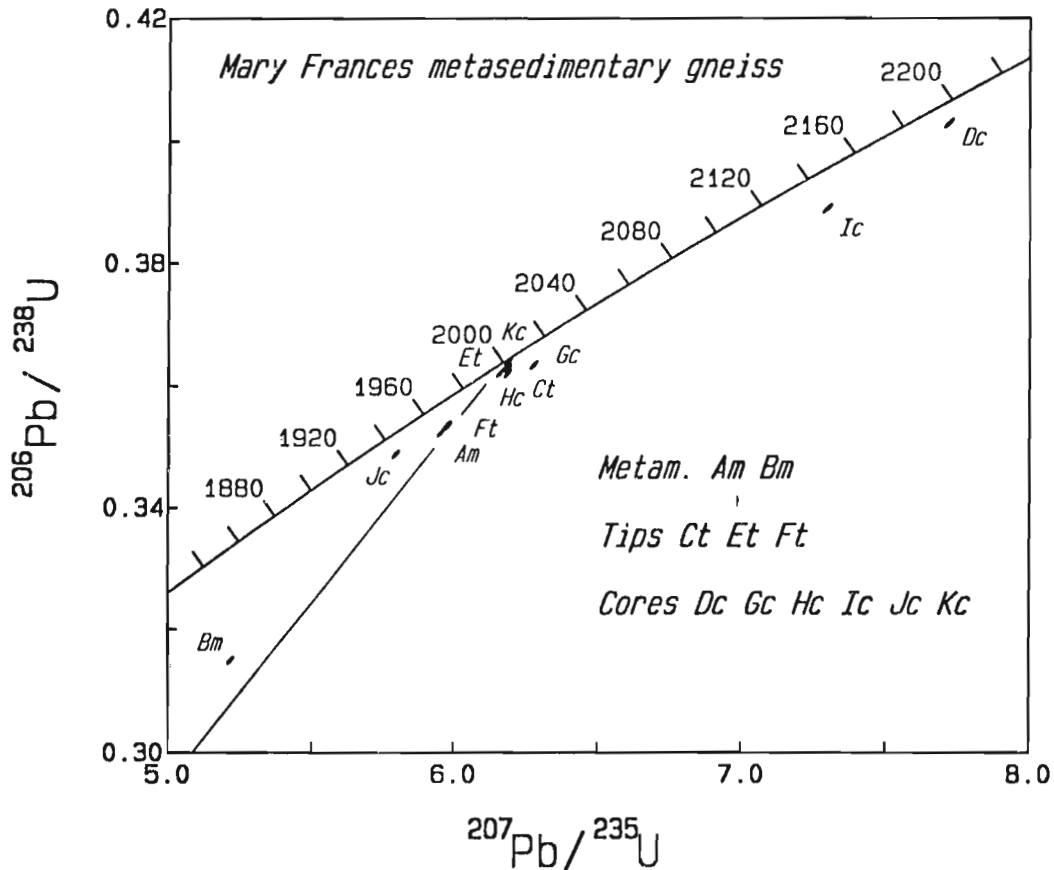
Figure 3. Concordia diagram for the Mary Frances metasedimentary gneiss. Although most of the fractions interpreted as core material are not distinguishable in age from those fractions interpreted as metamorphic in origin, two fractions are distinctly older. The data do not suggest any of the core material is Archean in age. Zircon fractions are classified as follows: Metam. = metamorphic zircon; Tips = zircon tips removed from core bearing grains; Cores = zircon cores isolated by removal of rim and tip material by breakage or abrasion. Error ellipses are 2%.
