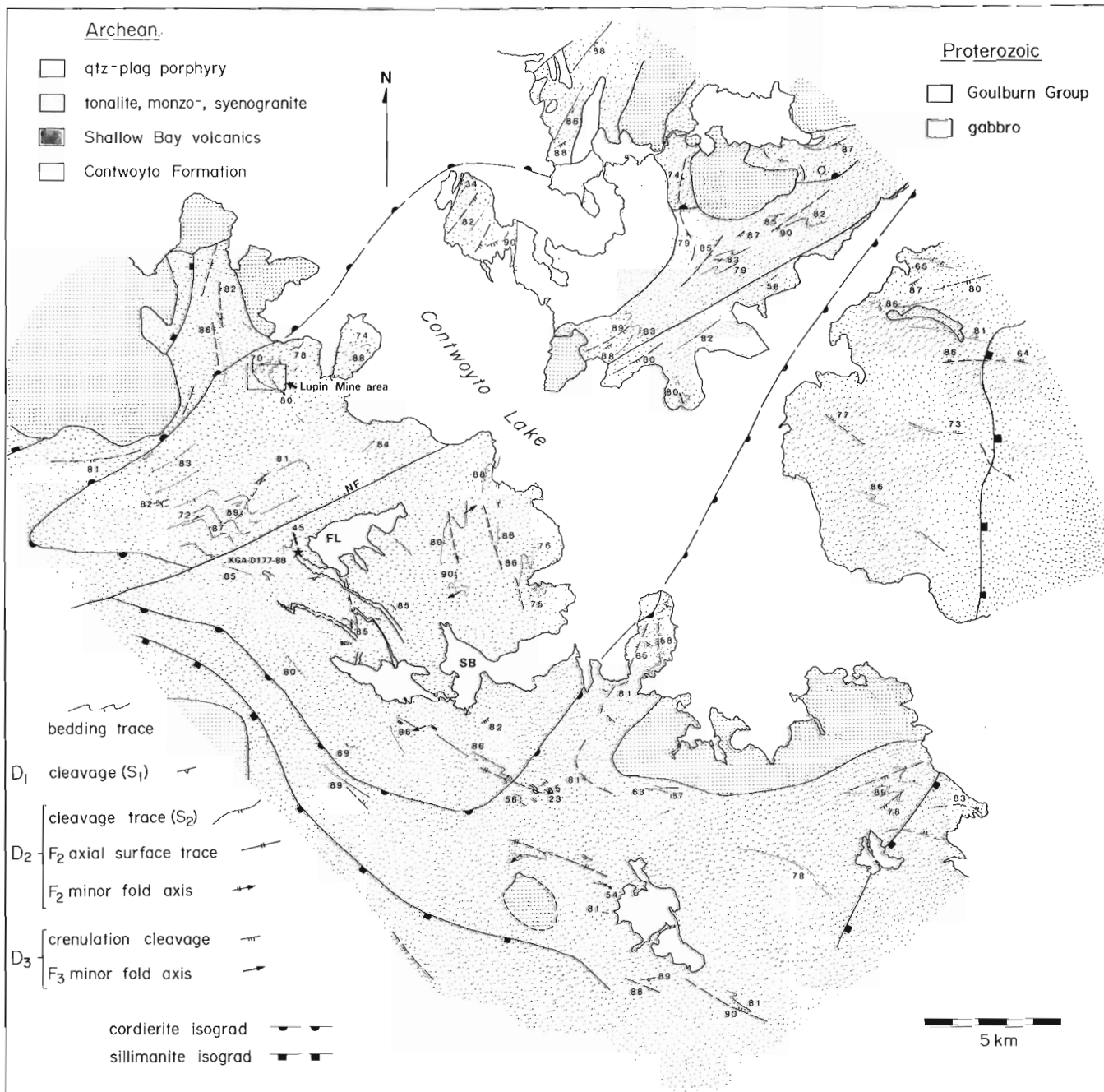
Figure 2. Simplified geological map of the Fingers Lake area. Sample locality is shown by the star. Geology by Relf (1989). FL = Fingers Lake; SB = Shallow Bay; NF = Norma Fault.
