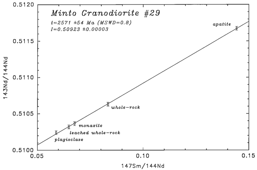
Figure 4. Mineral isochron for granodiorite #29 from the Minto block.
