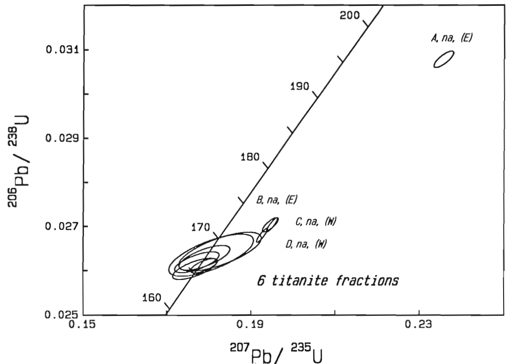
Figure 8. U-Pb concordia diagram for zircon and titanite from samples 6 and 7 of the Ruby Range stock, PCA-RRE-83 (6) and PCA-RRW-83 (7).
