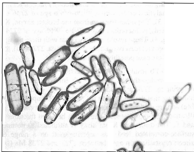
Figure 6. A photomicrograph of a picked aliquot of much less abundant, fine, \sim 74 \mu\text{m} zircon. The acicular morphology characterizes the group of zircons that are 2690 Ma old.
