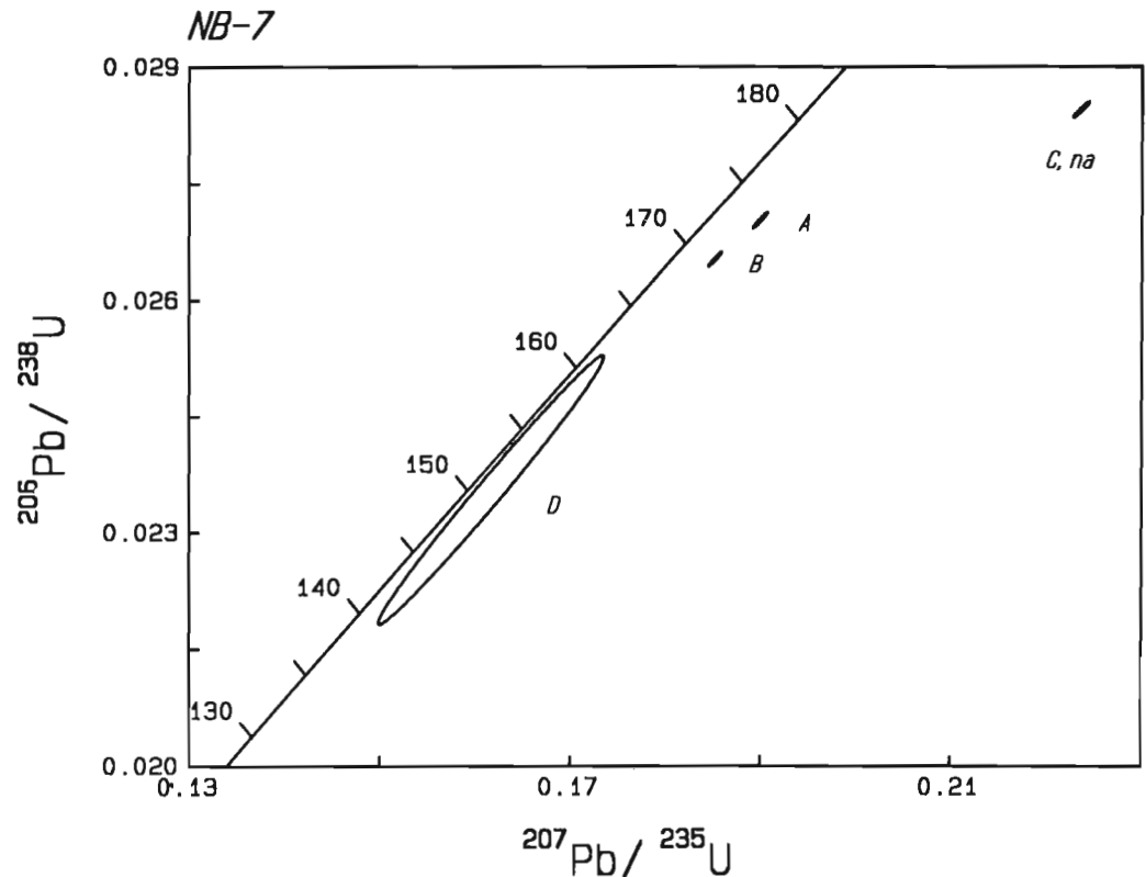
Figure 5. U-Pb concordia diagram for zircon from sample 4, NB-7.
