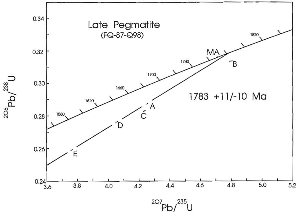
Figure 12. Concordia diagram showing U-Pb results from the late pegmatite (FQ-87-Q98).
