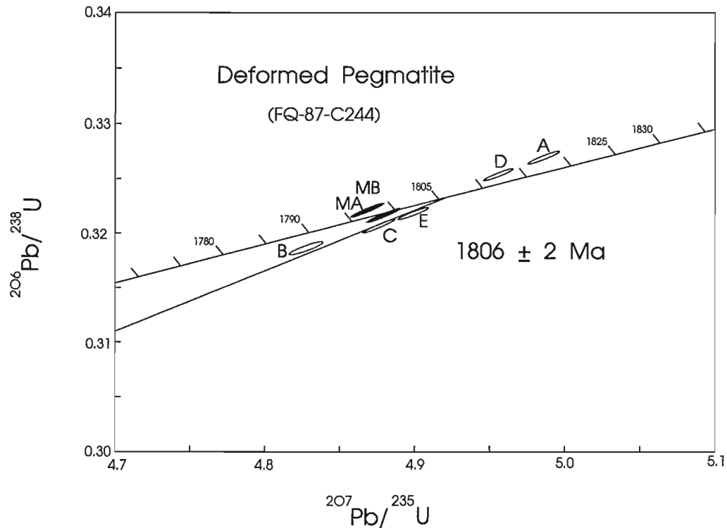
Figure 11. Concordia diagram showing U-Pb results from the deformed pegmatite (FQ-87-C244).
