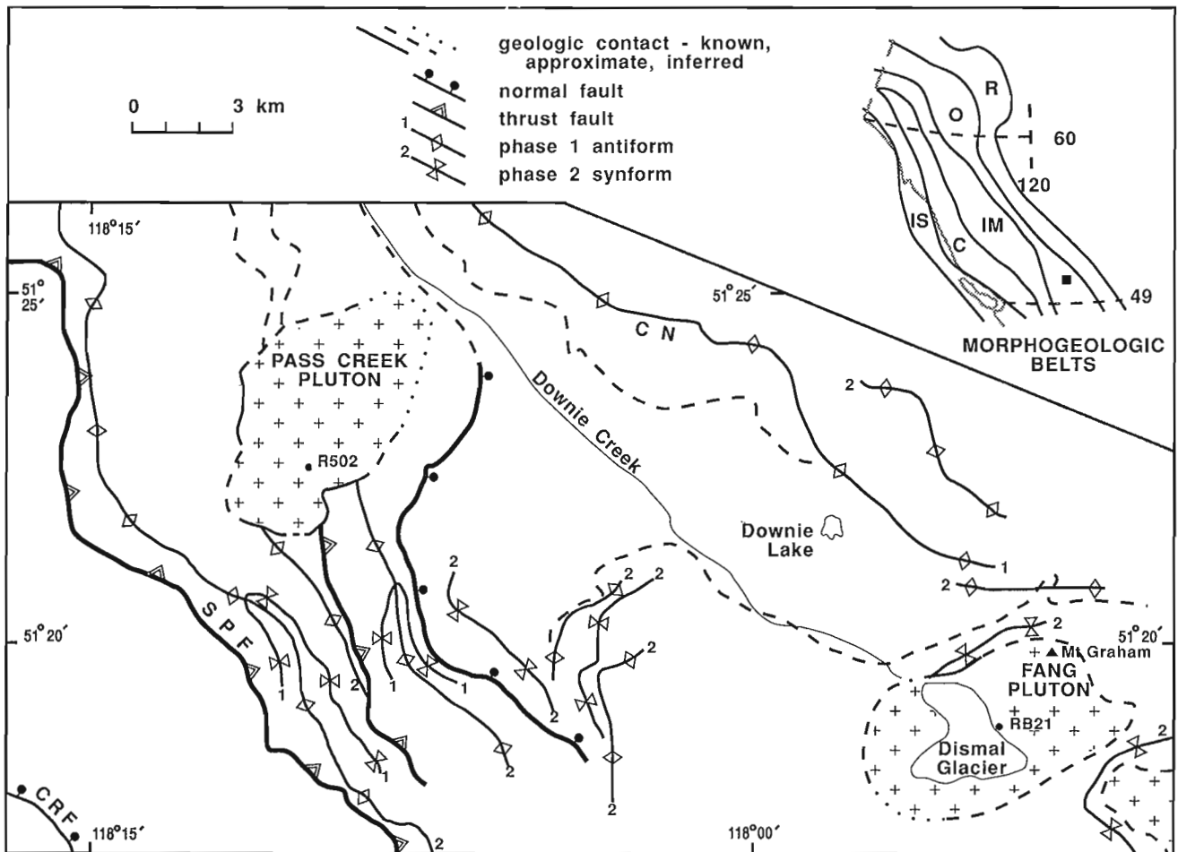
Figure 1. Location and geological setting of Pass Creek and Fang plutons. Black square in insert of Morphological Belts of the Canadian Cordillera locates the area. R – Rocky Mountain Belt, O – Omineca Belt, IM – Intermontane Belt, C – Coast Belt, IS – Insular Belt. CRF – Columbia River Fault, SPF – Standard Peak Fault, CN – Carnes Nappe. Plutons (+) are intrusive into greenschist grade Lower Paleozoic rocks of the Hamill Group, Badshot Formation, and Lardeau Group (unpatterned). Map is simplified from Brown (1991), Wheeler (1963), and unpublished data (RLB). See text for further explanation.
