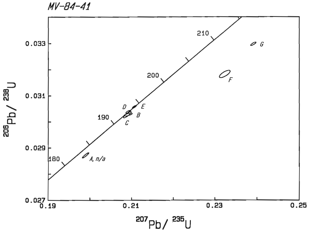
Figure 4a. U-Pb concordia plot of all of the data from sample MV-84-41, the Bromley Pluton. Error ellipses reflect the 2\sigma uncertainty.
