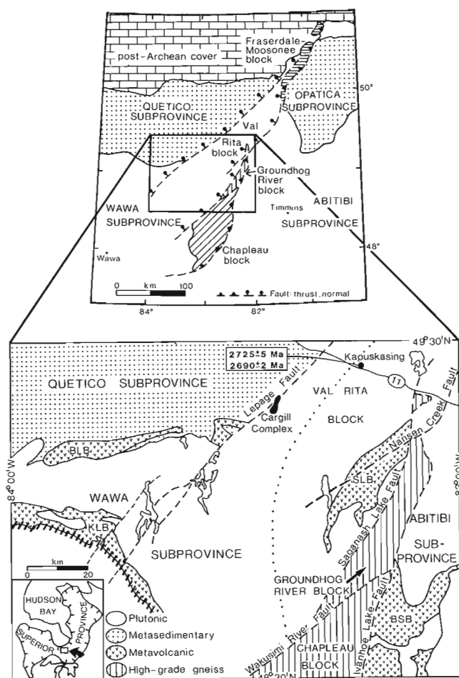
Figure 1. Generalized geological map of the Kapuskasing area showing distribution of belt-like subprovinces and major structural elements of the central Superior Province (after Card and Ciesielski, 1986; Percival and McGrath, 1986). Top map and inset show the location of the Kapuskasing area in the Superior Province. The location of the dated sample and the resulting ages are shown. The Kapuskasing uplift includes the Chapleau, Groundhog River, Fraserdale-Moosonee, and Val Rita blocks. Heavy diagonal dashes represent approximate extent of the Puskuta Lake shear zone. Dotted line is the axis of arcuate gravity and aeromagnetic anomalies of the Val Rita block. Metavolcanic belts are: BSB, Belford-Strachan belt; SLB, Saganash Lake belt; KLB, Kabinakagami Lake belt; BLB, Buchanan Lake belt.
