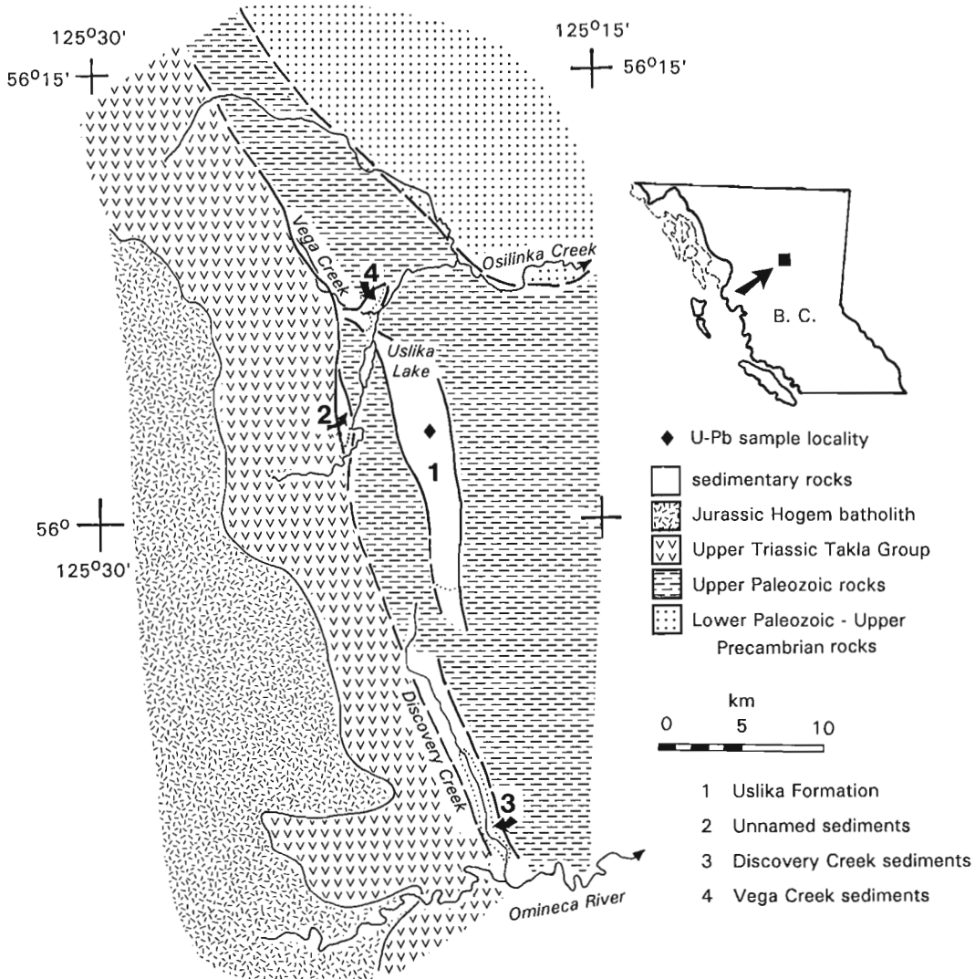
Figure 1. Geological map of the vicinity of Uslika Lake, north-central British Columbia, showing features discussed in the text and the locality of the dated boulder (after Roots, 1954 and Armstrong, 1949).
