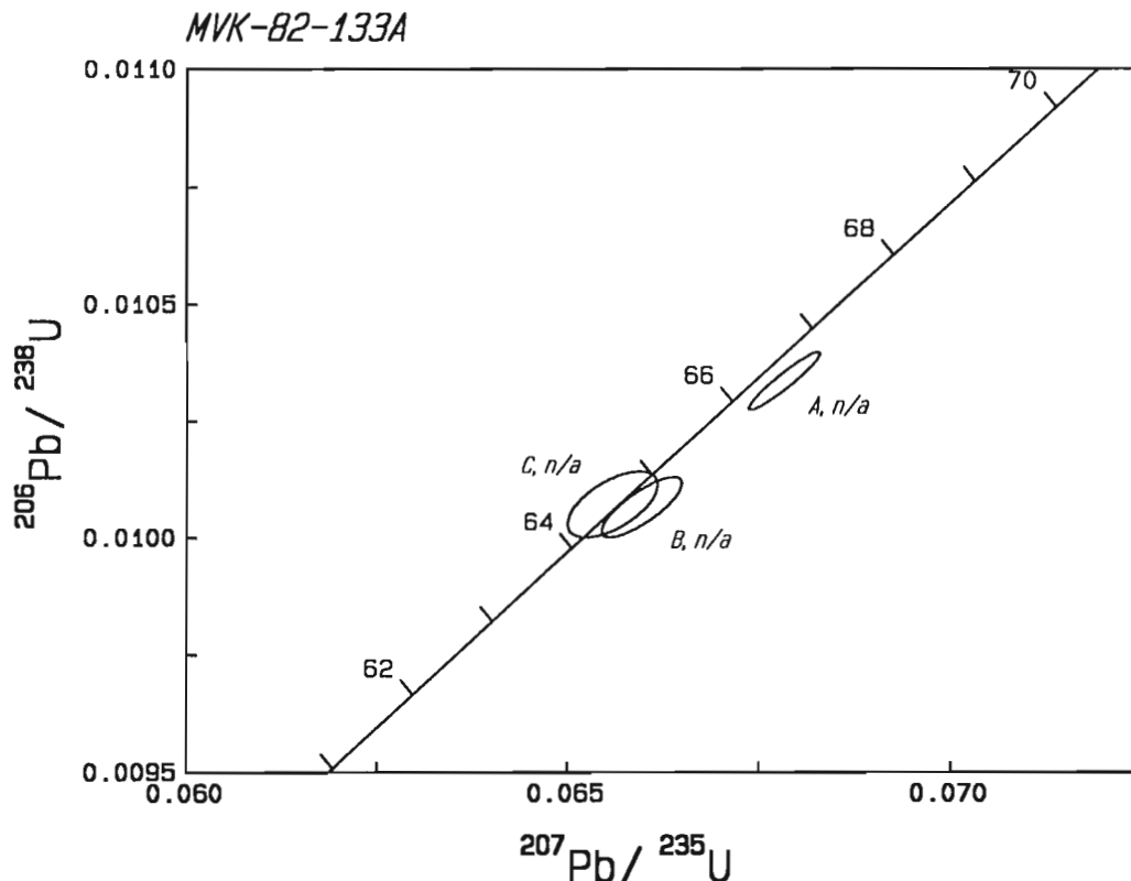
Figure 15. U-Pb concordia plot of MVK-82-133A, granodiorite of the Nicola Batholith. Error ellipses reflect the 2\sigma uncertainty.
