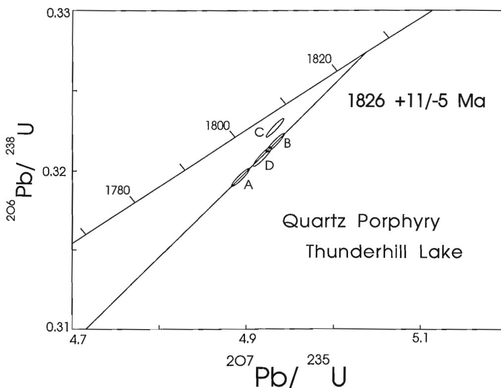
Figure 2. U-Pb concordia plot of zircon from the quartz porphyry.
