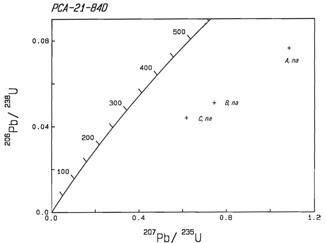
Figure 17. U-Pb concordia diagram for zircon from sample 15, PCA-21-84D.
