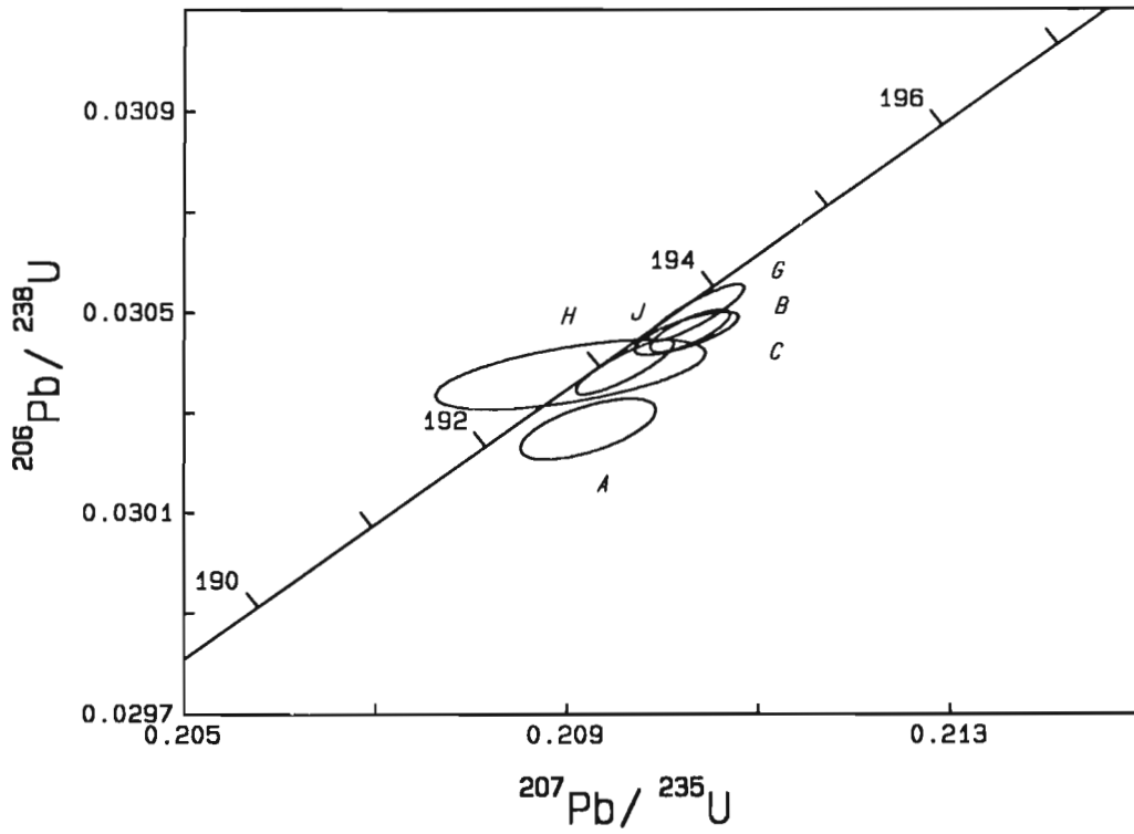
Figure 2. U-Pb concordia diagram for zircon from sample 1, PCA-64-85.
