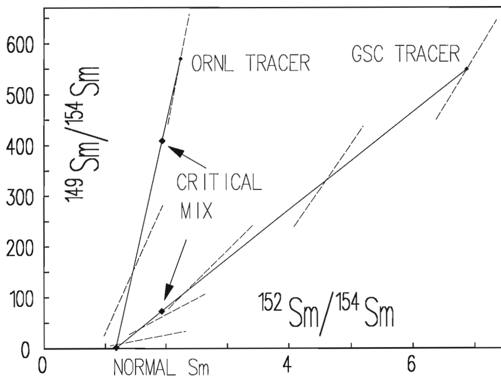
Figure 2. Mixing and fractionation relationships for normal Sm and two ^{149}\text{Sm} tracers. See Figure 1 caption for details.
