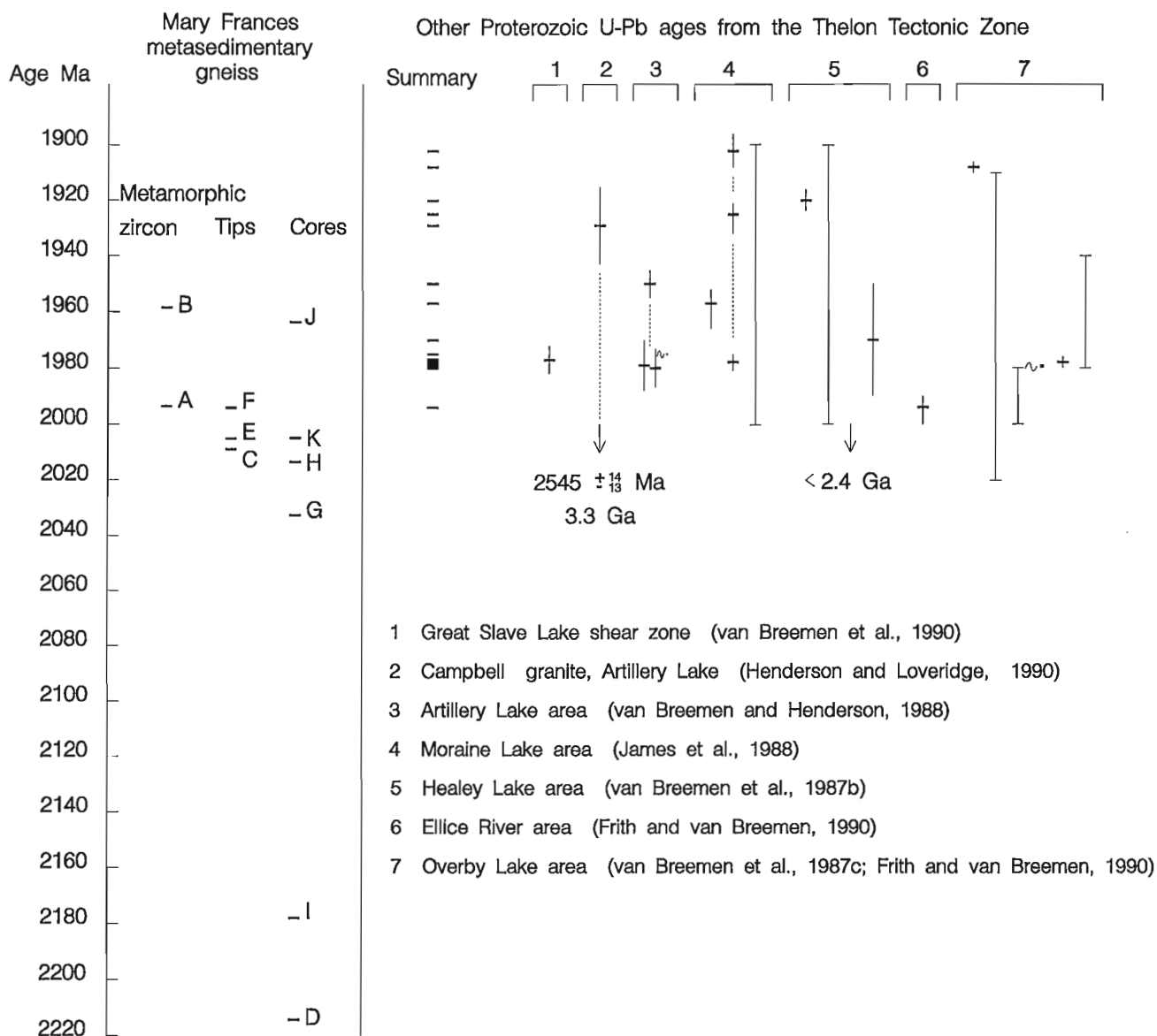
Figure 4. Summary of Mary Frances metasedimentary gneiss ^{207}\text{Pb} - ^{206}\text{Pb} ages shown in context with all other Proterozoic U-Pb ages from the Thelon Tectonic Zone or equivalents. Ages to date for the Thelon Tectonic Zone as a whole range between 1.90 Ga and 2.02 Ga with a concentration at about 1.98 Ga which may represent a major metamorphic event. Mary Frances metasedimentary gneiss zircon fractions interpreted as metamorphic in origin (metamorphic zircon and tips) range between 1.96 and 2.01 Ga in age; with one exception, somewhat older than the concentration at 1.98 Ga for the Thelon Tectonic Zone as a whole. The ages of 'core' fractions range between 1.96 Ga and 2.21 Ga but only two are significantly older than the metamorphic age range within the same rock. For the other Thelon Tectonic Zone ages, each entry represents a sample analyzed. In some samples, several ages, each with a vertical error bar, were separated (ie, cores and rims). These are joined by a dotted line. For some others, only a range is indicated.
