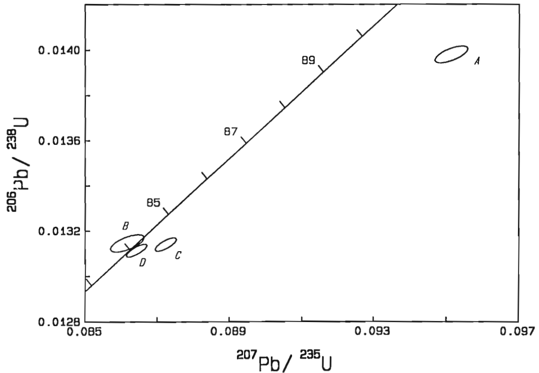
Figure 12. U-Pb concordia plot of MV-86-431, biotite quartz-monzonite of the Scuzzy Pluton. Error ellipses reflect the 2\sigma uncertainty.
