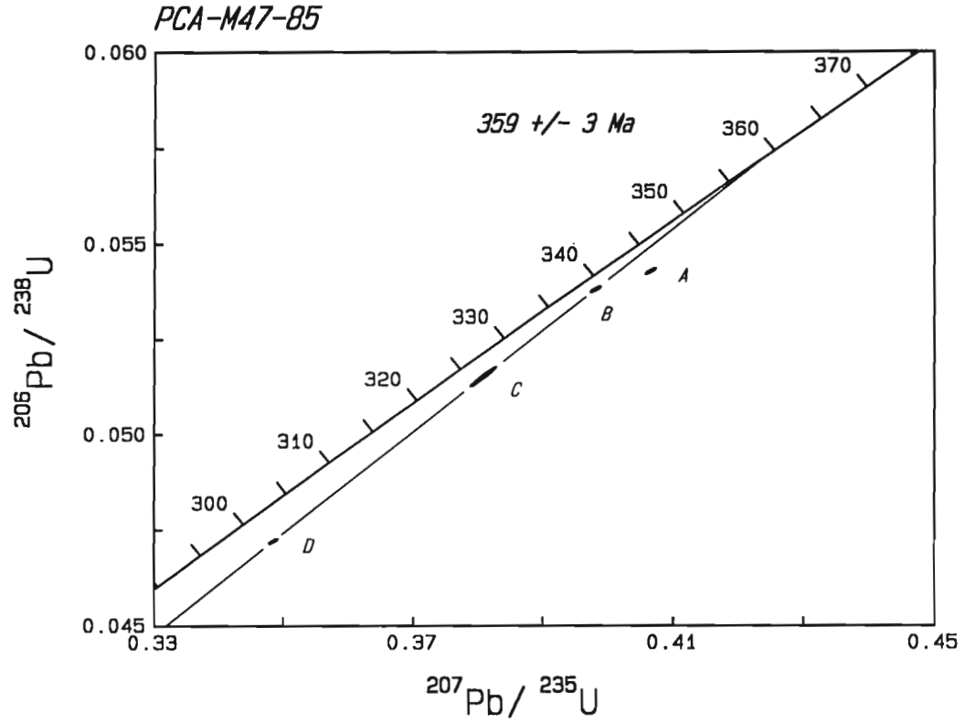
Figure 6. Concordia diagram for zircon U-Pb data from sample PCA-M47-85. Error ellipses reflect 2\sigma uncertainty.
