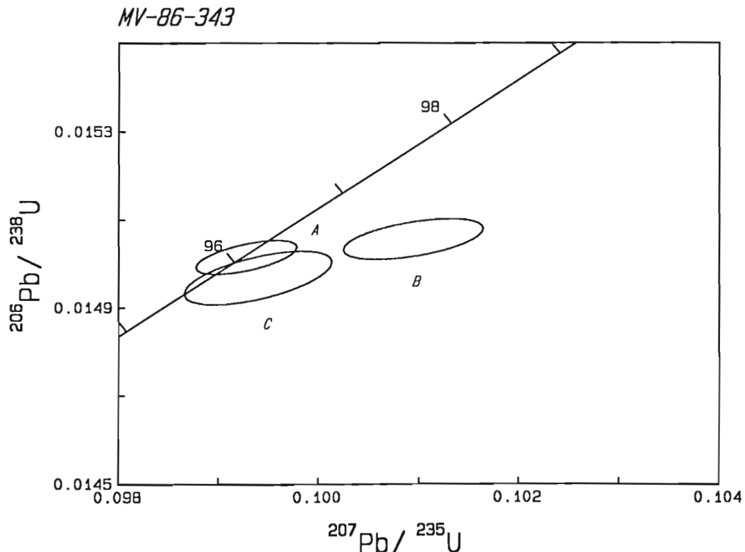
Figure 10. U-Pb concordia plot of MV-86-343, mafic Breakenridge gneiss. Error ellipses reflect the 2\sigma uncertainty.
