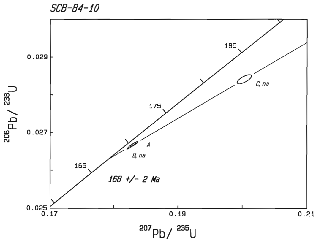
Figure 6. U-Pb concordia diagram for the Ste Marie Pluton, sample SCB-84-10. Error ellipses reflect 2\sigma uncertainty.
