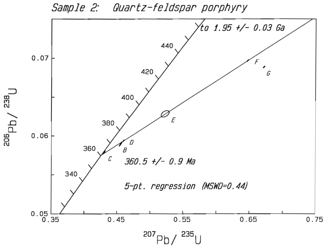
Figure 3b. U-Pb concordia plot for sample 2 (quartz-feldspar porphyry). Error ellipses are shown at 2\sigma level.
