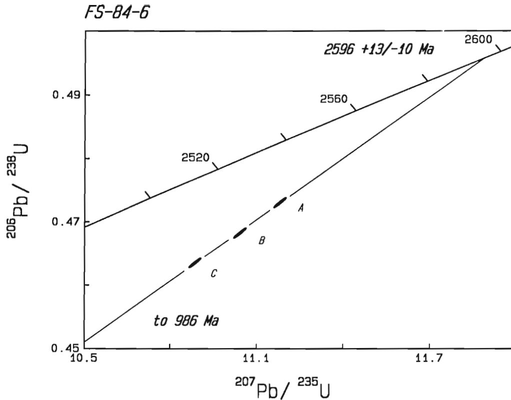
Figure 2. U-Pb concordia diagram for sample FS-84-6. Error ellipses are 2\sigma .
