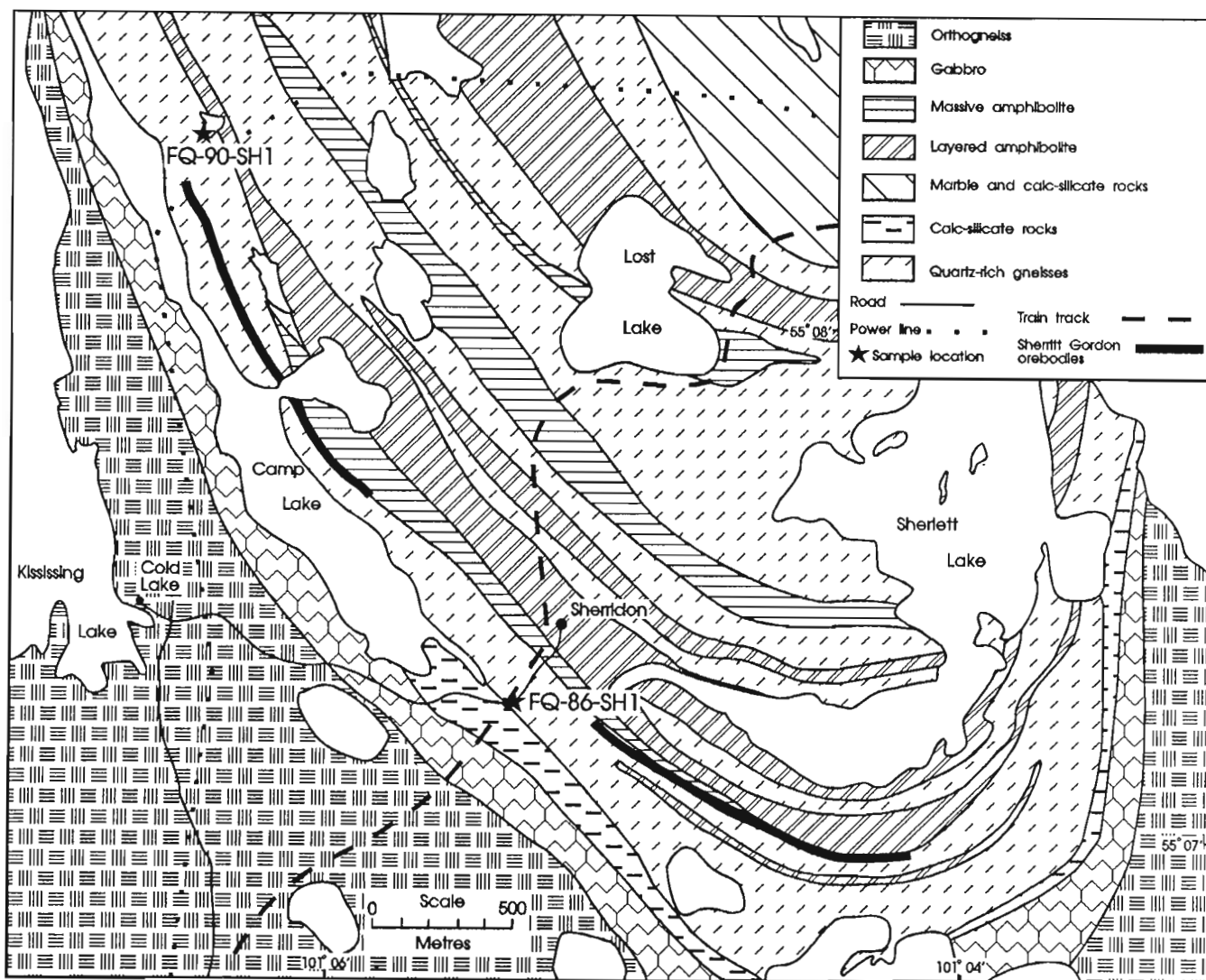
Figure 6. Simplified geological map showing sample locations in the Sherridon area.
