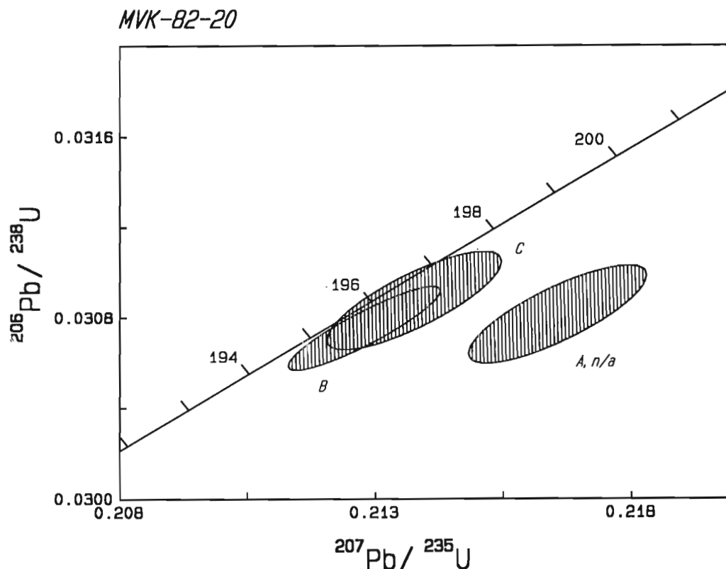
Figure 3. U-Pb concordia plot of MVK-82-20, granodiorite of the Wild Horse Batholith. Error ellipses reflect the 2\sigma uncertainty.
