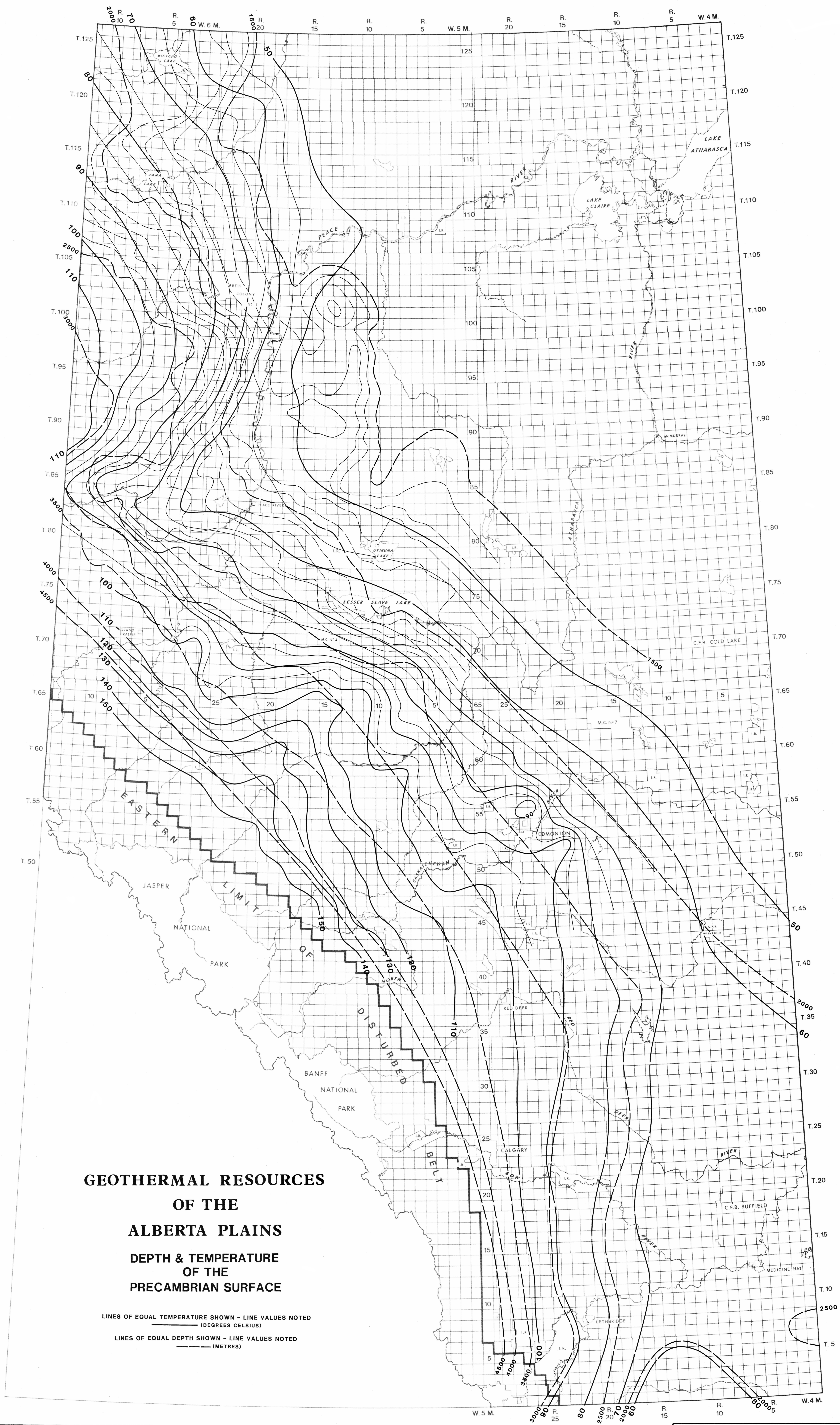
FIGURE 22 DEPTH & TEMPERATURE OF THE PRECAMBRIAN SURFACE
