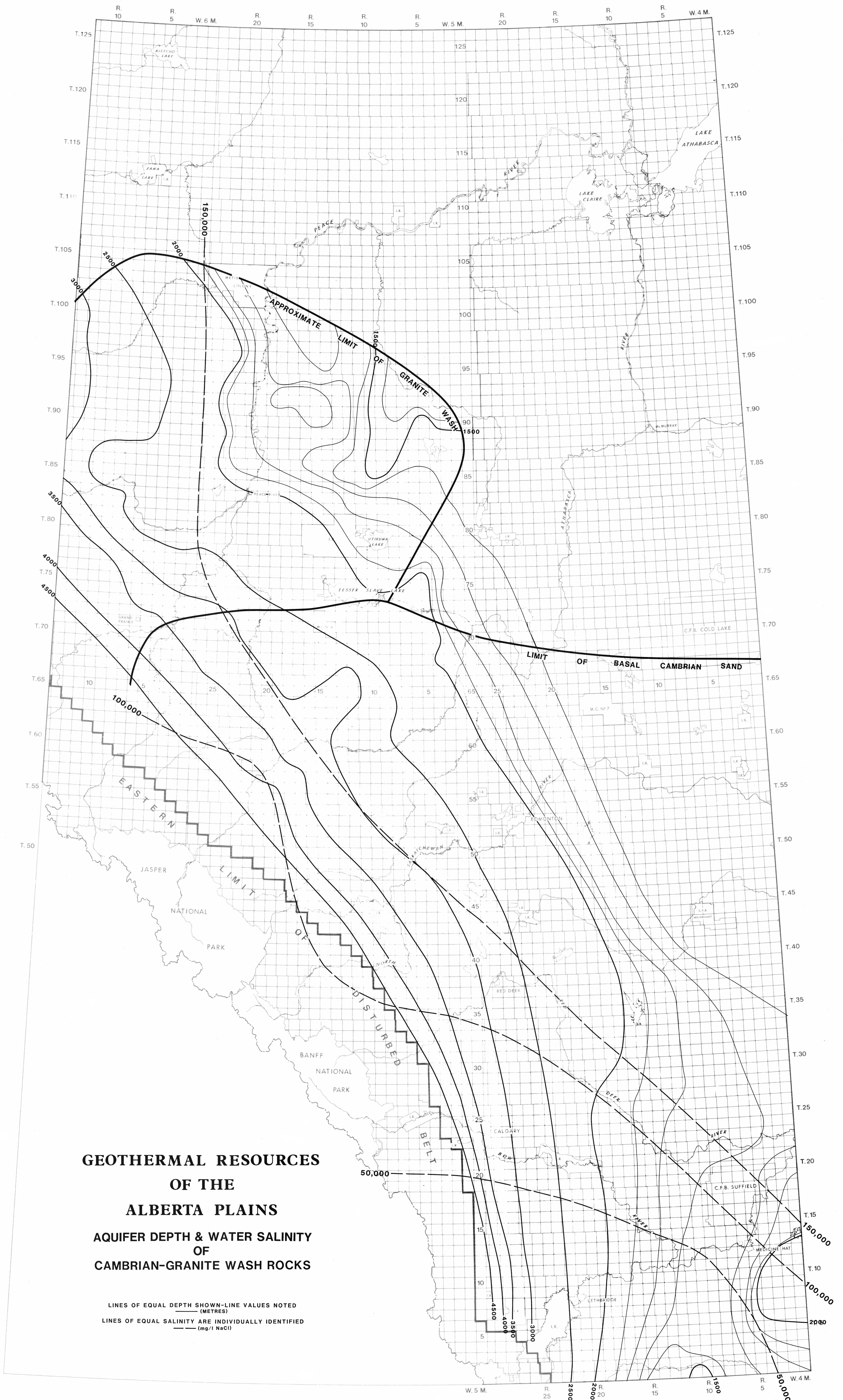
FIGURE 21 AQUIFER DEPTH & WATER SALINITY OF CAMBRIAN-GRANITE WASH ROCKS
