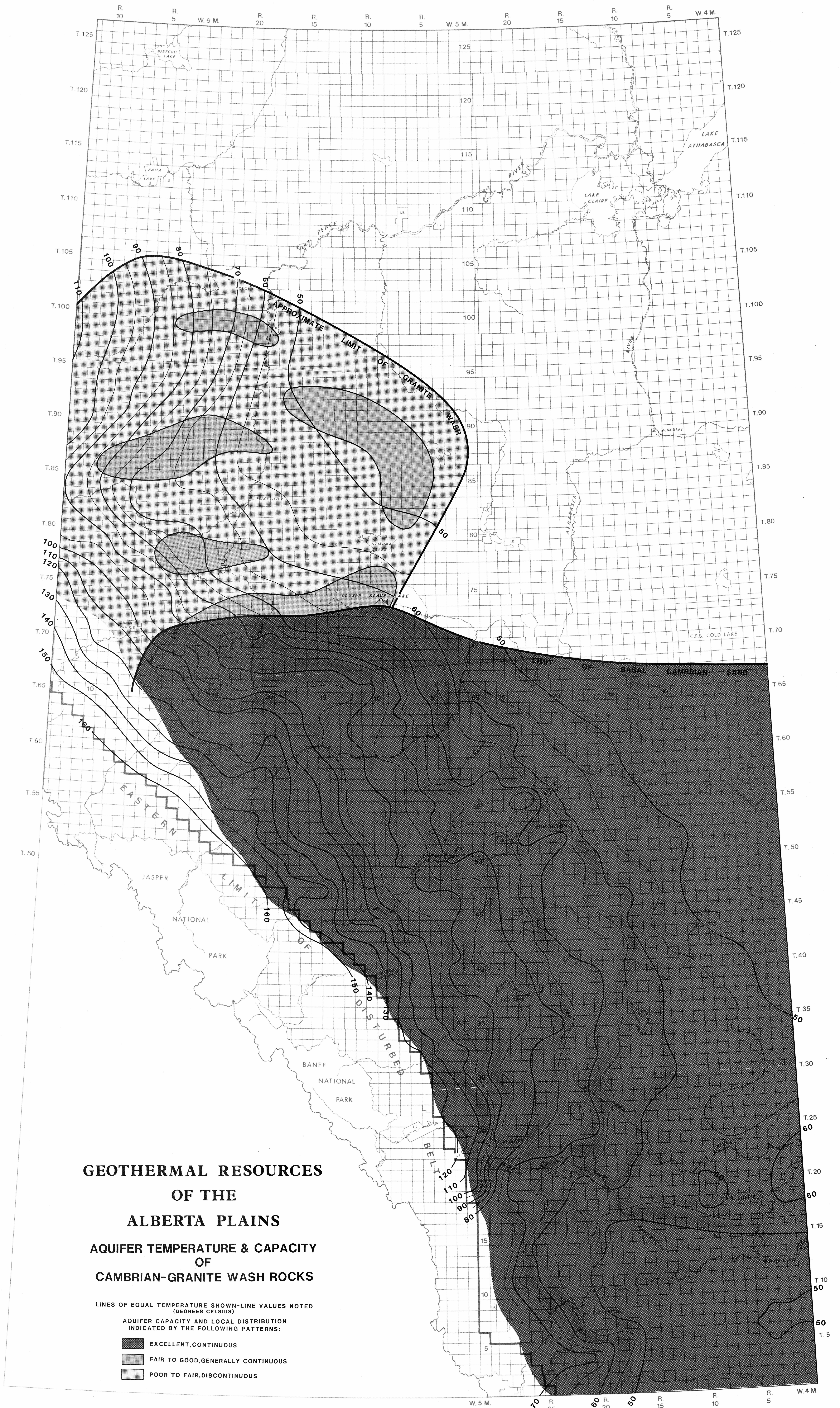
FIGURE 20 AQUIFER TEMPERATURE & CAPACITY OF CAMBRIAN-GRANITE WASH ROCKS
