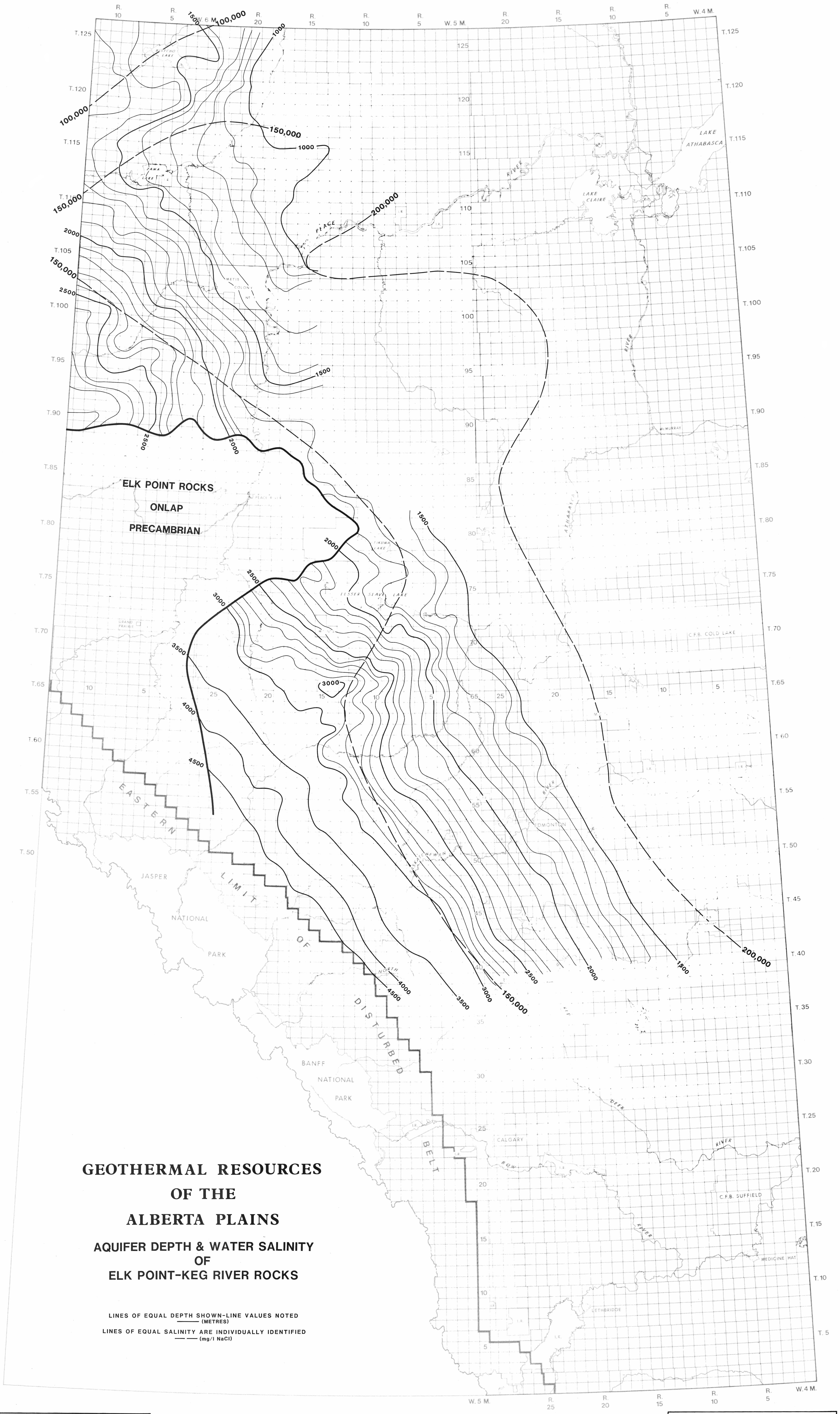
FIGURE 19 AQUIFER DEPTH & WATER SALINITY OF ELK POINT-KEG RIVER ROCKS
