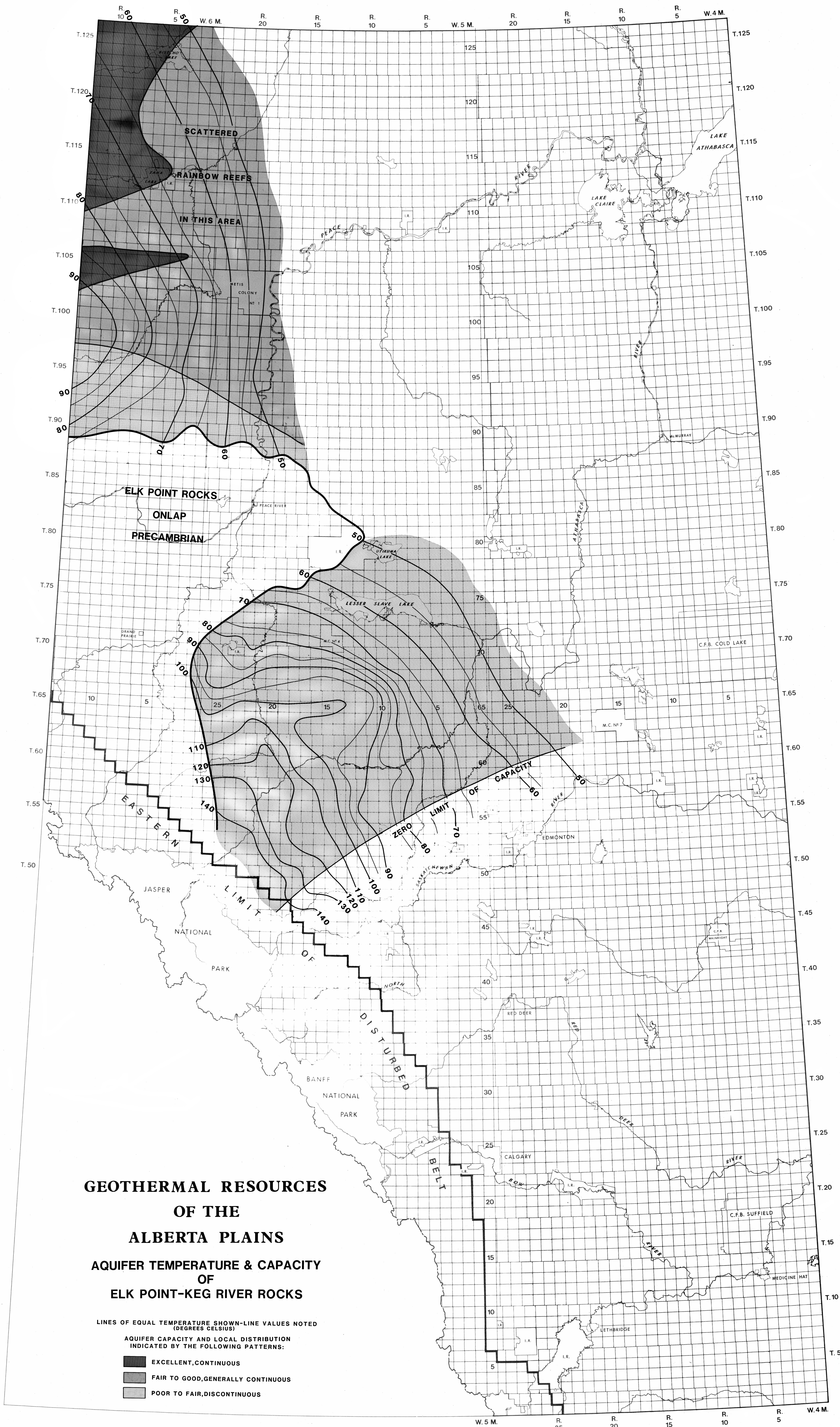
FIGURE 18 AQUIFER TEMPERATURE & CAPACITY OF ELK POINT-KEG RIVER ROCKS
