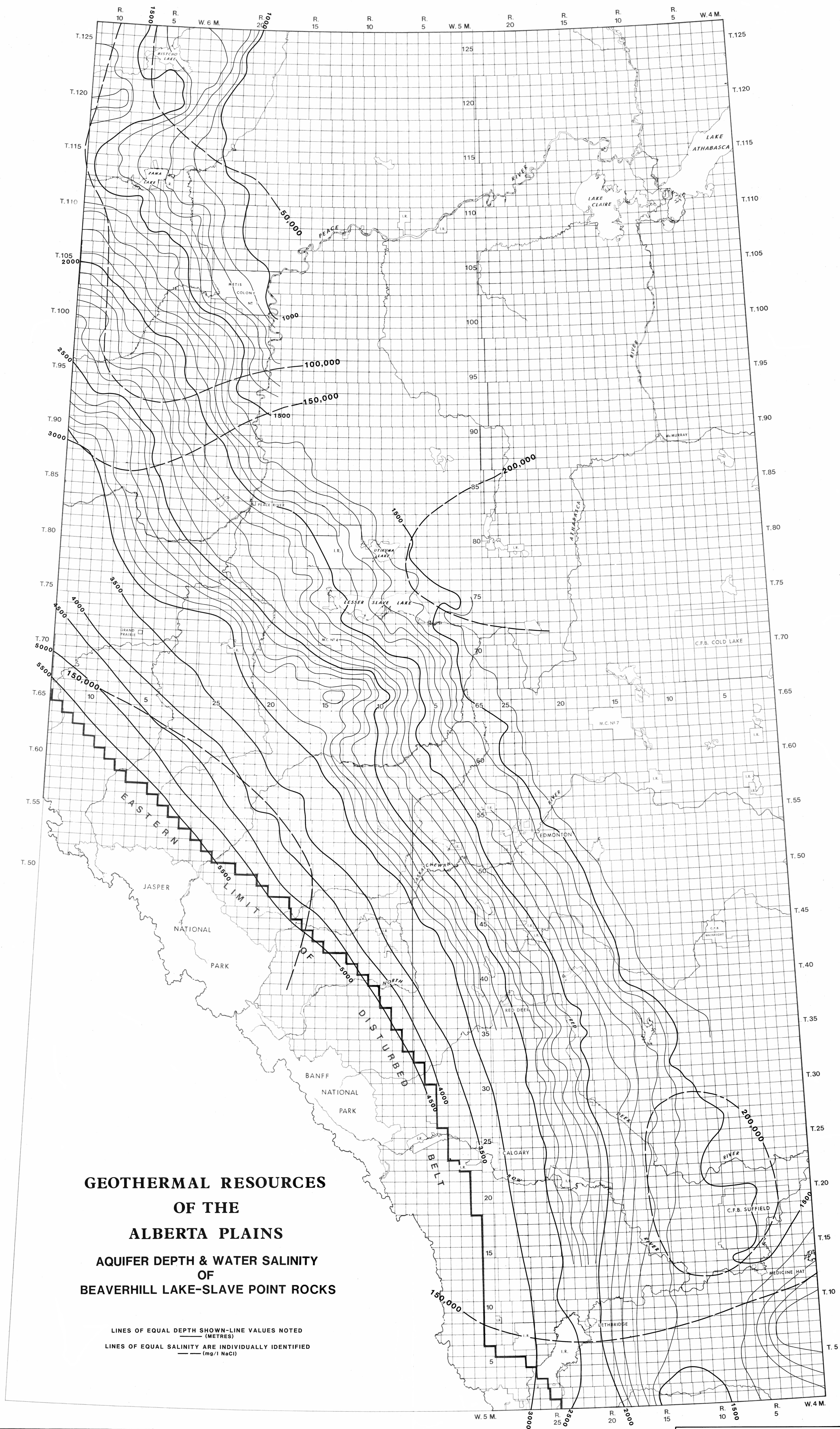
FIGURE 17 AQUIFER DEPTH & WATER SALINITY OF BEAVERHILL LAKE-SLAVE POINT ROCKS
