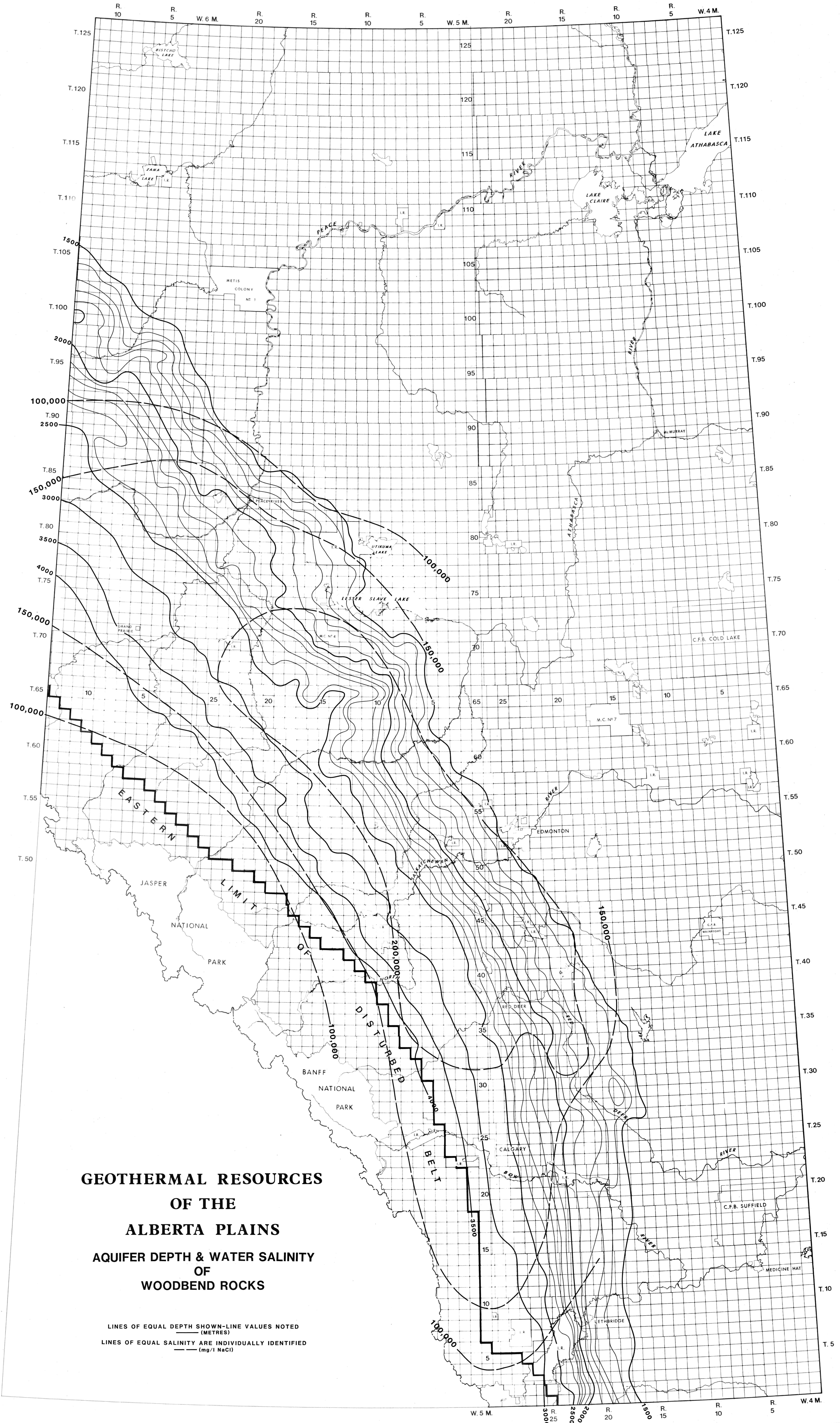
FIGURE 15 AQUIFER DEPTH & WATER SALINITY OF WOODBEND ROCKS
