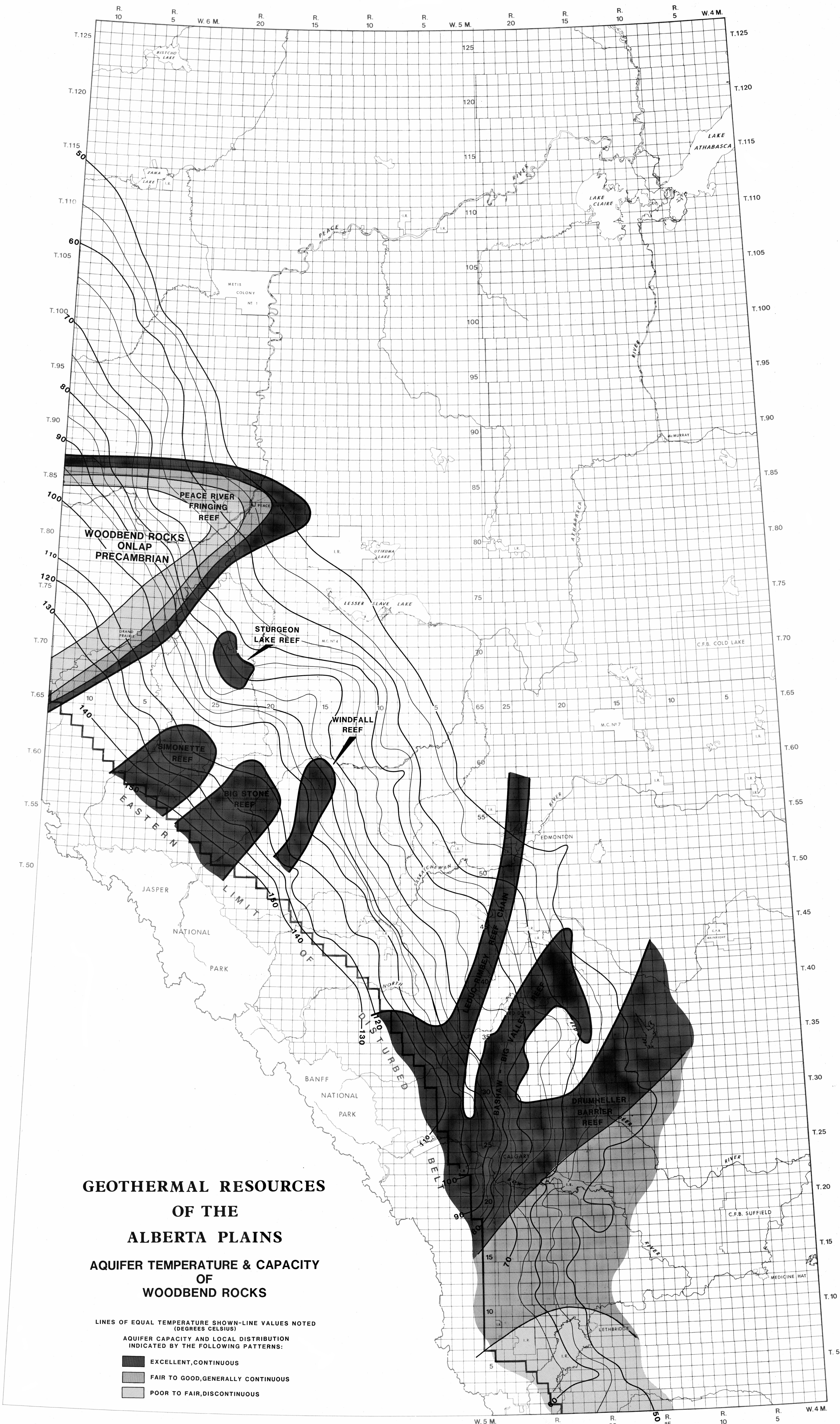
FIGURE 14 AQUIFER TEMPERATURE & CAPACITY OF WOODBEND ROCKS
