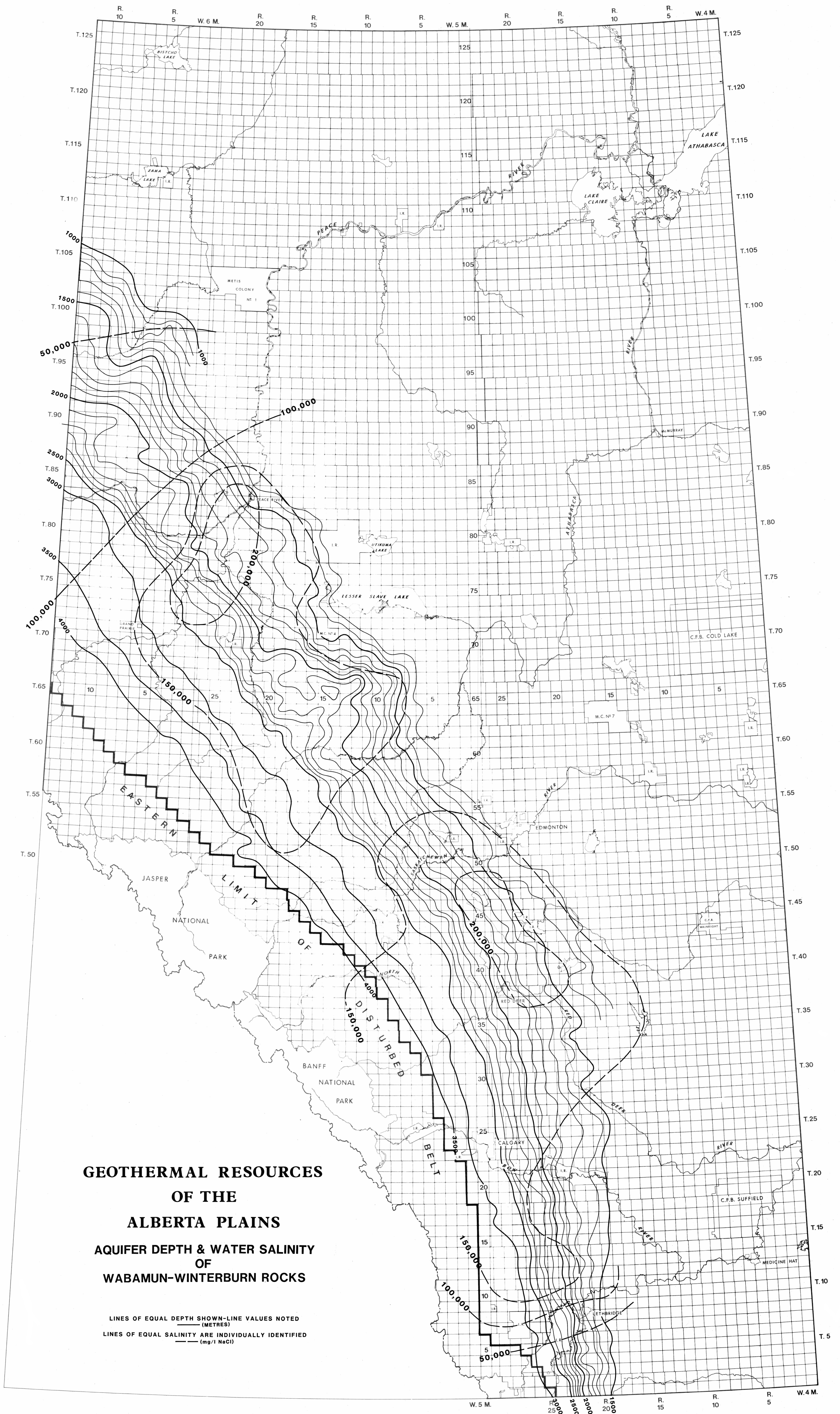
FIGURE 13 AQUIFER DEPTH & WATER SALINITY OF WABAMUN-WINTERBURN ROCKS
