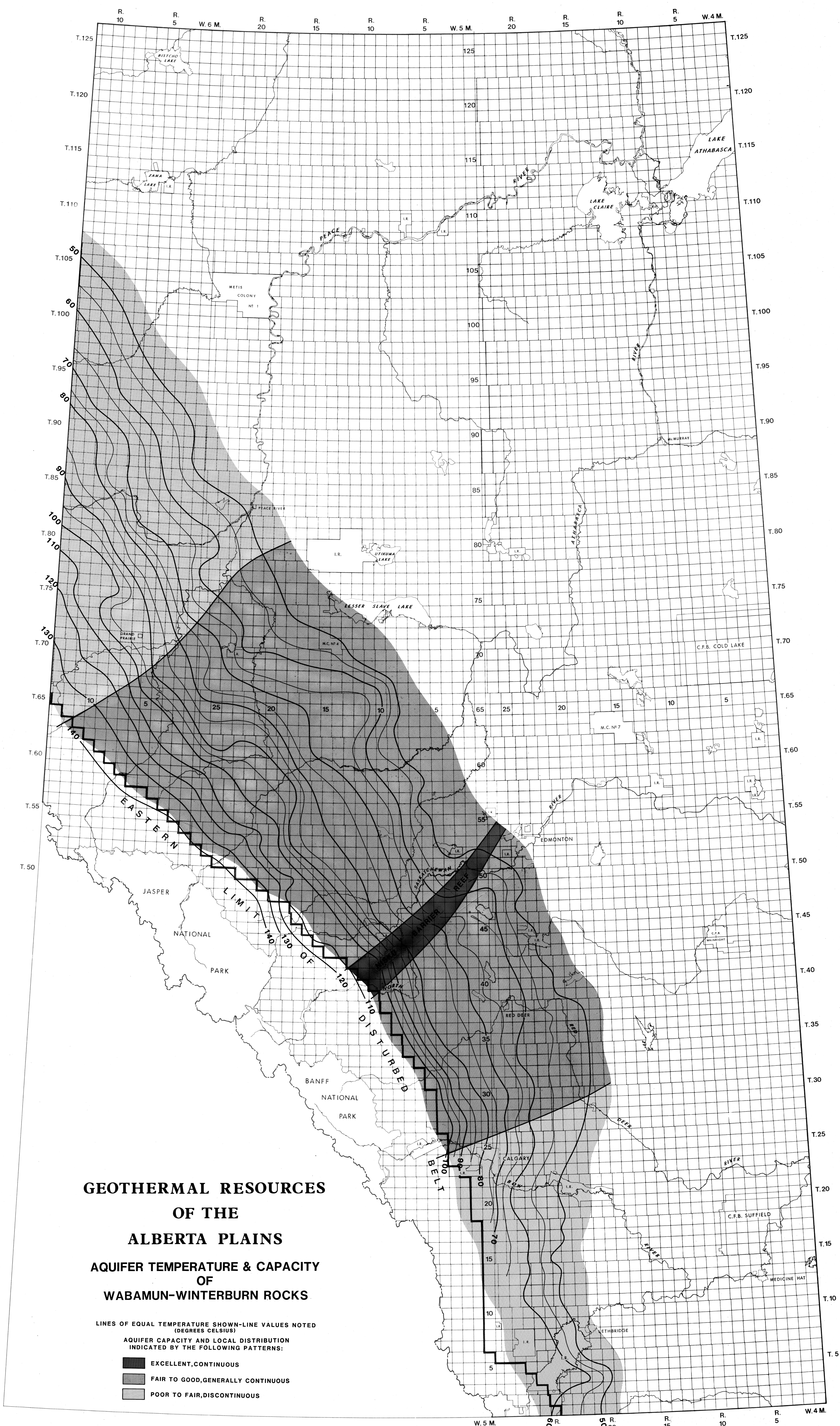
FIGURE 12 AQUIFER TEMPERATURE & CAPACITY OF WABAMUN-WINTERBURN ROCKS
