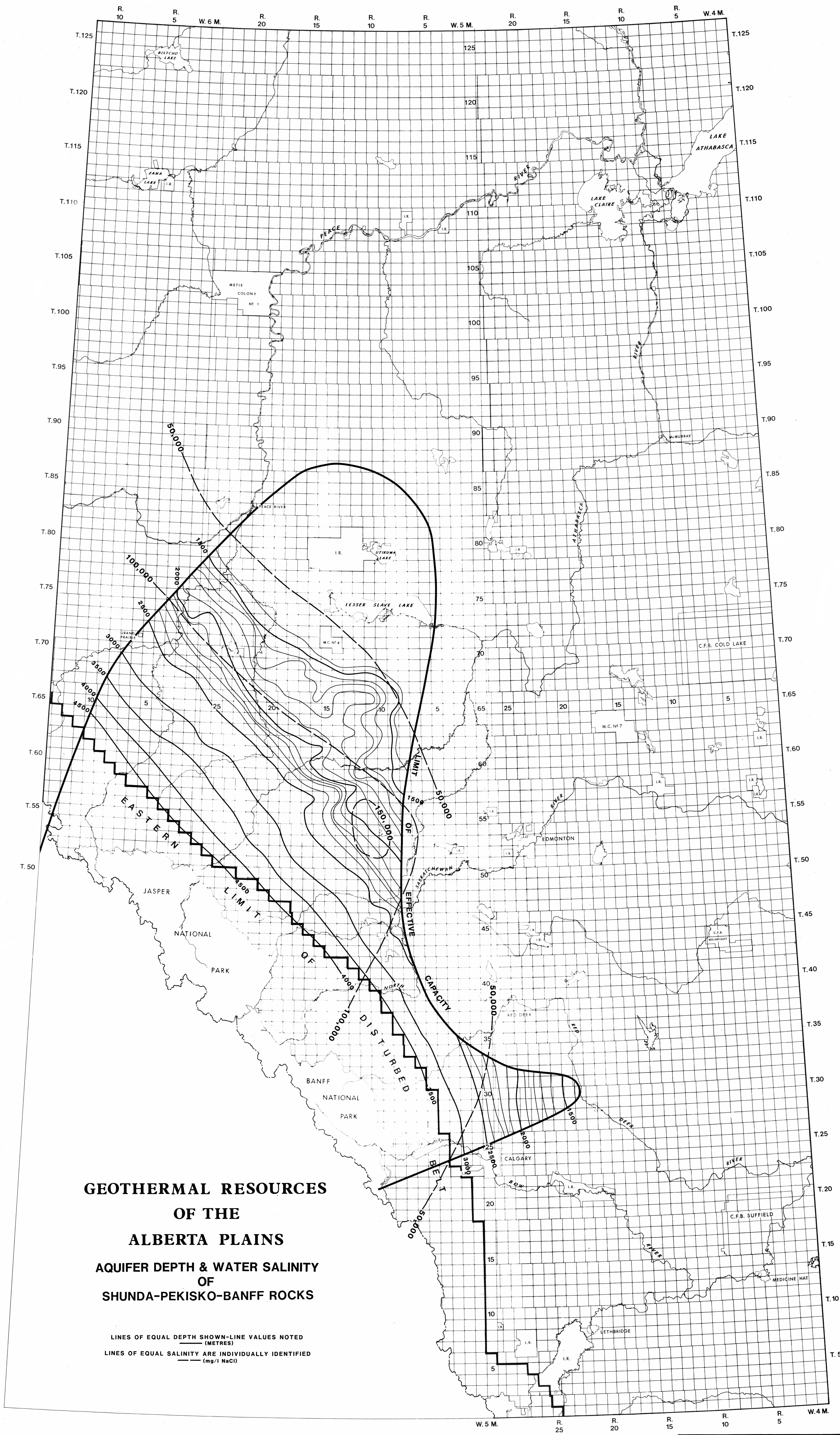
FIGURE 11 AQUIFER DEPTH & WATER SALINITY OF SHUNDA-PEKISKO-BANFF ROCKS
