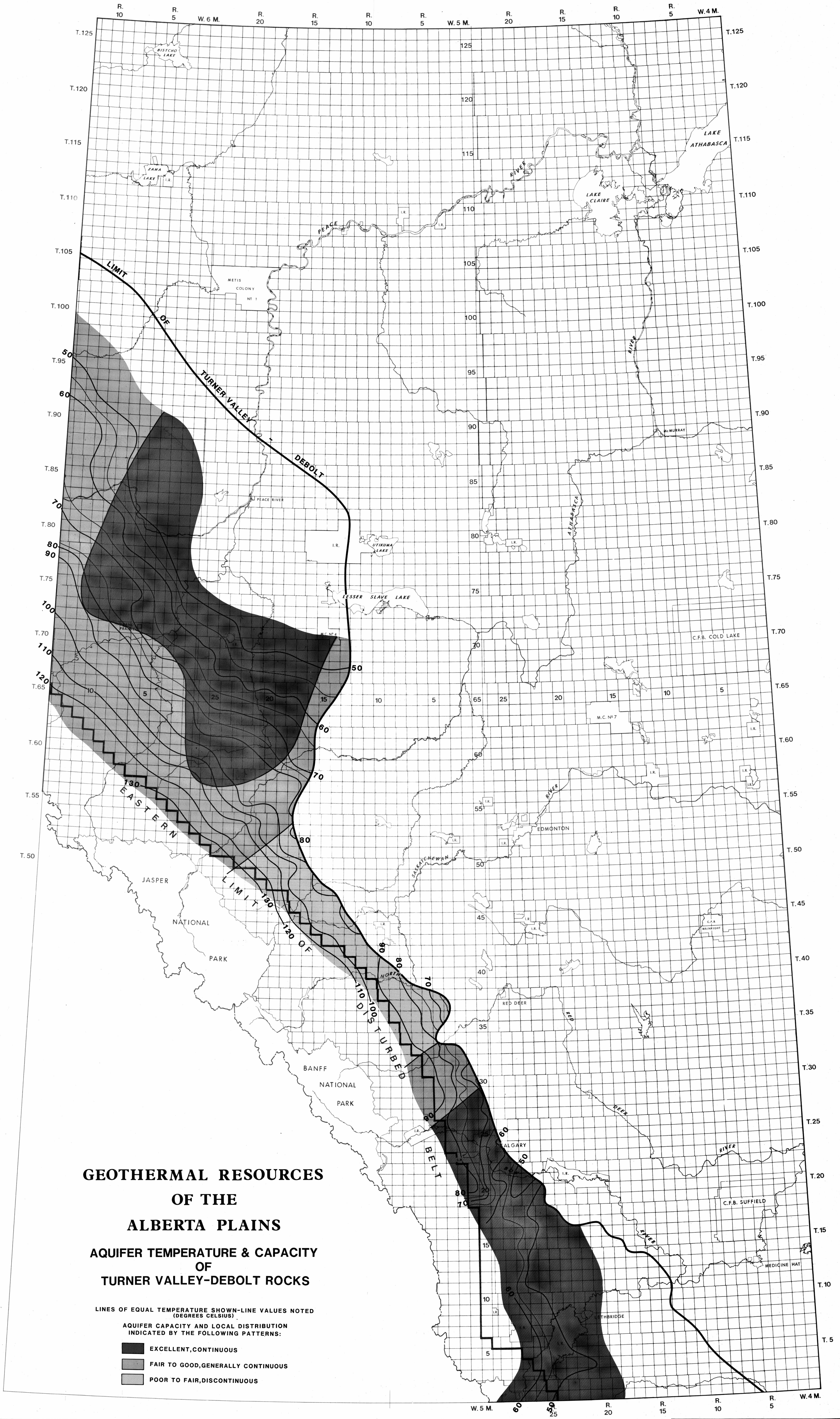
FIGURE 8 AQUIFER TEMPERATURE & CAPACITY OF TURNER VALLEY-DEBOLT ROCKS
