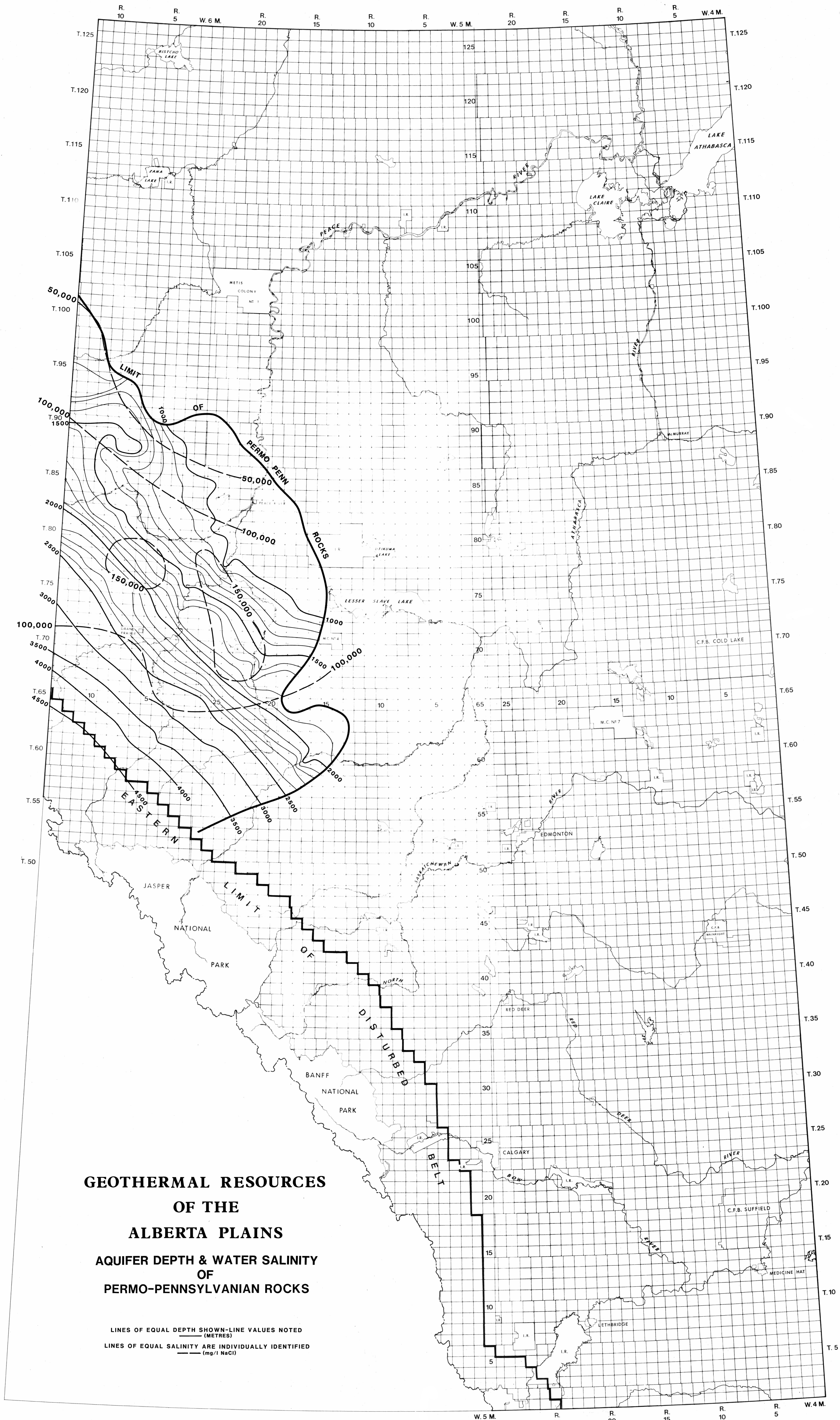
FIGURE 7 AQUIFER DEPTH & WATER SALINITY OF PERMO-PENNSYLVANIAN ROCKS
