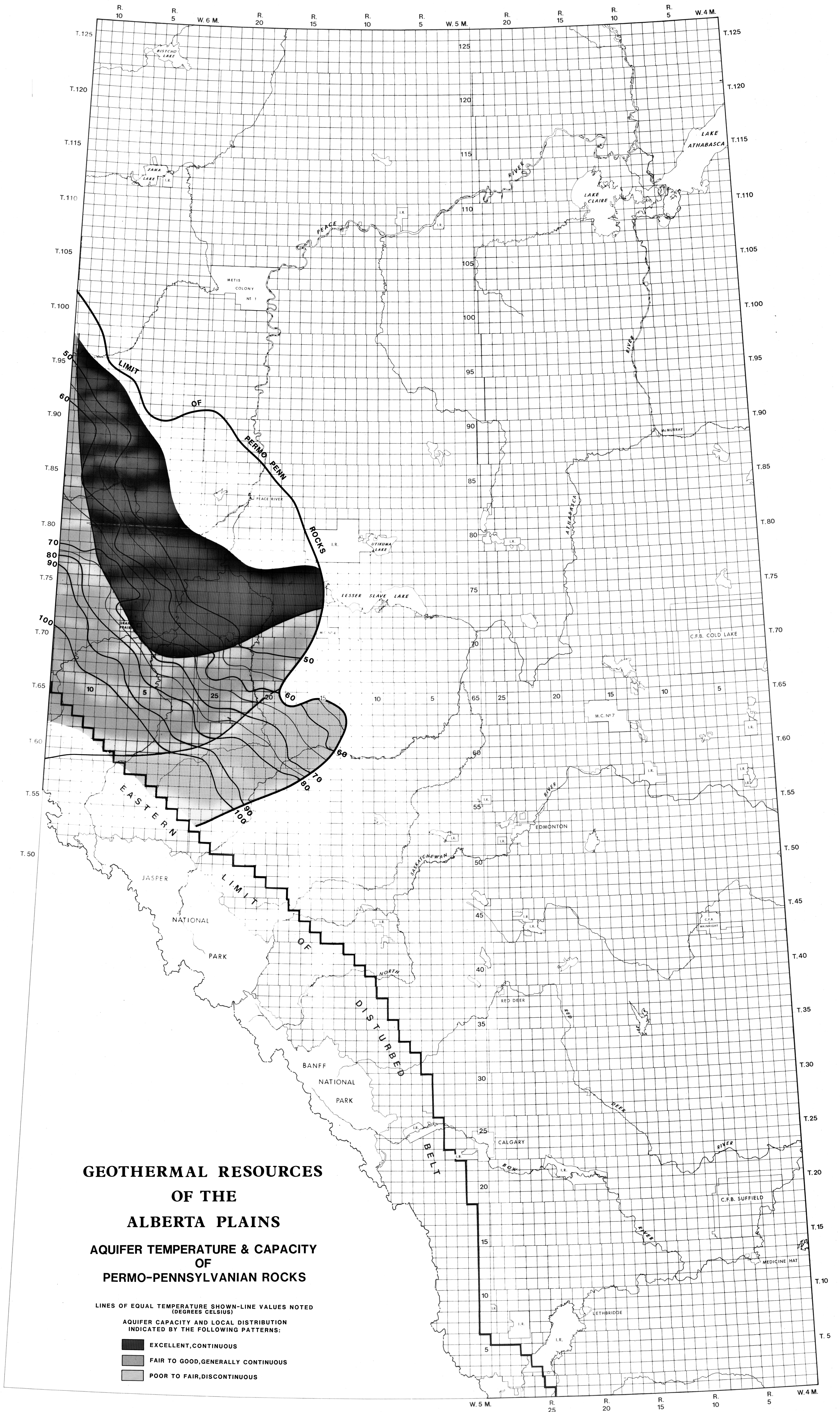
FIGURE 6 AQUIFER TEMPERATURE & CAPACITY OF PERMO-PENNSYLVANIAN ROCKS
