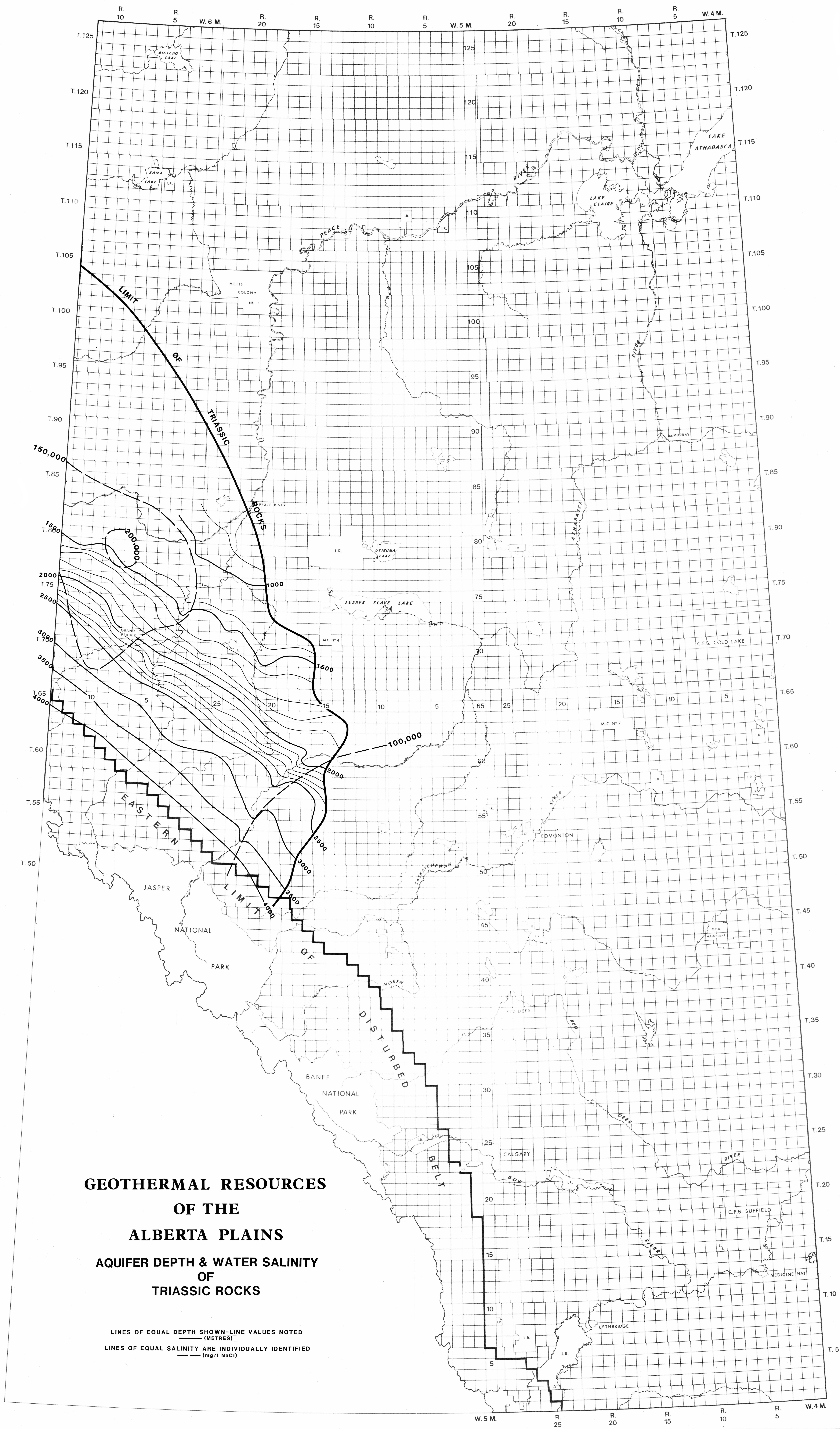
FIGURE 5 AQUIFER DEPTH & WATER SALINITY OF TRIASSIC ROCKS
