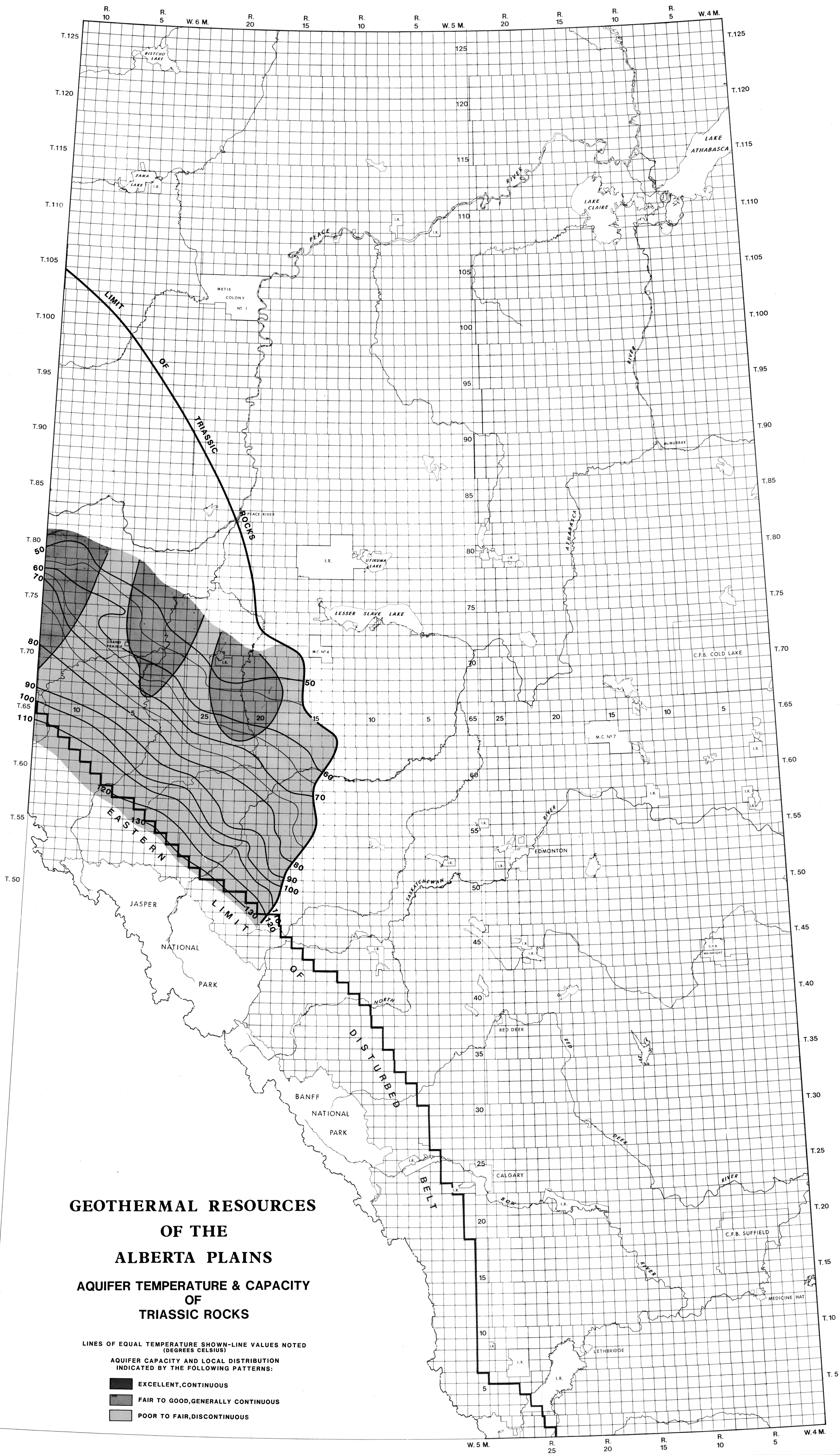
FIGURE 4 AQUIFER TEMPERATURE & CAPACITY OF TRIASSIC ROCKS
