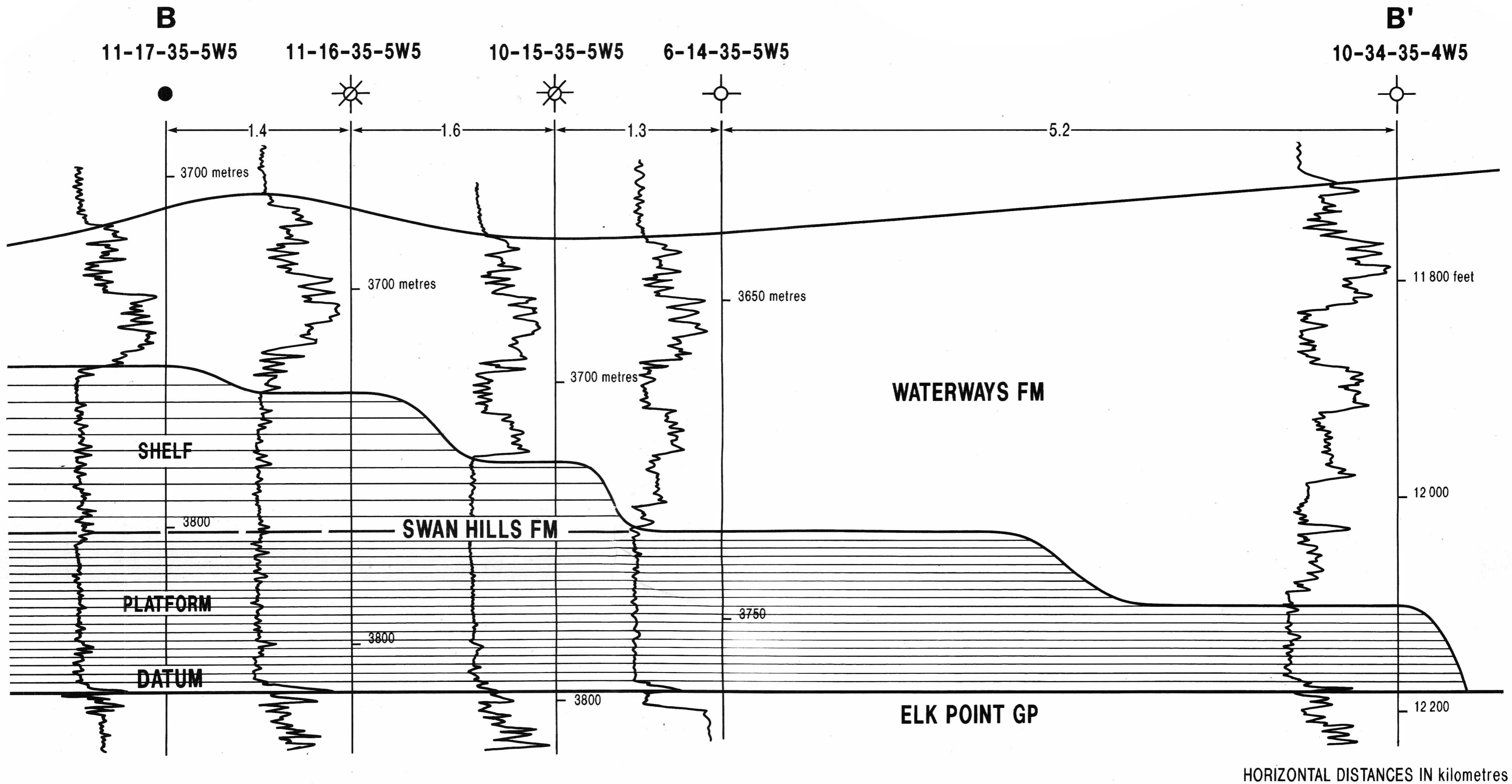
FIGURE 3 CROSS SECTION B - B' SWAN HILLS FORMATION
