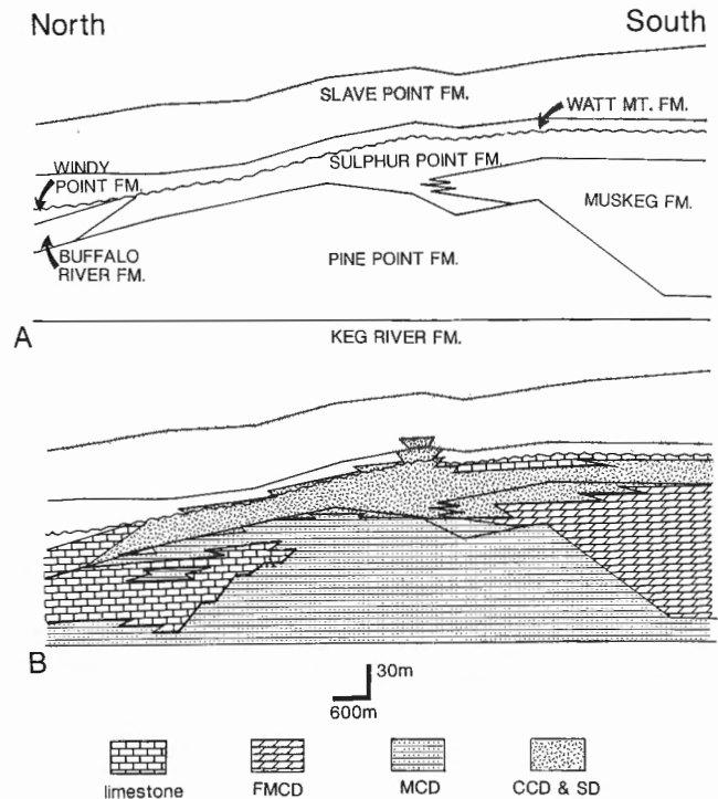
Figure 2. a) Stratigraphy of the Presqu'ile barrier in the western part of Pine Point property (600 m west of open pit N81, along -92 500 geodeparture). b) Spatial distribution of four types of dolomites.
