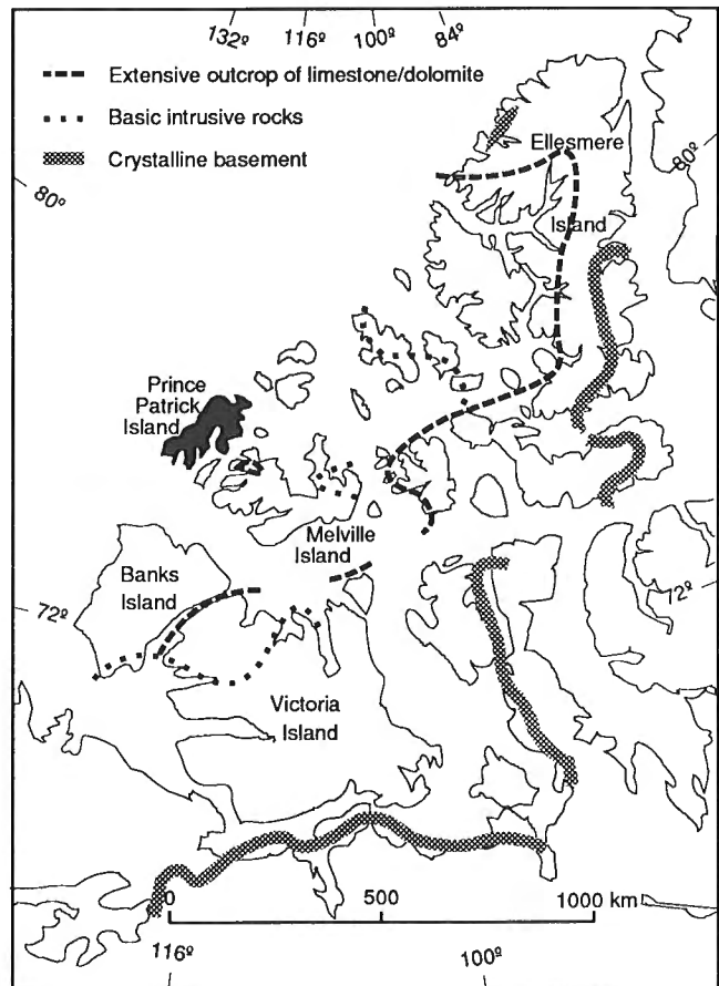
Figure 2. Sources of common erratics on Prince Patrick Island: northwesternmost limits.
