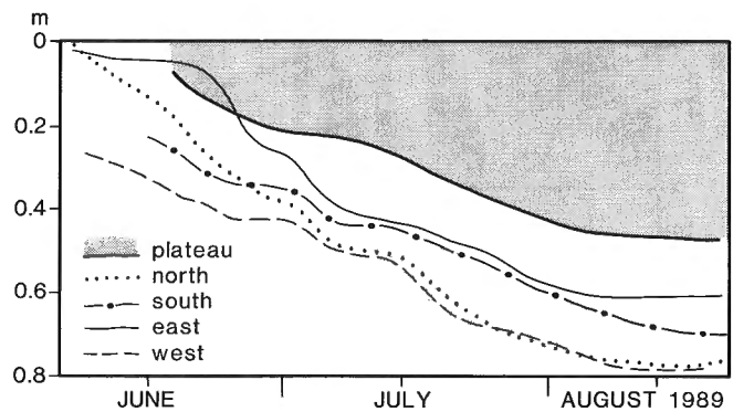
Figure 8. Comparison of frost table development at the middle of four slopes and on the plateau.
