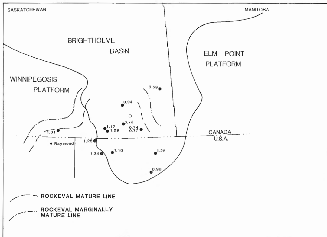
Figure 6. Geographic variation of C_{29} S/R sterane thermal maturity indicator for oils (closed circles). The figure also indicates the location of the Steelman well (open circle). Limits of fondofacies source rock thermal maturity and shelf edge from Figure 1.
