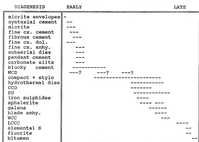
Figure 3. Diagenetic paragenesis of the Presqu'ile barrier (abbreviations: cx. = crystalline; dol. = dolomite; diss = dissolution; MCD = medium crystalline dolomite; compact = compaction; stylo = stylolization; CCD = coarse crystalline dolomite; SD = saddle dolomite; anhy. = anhydrite; WCC = white coarse crystalline calcite; LCCC = late stage coarse crystalline calcite).
