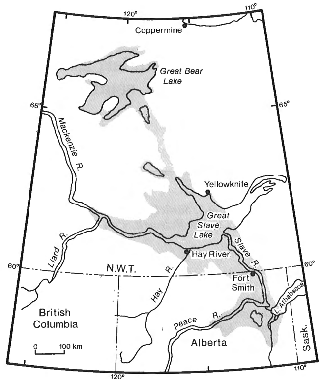
Figure 1. Glacial Lake McConnell (shaded) at its maximum extent, about 10 000 BP (modified from Craig, 1965).
