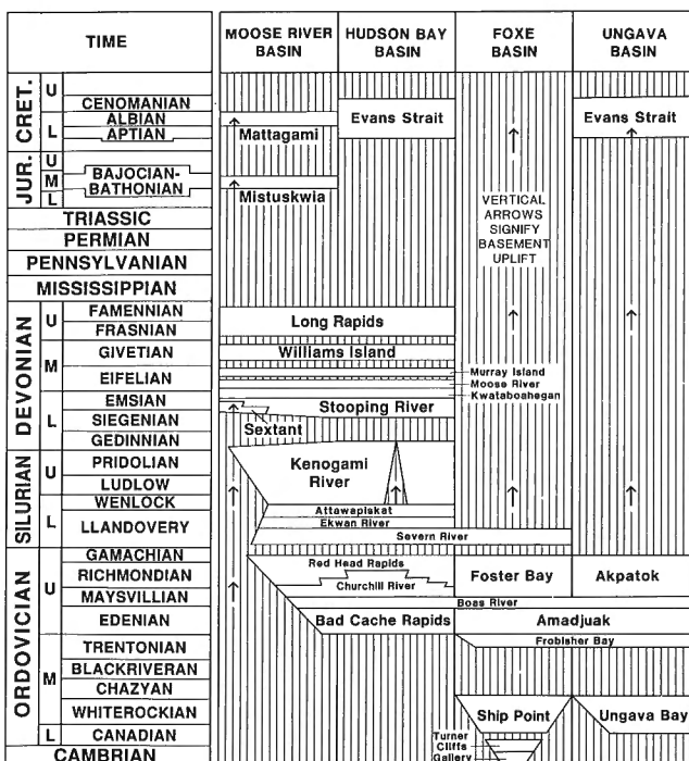
Figure 2. Time-stratigraphic framework of Paleozoic and Mesozoic sequences.
