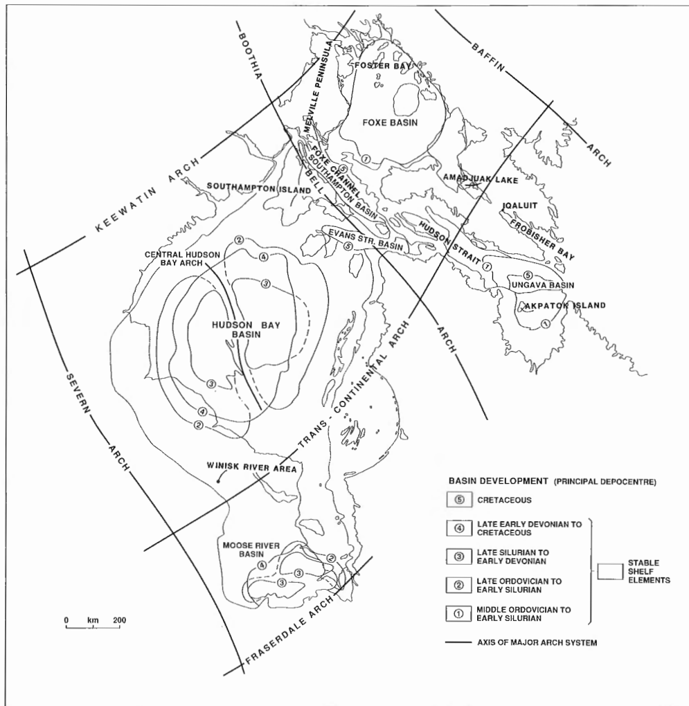
Figure 1. Index map of Hudson Platform showing tectonic elements and localities referred to in text.
