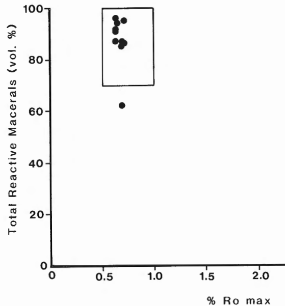
Figure 4. Predicted liquefaction potential of Coalspur coal based on maximum reflectance (Ro max) and total reactive macerals (mmf). (Modified from Davis et al., 1976.)
