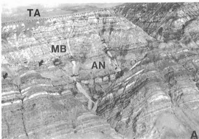
Figure 3. Exposures of the Mount Bayley Formation on west-central Ellesmere Island. A. Greely Fiord section. Upper Antoinette ( AN ), Mount Bayley ( MB ) and lower Tanquary ( TA ) formations are shown. Note dolostone (arrows) and evaporite (white bands) horizons within Antoinette Formation and carbonate horizons (dark bands) within Mount Bayley Formation. Sediments above dashed line in Antoinette Formation comprise porous dolostones. B. Mount Bridgman Section. Note multiple carbonate layers (dark bands) interstratified with evaporites.
