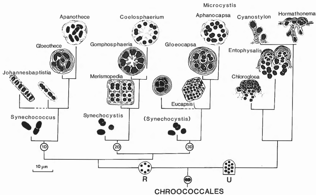
Figure 6. Morphology of modern Chroococcales or coccoid cyanophytes. (From Golubic, 1976.) Growth of coccoids can either be radial (R) or unidirectional (U), and in one-(1D), two-(2D), or three- dimensional (3D) outward growth.
