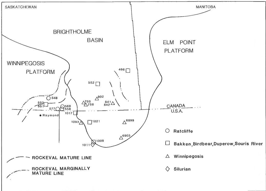
Figure 2. Location and stratigraphic position of oils and stains from reservoirs attributed to Winnipegosis source rocks mentioned in this study. Limits of fondofacies source rock thermal maturity and shelf edge from Figure 1.
