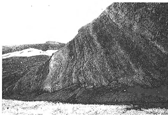
Figure 4. Approximately 30 m thick section of grey and black laminated and massive shale of unit 2.
