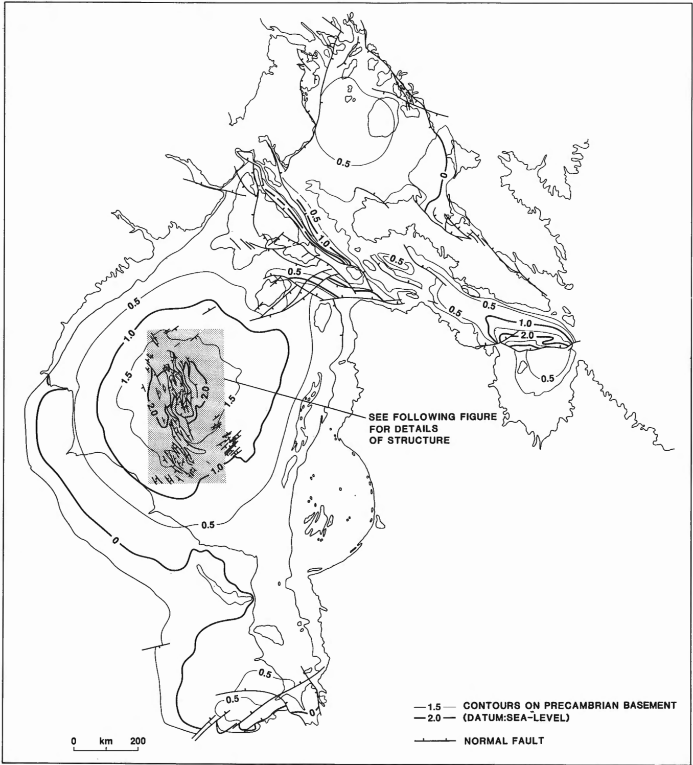
Figure 6. Regional structural framework of Hudson Platform.
