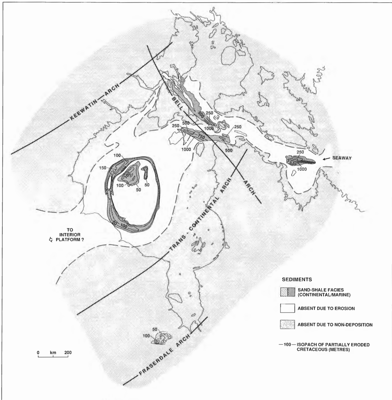
Figure 8. Cretaceous deposition in Hudson Platform.
