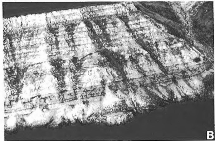
Figure 3. Exposures of the Mount Bayley Formation on west-central Ellesmere Island. A. Greely Fiord section. Upper Antoinette ( AN ), Mount Bayley ( MB ) and lower Tanquary ( TA ) formations are shown. Note dolostone (arrows) and evaporite (white bands) horizons within Antoinette Formation and carbonate horizons (dark bands) within Mount Bayley Formation. Sediments above dashed line in Antoinette Formation comprise porous dolostones. B. Mount Bridgman Section. Note multiple carbonate layers (dark bands) interstratified with evaporites.
