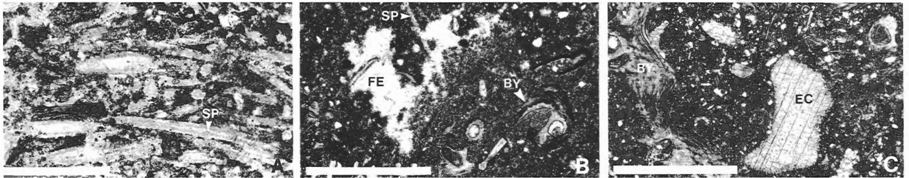
Figure 5. Microfacies of the "unnamed" B formation in BP Graham C-52 well. A. Slightly dolomitic spiculitic (SP) chert; 2569 m (8430 ft.). B. Bryozoan (BY) wackestone with accessory sponge spicules (SP) and cemented fenestrae (FE); 2710 m (8890 ft.). C. Bryozoan (BY), echinoderm (EC) silty packstone; 2710 m (8890 ft.). Scale bars are 400 microns (A) and 1000 microns (B-C).
