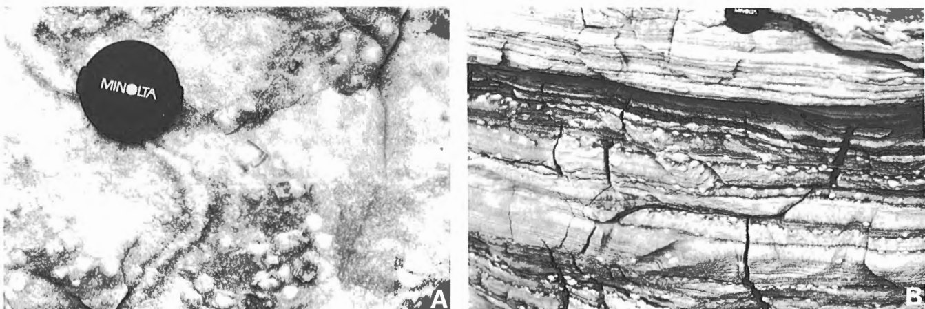
Figure 7. Pseudomorphs of halite hoppers in Mount Bayley Formation, North D'Iberville outcrop. A. Close-up view of bedding plane showing range of hopper preservation. B. Abundant hoppers superimposed on varve-like laminae. Lens cap is 5 cm wide.
