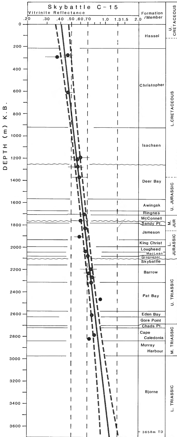
Figure 4. Observed vitrinite reflectance vs. depth, Panarctic et al. Skybattelle Bay C-15 drillhole. The log-linear least squares fit to the data is shown (solid line) and the 95 per cent confidence limits are given by the dashed lines.
