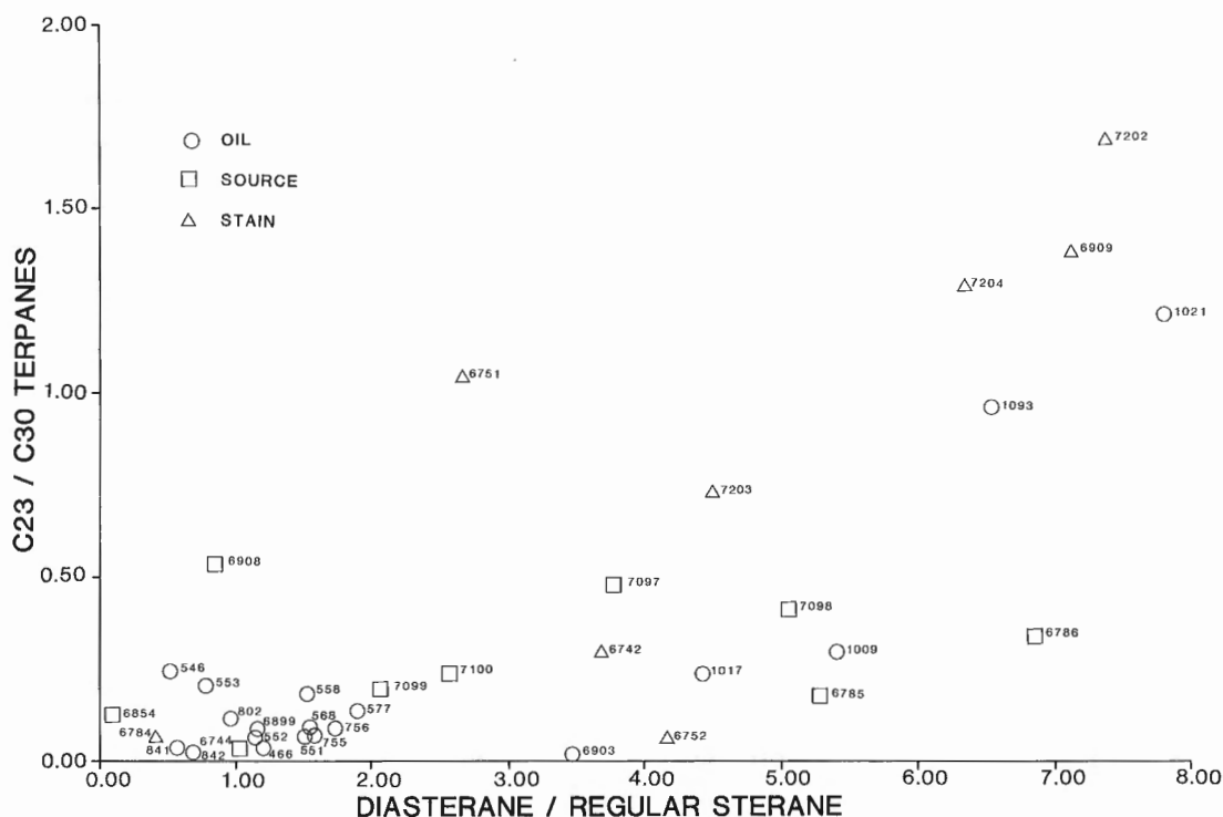
Figure 4. Cross-plot of diasterane/regular sterane ratio and C 23 tricyclic/ C 30 pentacyclic terpane ratio for oils, stains and source rocks from Table 2. Notice both the distribution of samples into fields following critical ratios discussed in the text and the position of samples from the Steelman 2-14 well with respect to the nearby stain 6784 and nearby oils from Bienfait (802) and Oxbow (840 and 841).
