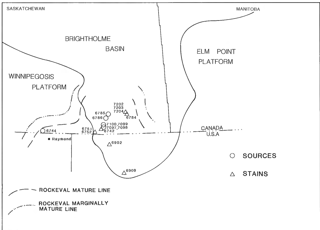
Figure 3. Location of source rocks and stains solvent extracted for this study. Limits of fondofacies source rock thermal maturity and shelf edge from Figure 1.
