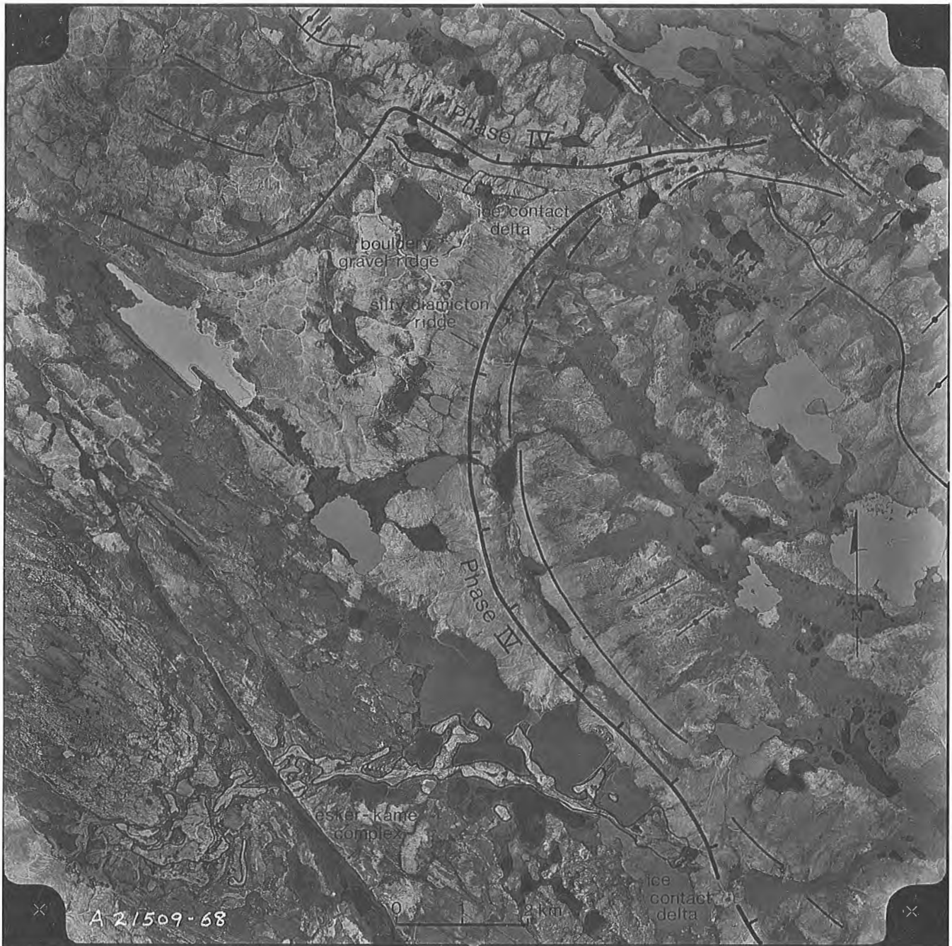
Figure 8. Stapylton Bay (Phase IV) morainic ridges. The east-west ridges are composed of south-dipping beds and lenses of poorly sorted bouldery gravel. The diamicton of the north-south arcuate ridge includes a high percentage of reddish silt similar to the marine sediments to the east. See Figure 4 for legend.
