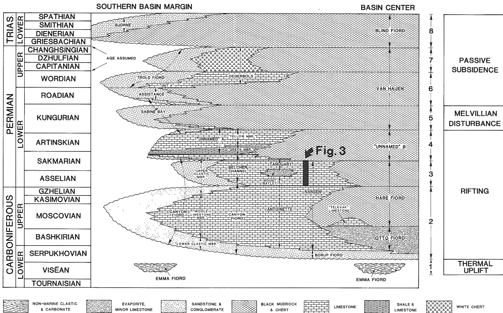
Figure 2. Upper Paleozoic second- and third-order transgressive-regressive sequences in the Sverdrup Basin. (Modified from Beauchamp et al., 1989b). Stratigraphic position of section depicted in Figure 3 is shown.
