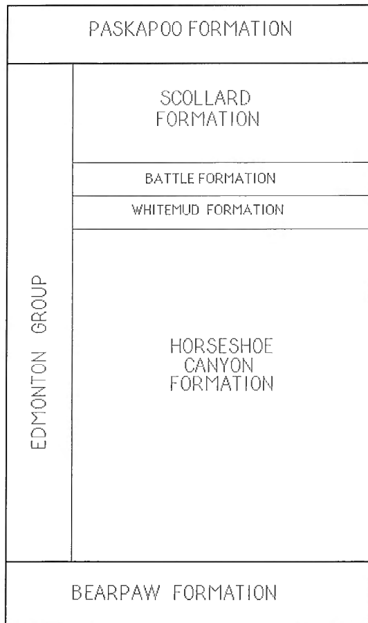
Figure 2. Stratigraphic section of the Upper Cretaceous/Lower Tertiary in the Alberta Plains. (after Gibson, 1977.)
