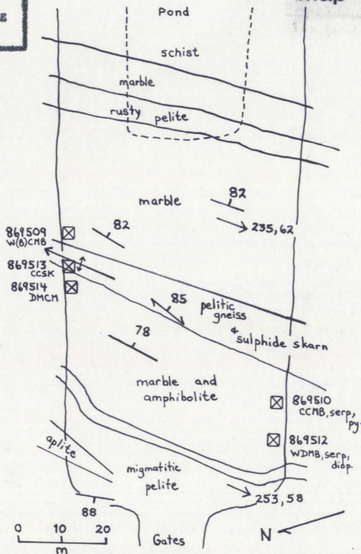
Detailed Plan, McMillan Flowage Tunnel Access Ramp (geology from Barr et. al., 1985, fig. 12)
