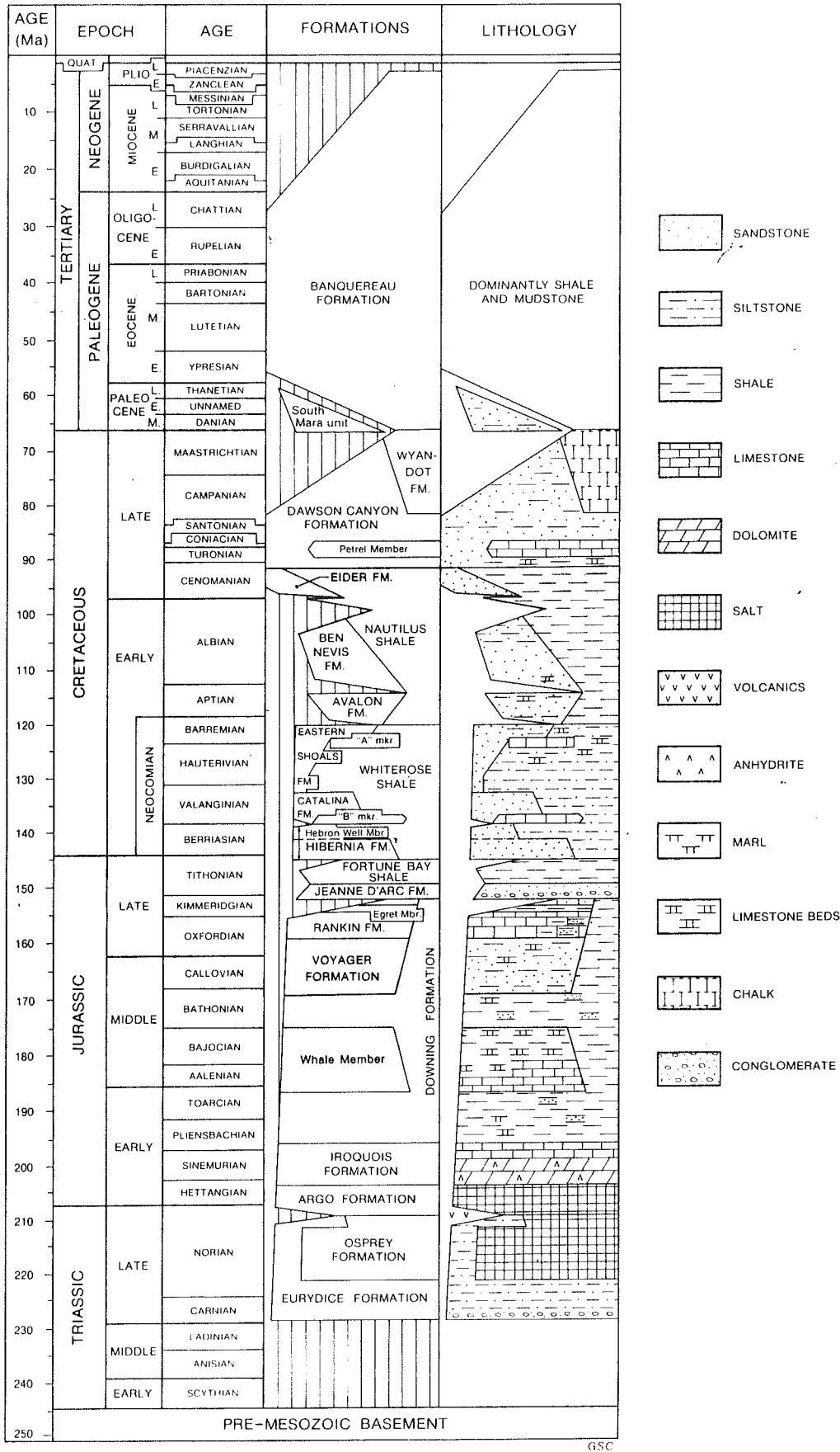
Figure 2. Lithostratigraphic chart for the Jeanne d'Arc Basin (from McAlpine, in press).
