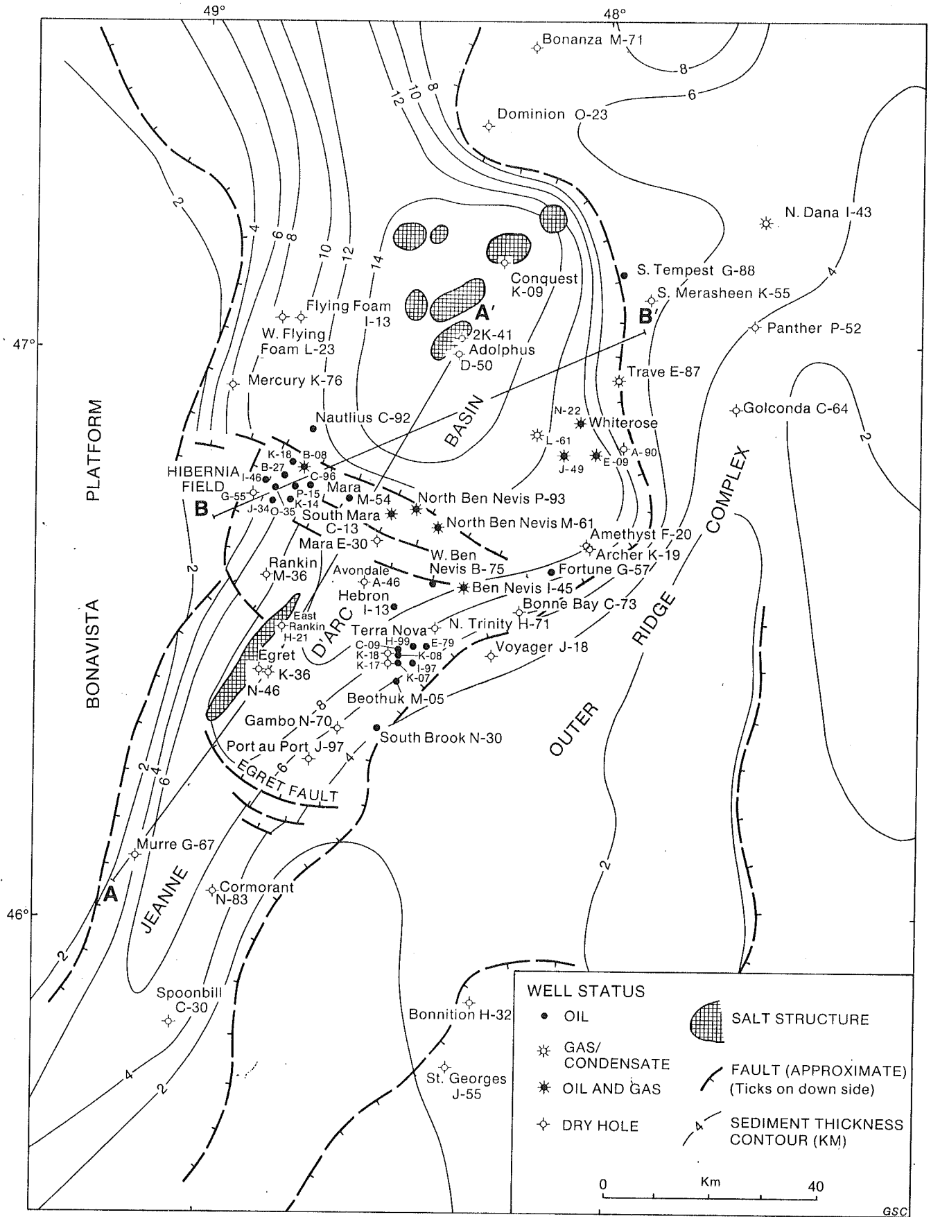
Figure 1. Diagrammatic tectonic element and sediment thickness map of the Jeanne d'Arc Basin showing locations of all wells listed in this report (from McAlpine, in press).
