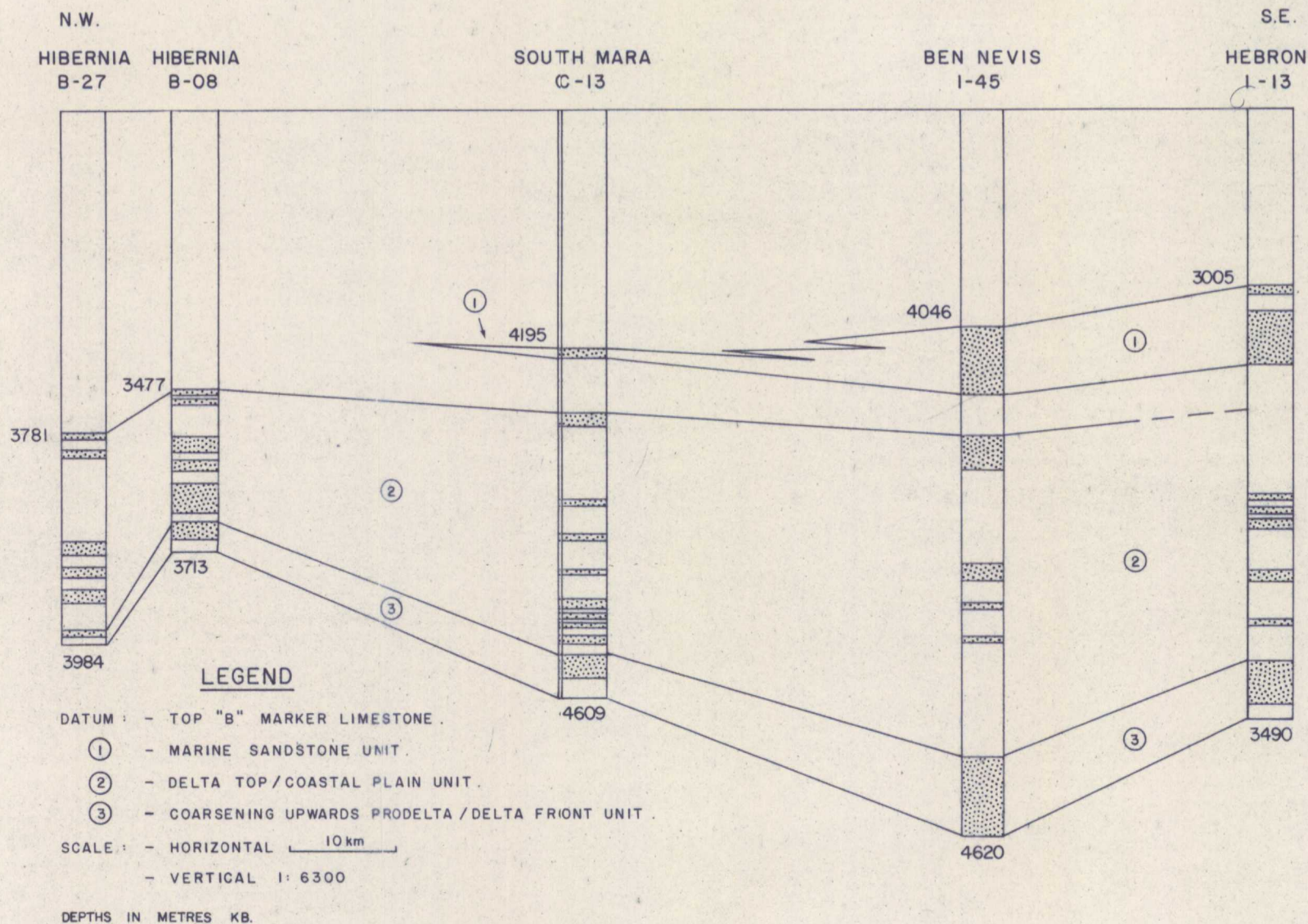
LITHOFACIES CORRELATION DIAGRAM - HIBERNIA MEMBER
