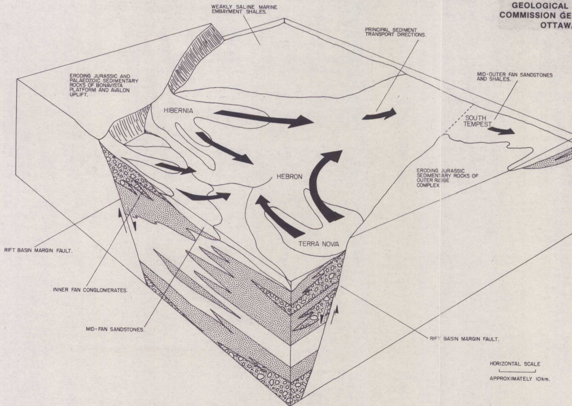
FIGURE: 5 SCHEMATIC BLOCK DIAGRAM TO ILLUSTRATE JEANNE D'ARC MEMBER FACIES RELATIONSHIPS - JEANNE D'ARC BASIN.
