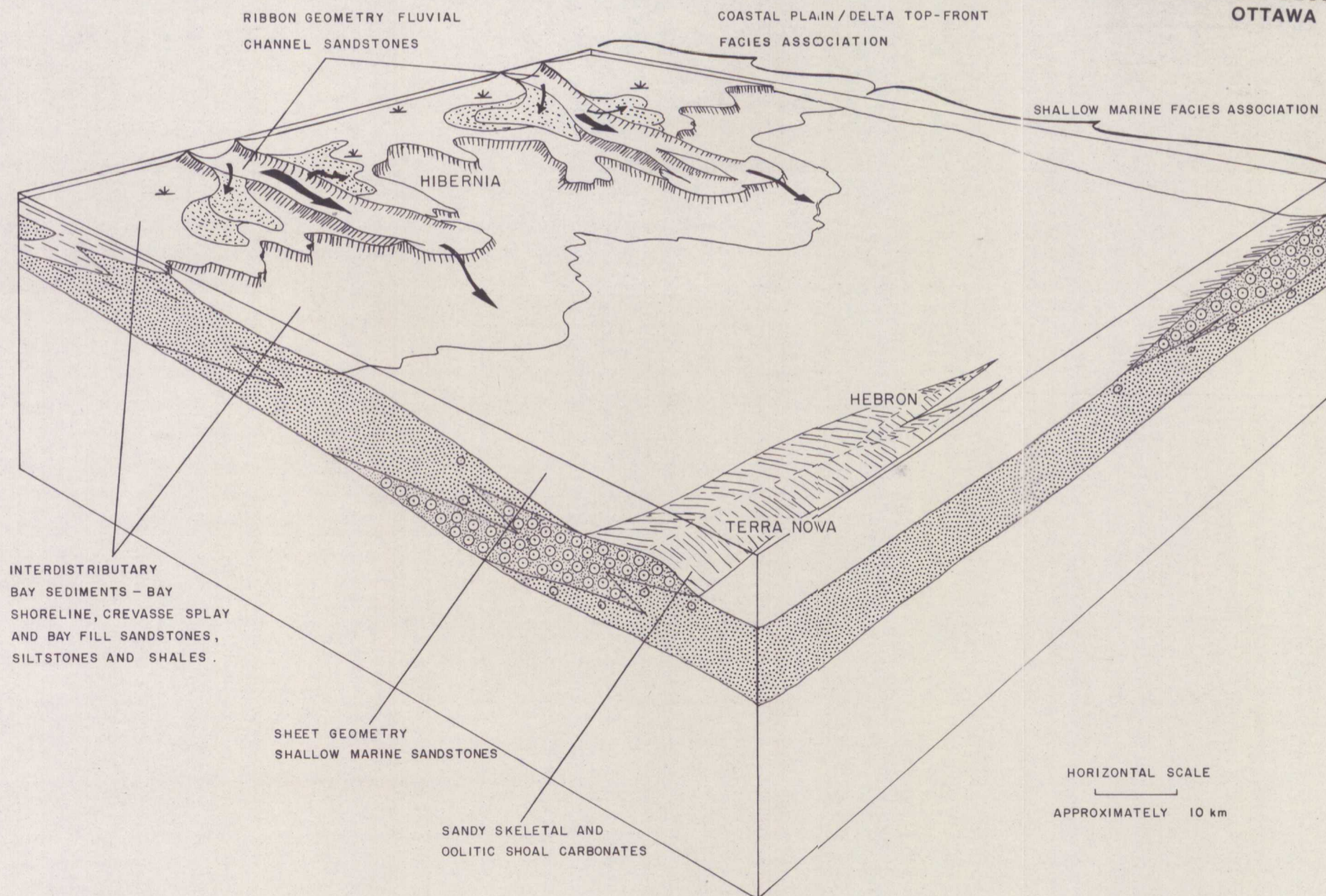
FIGURE: 4 SCHEMATIC BLOCK DIAGRAM TO ILLUSTRATE "C" MEMBER IFACIES RELATIONSHIPS IN THE JEANNE D'ARC BASIN
