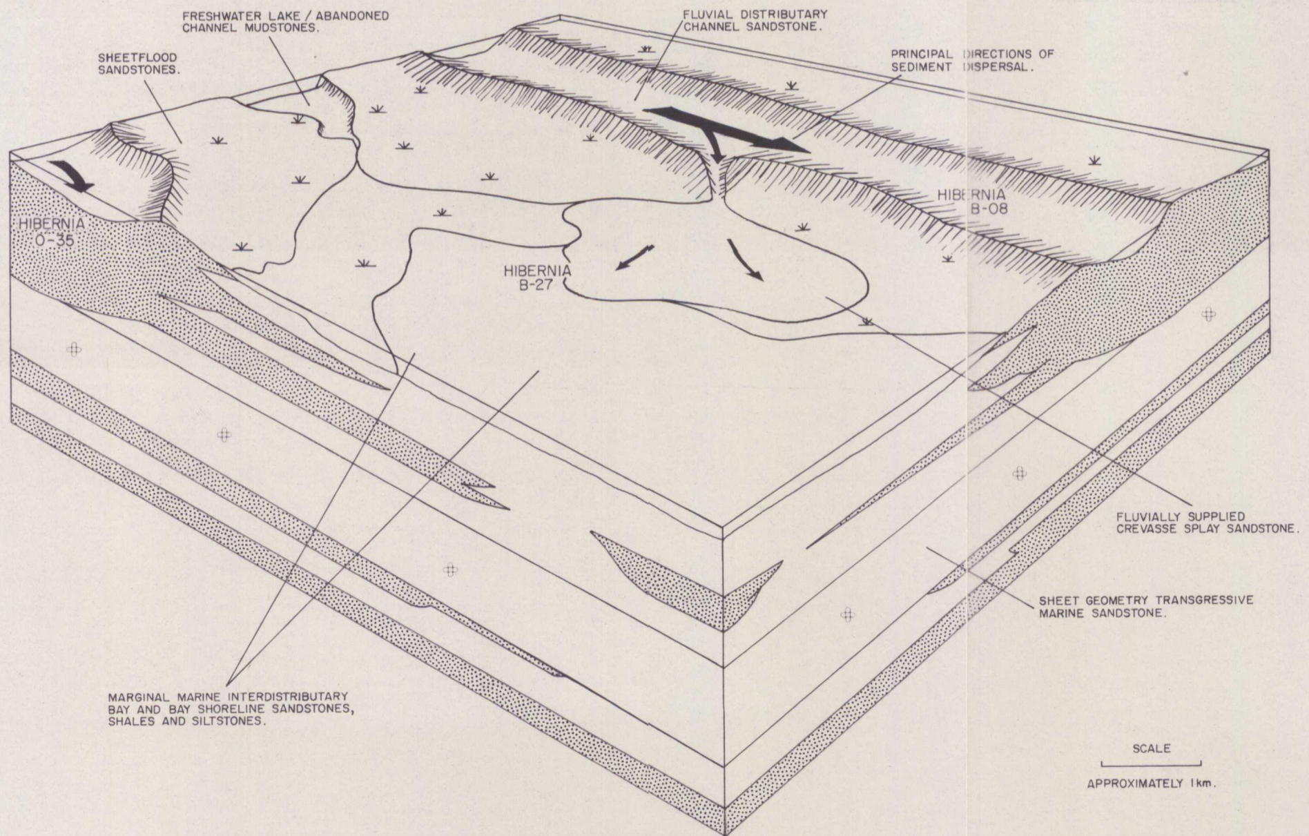
FIGURE: 3 SCHEMATIC BLOCK DIAGRAM ILLUSTRATING THE FACIES RELATIONSHIPS OF HIBERNIA MEMBER SEDIMENTS IN THE HIBERNIA FIELD AREA.
