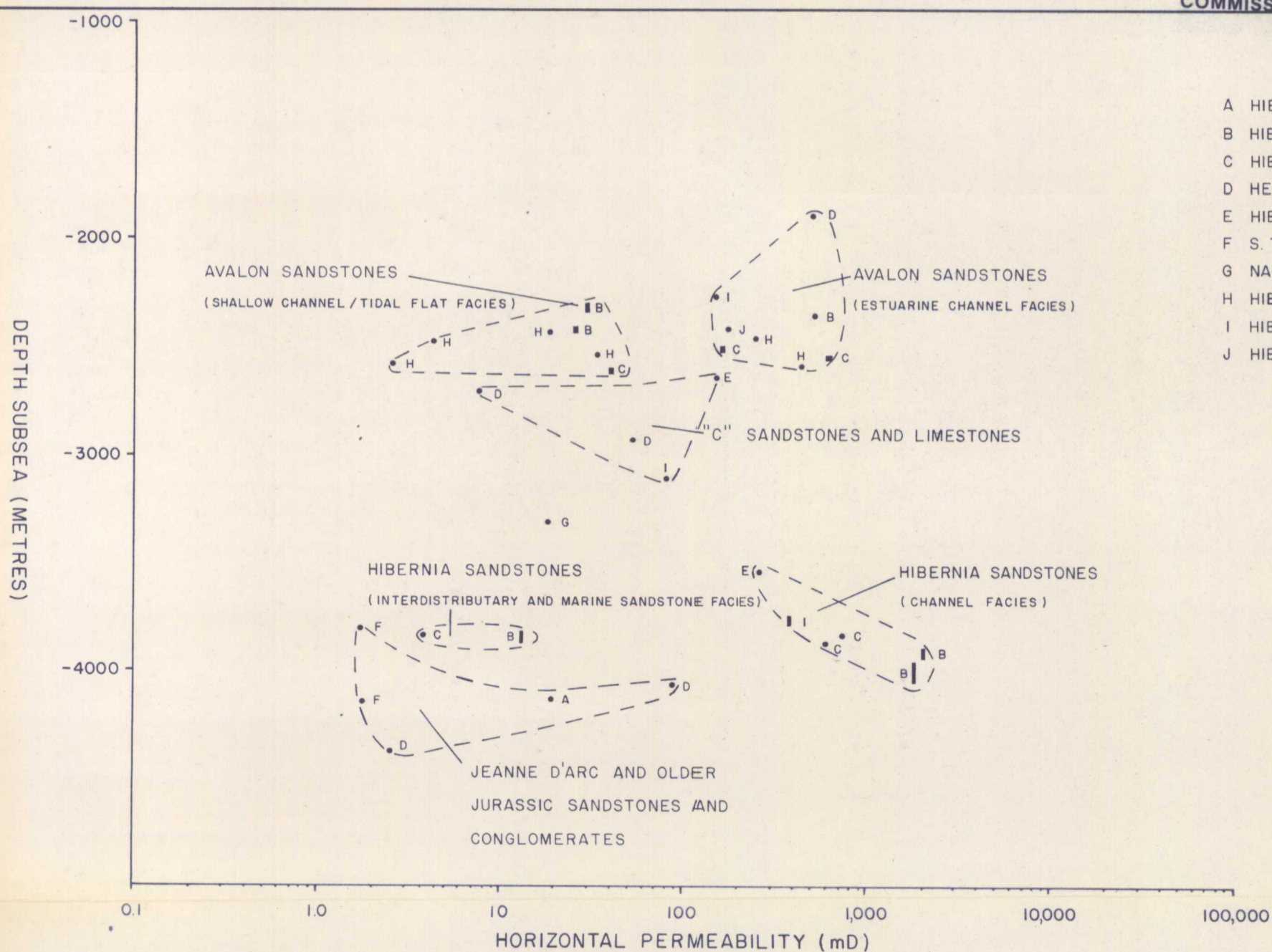
FIGURE 16 DEPTH vs MEAN HORIZONTAL PERMEABILITY (AS RECORDED ON DATA SUMMARY CHARTS).
