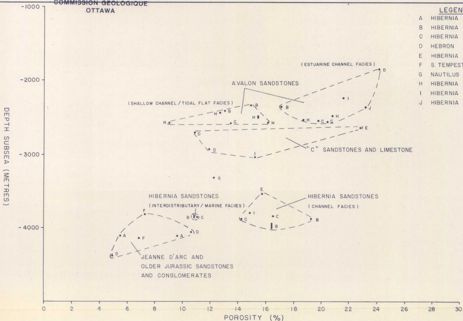
FIGURE 15 DEPTH vs MEAN POROSITY (AS RECORDED ON DATA SUMMARY CHARTS).
