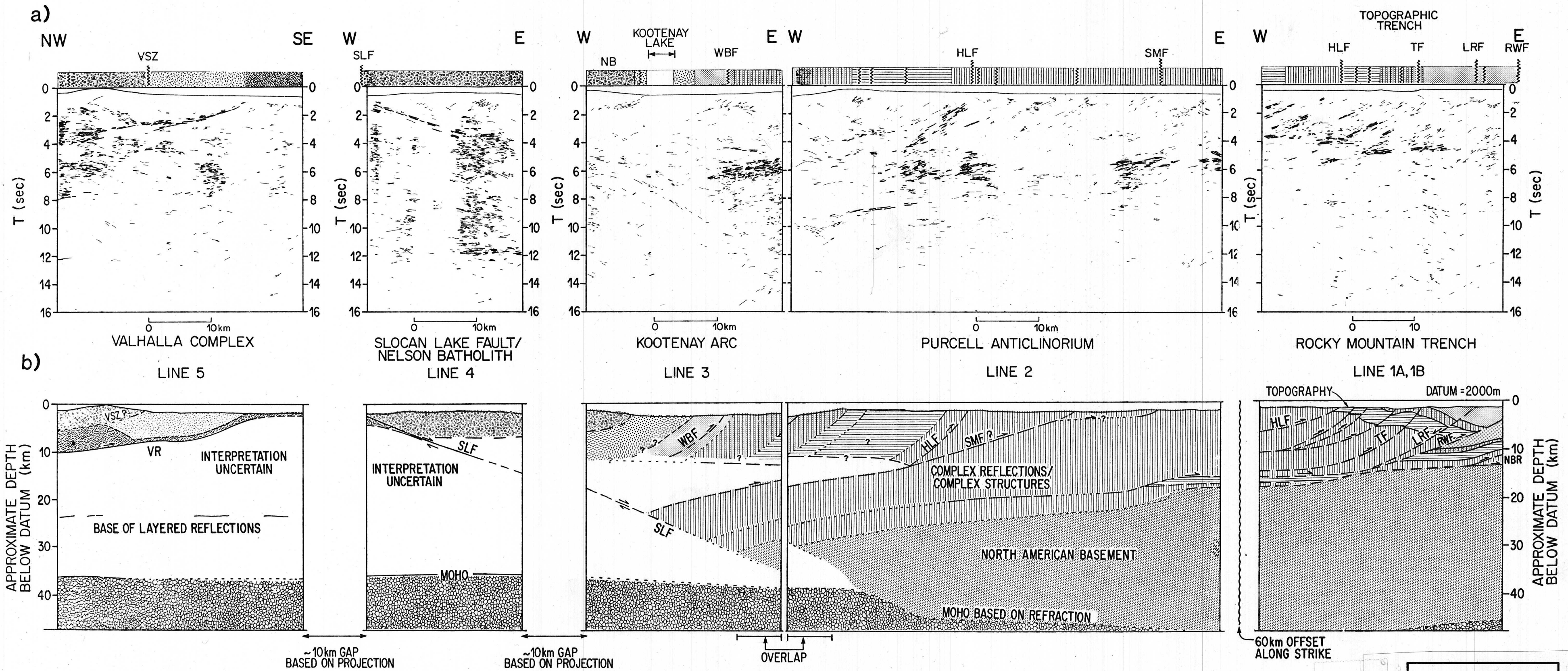
Plate 1. Line drawing summary of the reflection geometry observed on the Lithoprobe data (unmigrated). (a) Line drawings of the reflection events with the general geological boundaries shown at the top. (b) Generalized interpretation based upon correlations with surface features, industry seismic data, and other geophysical information. The patterns used are consistent with Figure 1. Solid lines are certain, dashed lines are probable, and dotted lines are only weakly controlled. Abbreviations used, in addition to those of Figure 1, are NBR = near-basement reflections, LRF = Lussier River fault, TF = Torrent fault, VR = Valhalla reflection.
