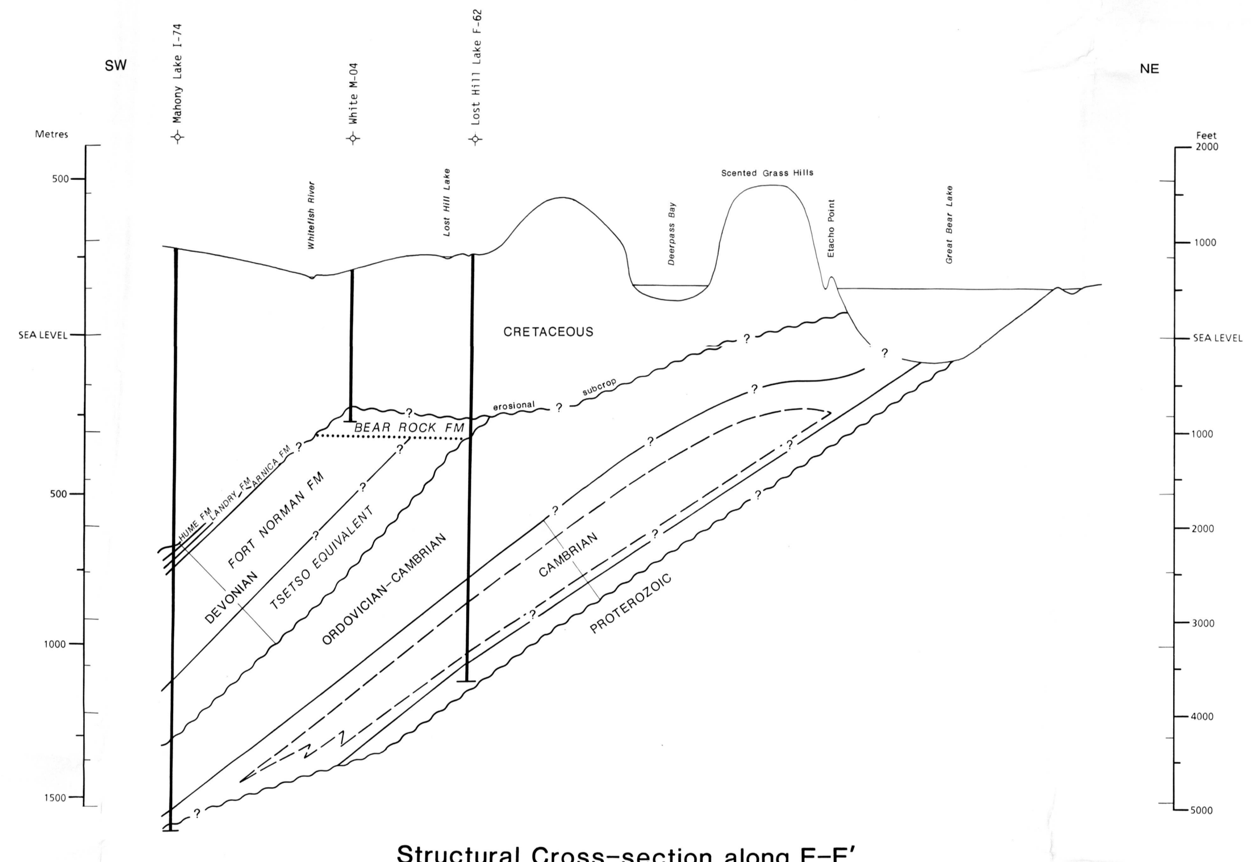
Structural Cross-section along E-E'
