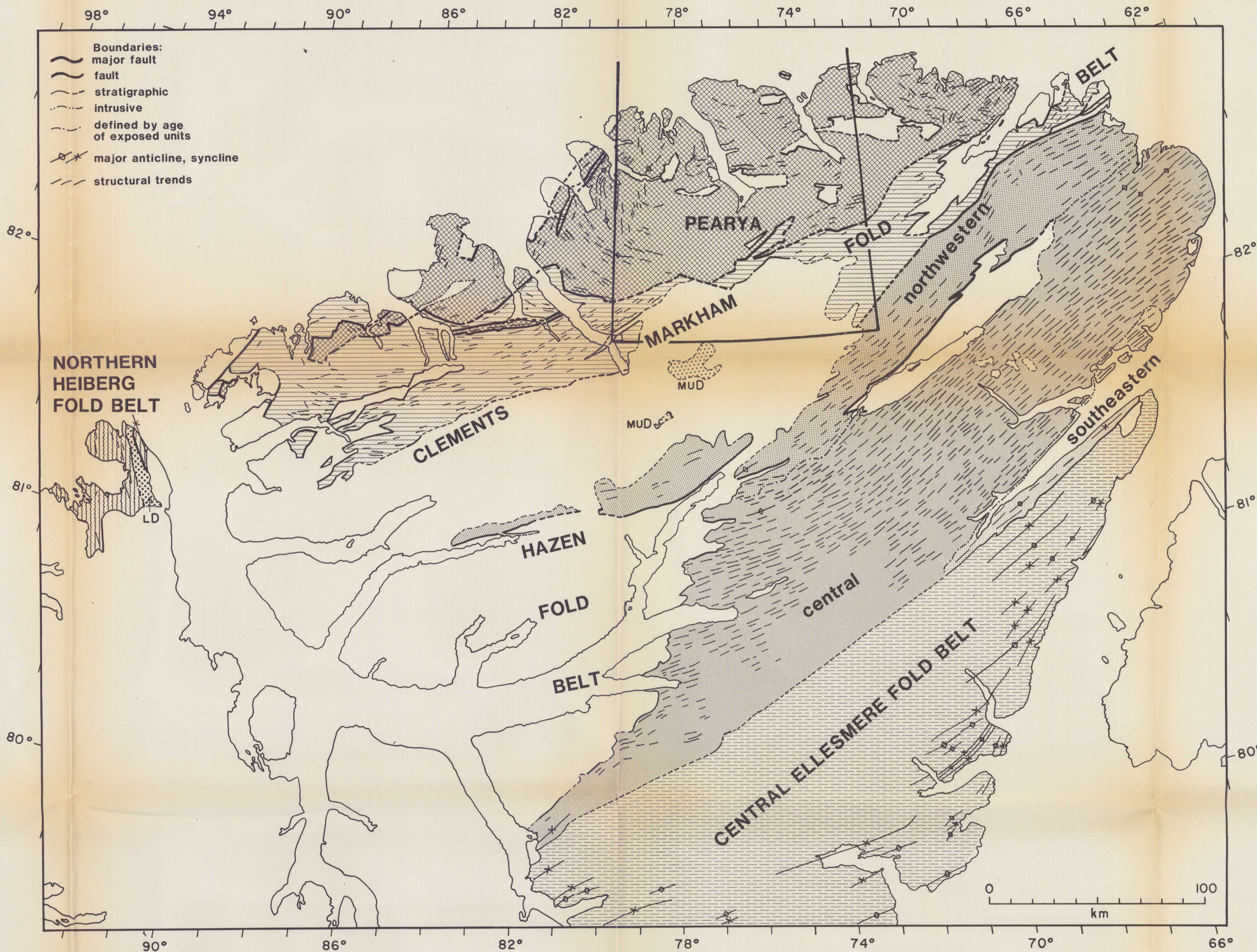
Figure 1. Stratigraphic-structural subdivisions, northern Ellesmere and Axel Heiberg islands and location of M'Clintock Inlet map-area. LD: Lower Devonian and (?) Upper Silurian; MUD: Middle-Upper Devonian. Blank areas are covered by upper Paleozoic and younger strata.
