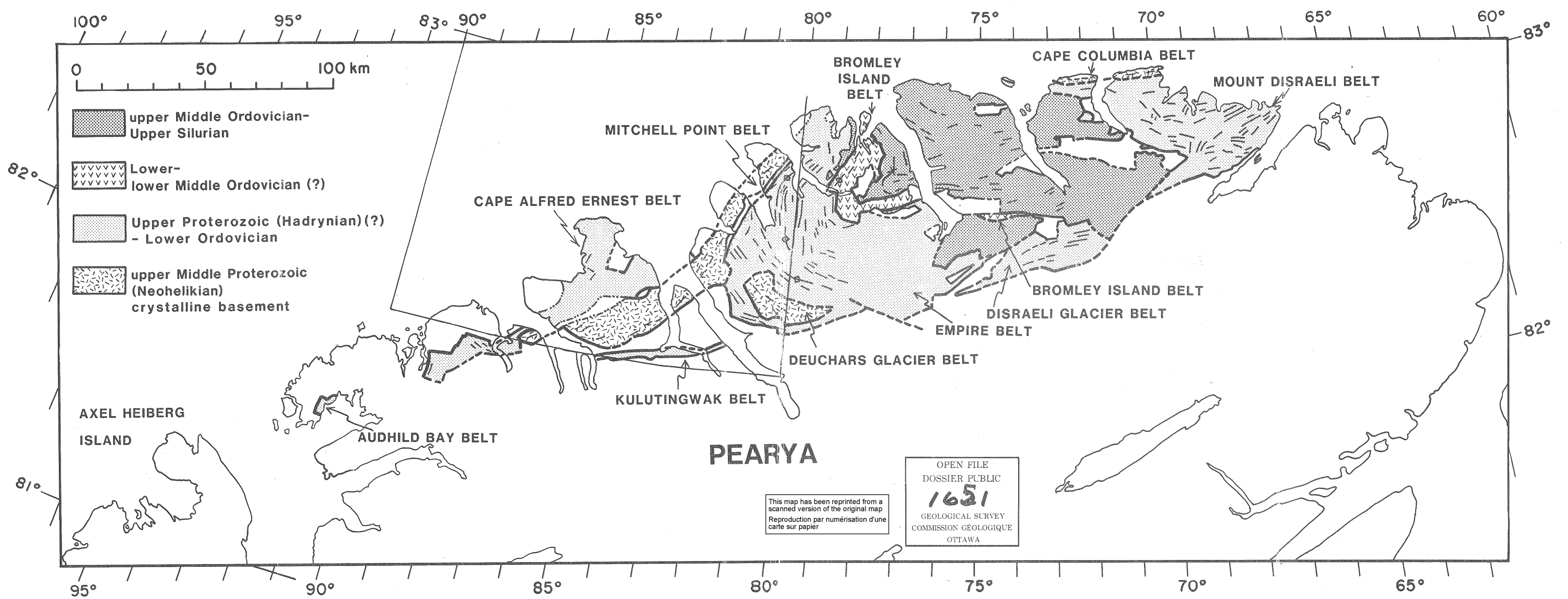
Figure 2. Components of Peary Terrane and index.
