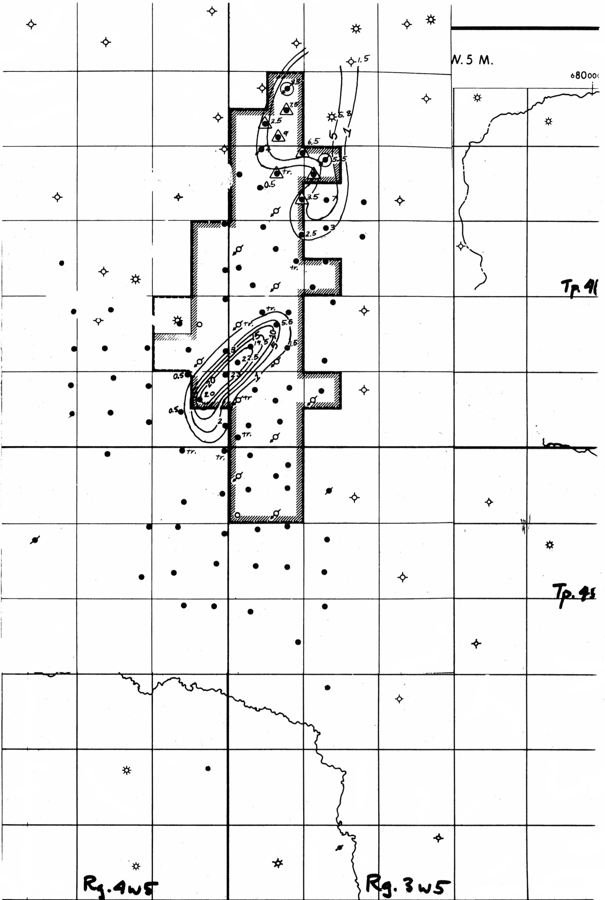
CRYSTAL VIKING FIELD (Scale 1:50,000) ISOPACH MAP OF CONGLOMERATE LITHOFACIES The 1, 5, 10, 15, and 20-metre isopach lines are shown.
