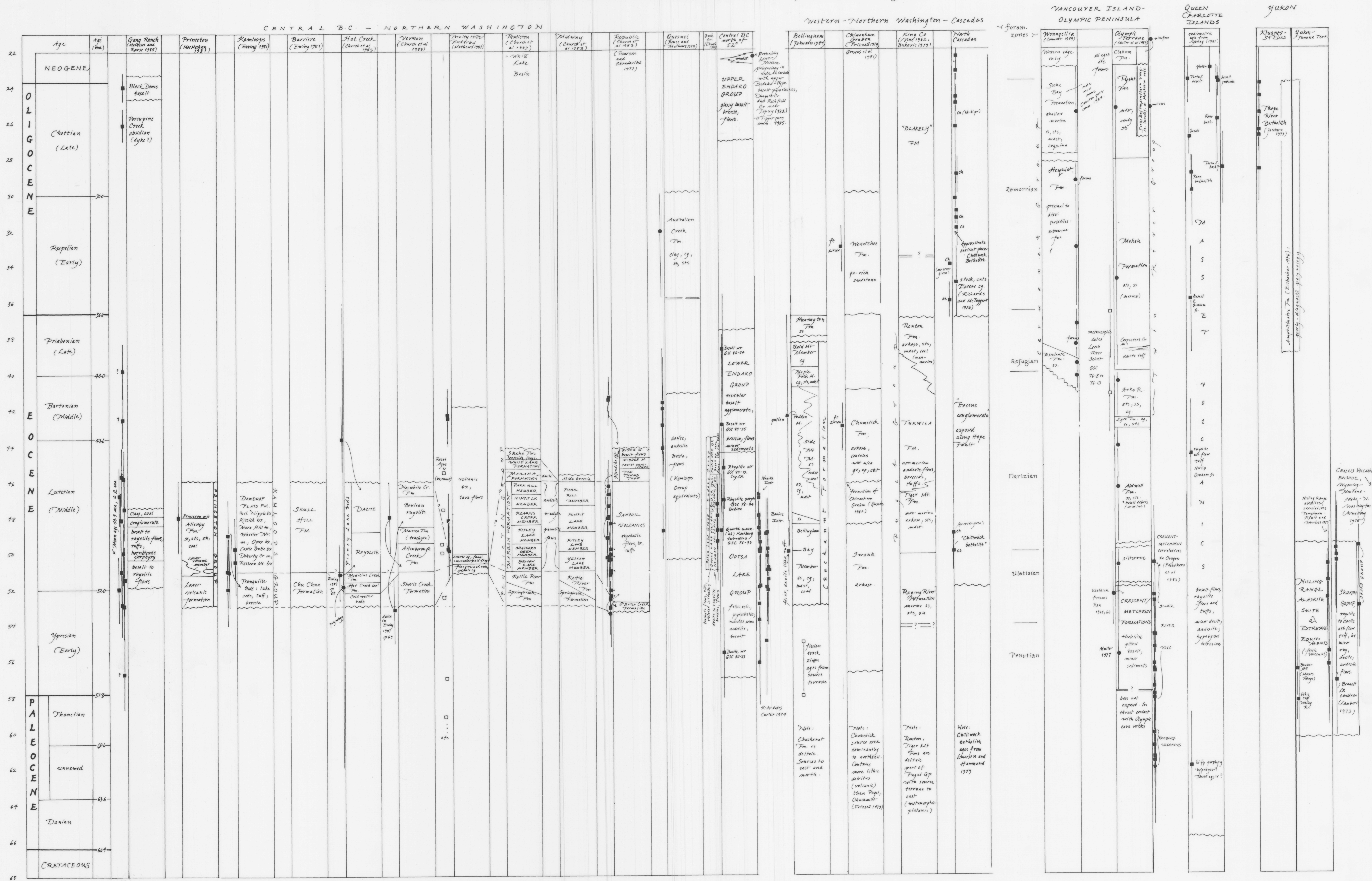
FIGURE 4 PALEOGENE STRATIGRAPHY, WESTERN CANADIAN CORDILLERA (includes parts of northern Washington)
