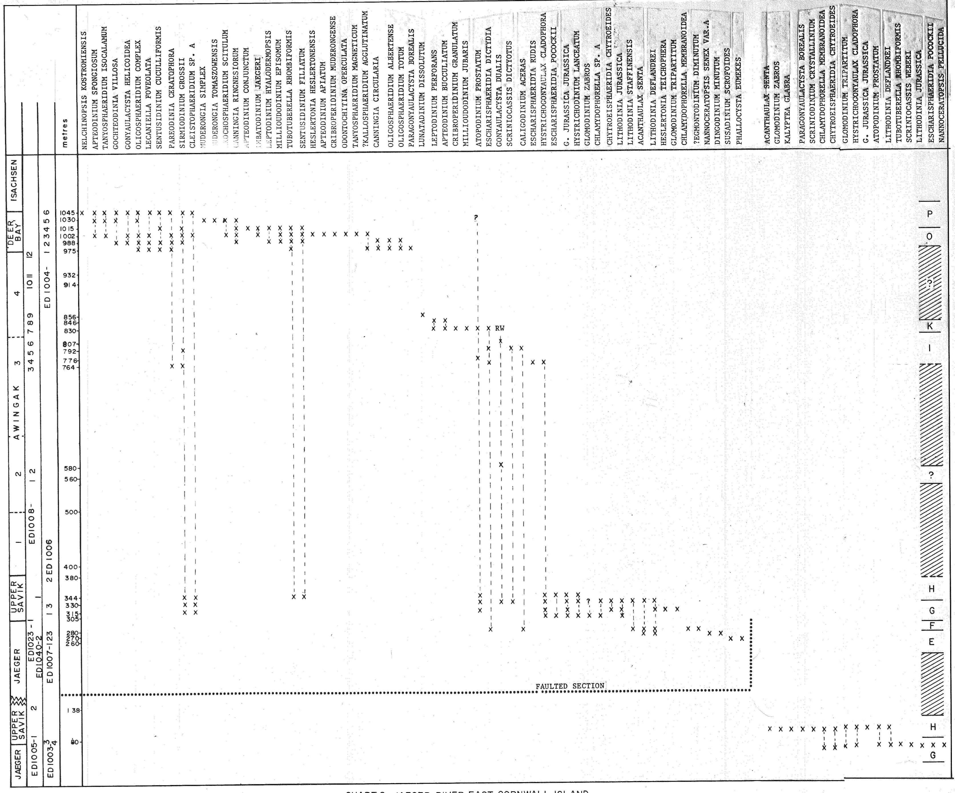
CHART 8. JAEGER RIVER EAST CORNWALL ISLAND
