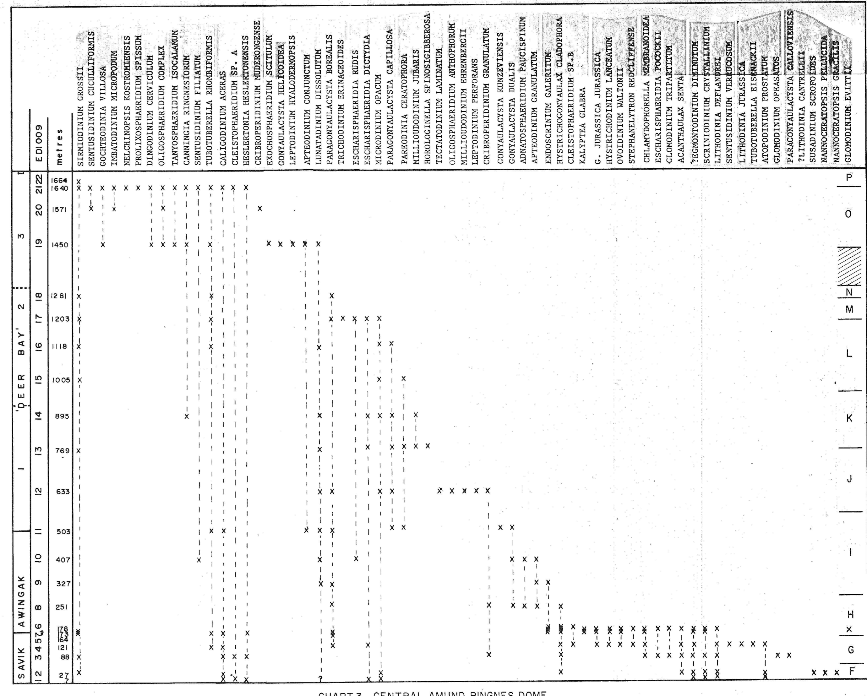
CHART 3. CENTRAL AMUND RINGNES DOME
