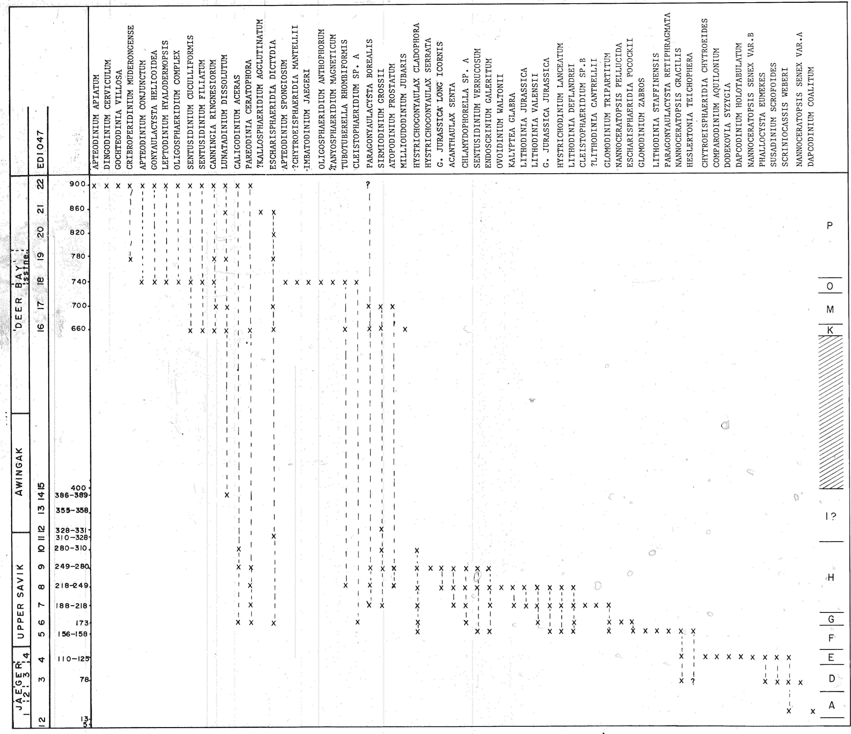
CHART 6. NORTHWEST CORNWALL ISLAND
