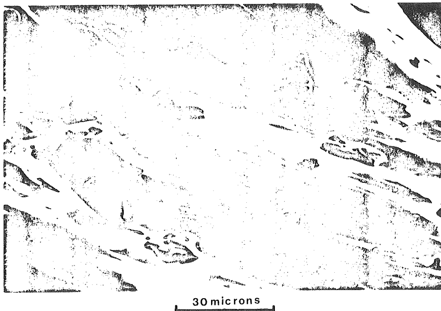
Parallel striae and silica plastering.
