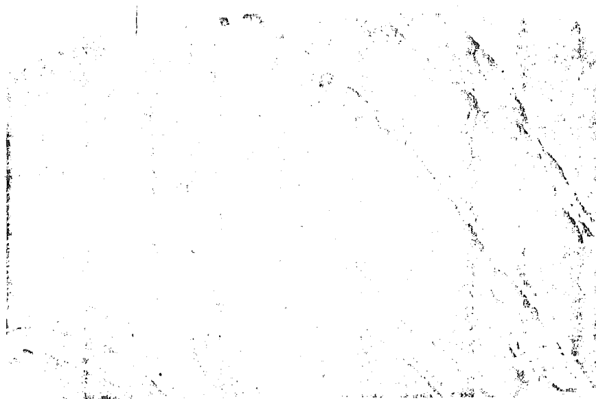
Silica plastering on cleavage faces.
