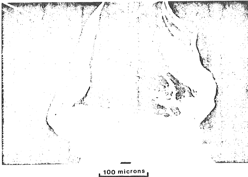
Angular quartz grain showing high relief and conchoidal fracturing.
