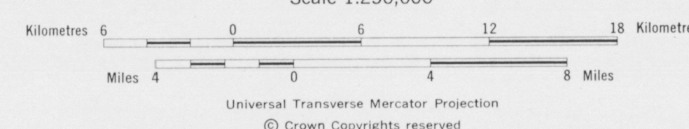
NATIONAL GEOCHEMICAL RECONNAISSANCE MAP 15-1976 MOLYBDENUM IN STREAM SEDIMENTS URANIUM RECONNAISSANCE PROGRAM Scale 1:250,000
