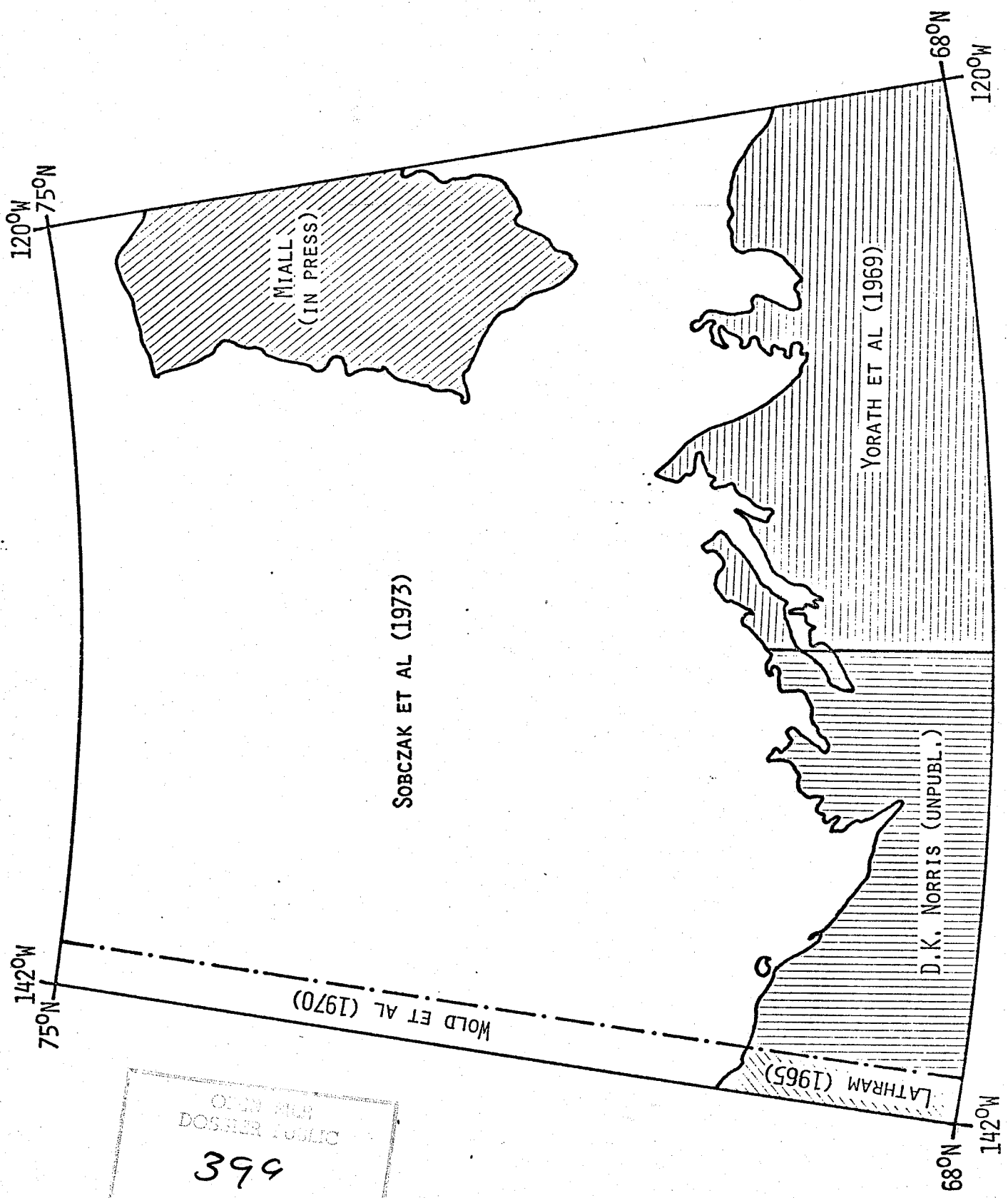
SOURCES OF INFORMATION FOR GEOLOGICAL MAP OF SOUTHERN RIM OF CANADA BASIN
