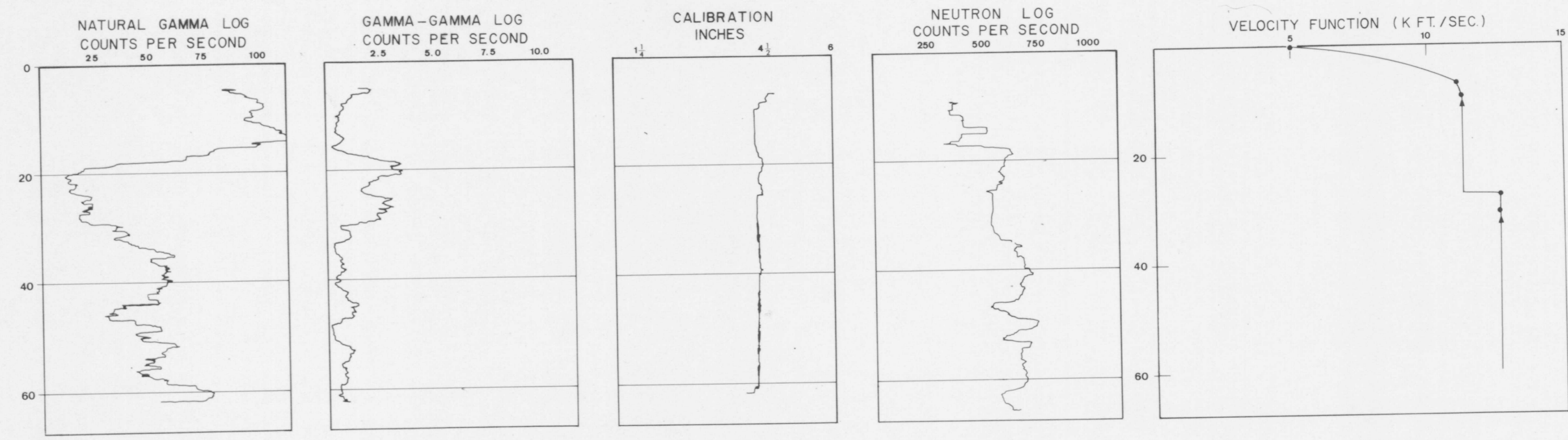
Figure 4: Geology, Borehole Geophysics and Seismic Soundings at Location 3.
