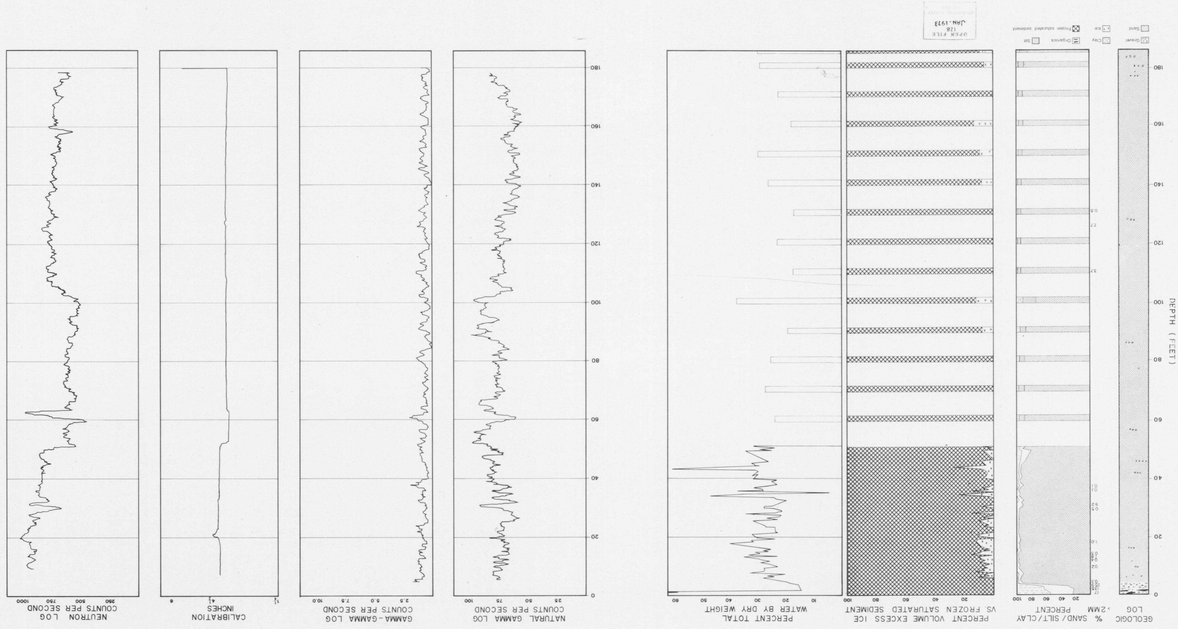
Figure 3a: Geology and Borehole Geophysics at Location 2
