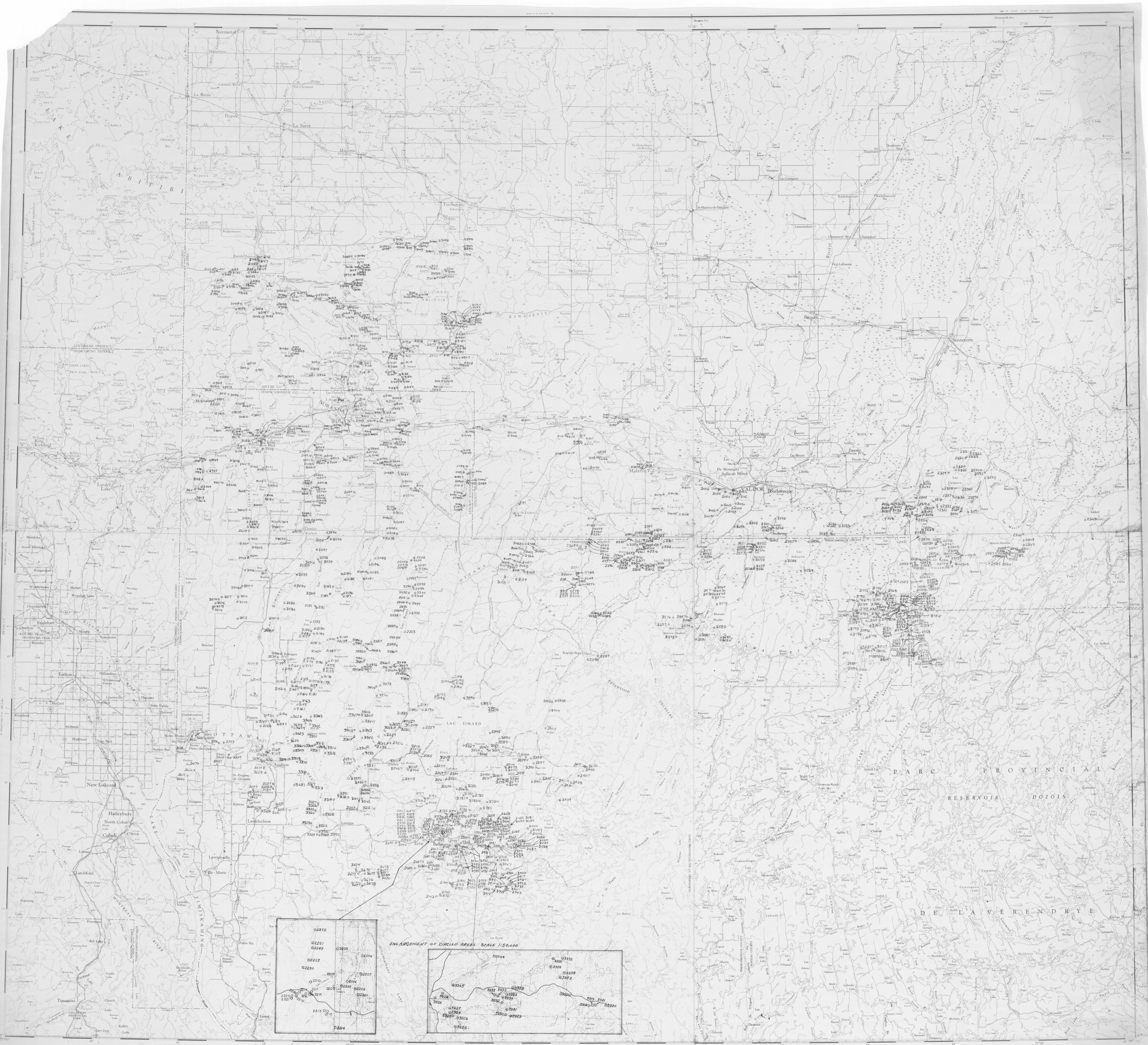
LOCATION OF LAKE BOTTOM SEDIMENT SAMPLES FROM NORANDA - VAL D'OR AND BELLETERRE AREAS - QUEBEC
